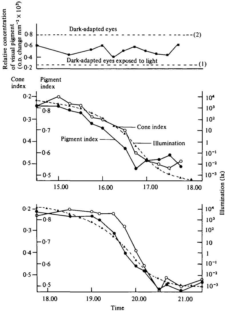
Fig. 4. Average concentration of extractable visual pigment at equal intensities during two dusk periods. The concentration of visual pigment represents the average concentration in three eyes at various intensities during two dusk periods. The position of the retinal epithelial pigment and cones on the two occasions are plotted below these. The retinal pigment index is shown by the filled circles (●), the cone index by the open circles (○), and the intensity of the light by the broken line and filled triangles (▲---▲). (1) and (2) are the levels of visual pigment found in dark-adapted eyes followed by a 10 min bleach and fully dark-adapted eyes respectively, as described in the text.
