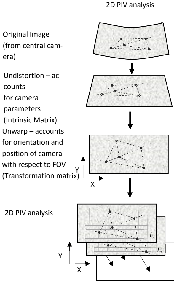
Figure 4. PIV analysis procedure to determine horizontal displacements (after Le et al. 2016)
