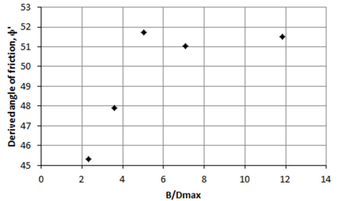
Figure 5. Angle of friction of platform material obtained from test results
