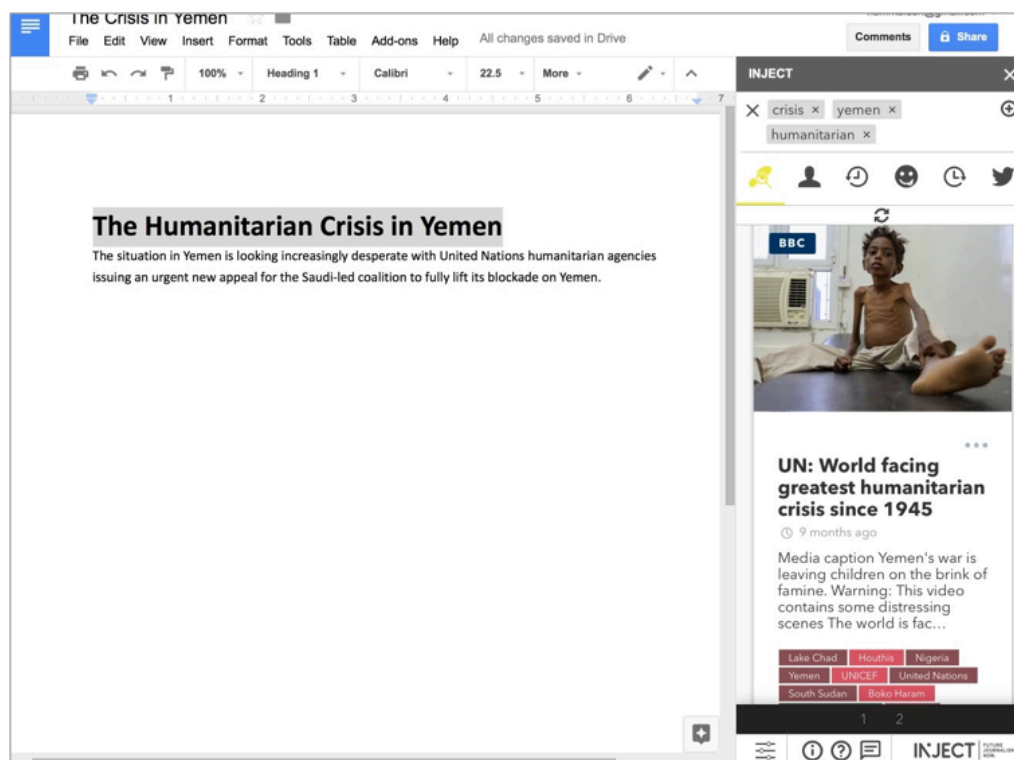
Figure 3. The INJECT sidebar, showing news information retrieved using INJECT’s backing and evidence creative strategy, presented in interactive cards
