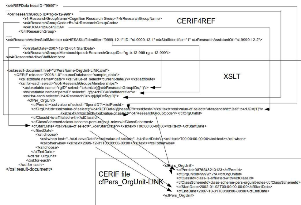
Figure 8. Deriving cfPERS-OrgUnit-LINK from CERIF4REF using XSLT.
