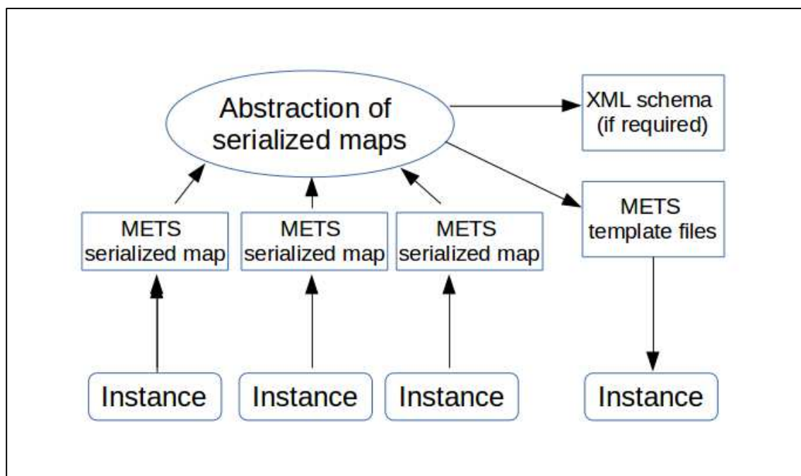
Figure 2 Model for proposed synthesis of three intermediary schema methods
