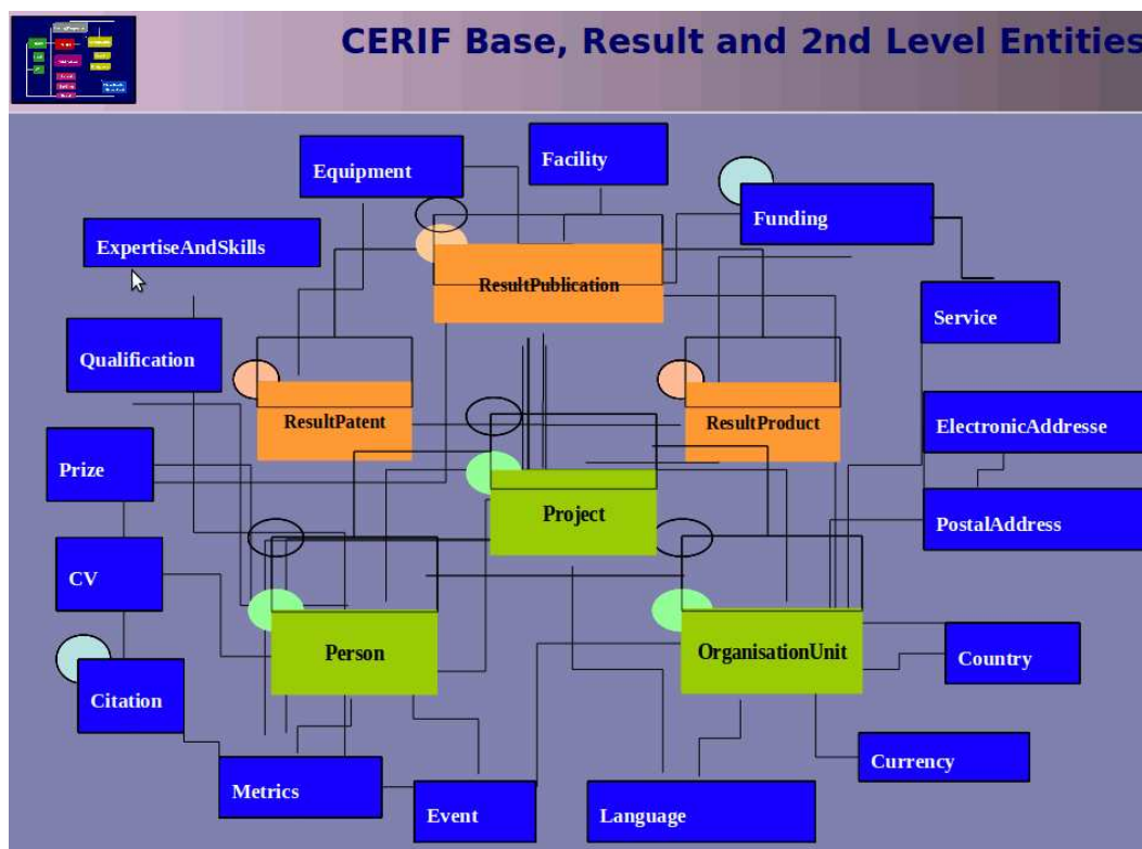
Figure 3. CERIF Base, Result and 2nd Level entities.
