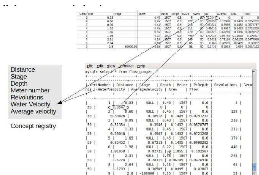
Figure 2 Mapping data entries via a concept repository
