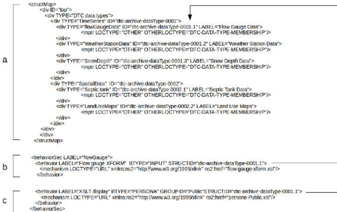
Figure 1 Incorporating XFORM and XSLT associations into template METS file
