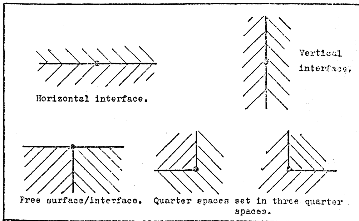
Interface nodes for which second order formulations are given.
