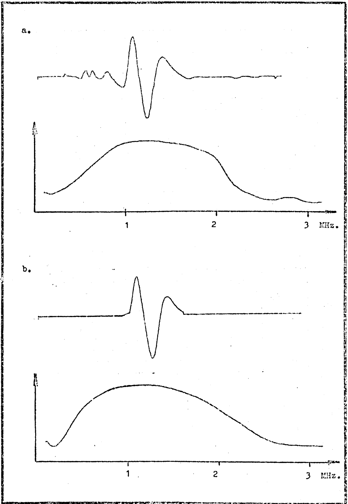
Time domain signals and spectra for pulses on an aluminium quarter space; a. when using a wide gate (about 5 \mu sec.) b. when using a narrow gate (about 1.2 \mu sec.)
