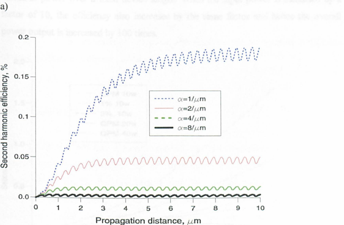
Fig 6.18 Numerical simulation of various assumed loss values in a) non-QPM GaAs device and b) QPM GaAs device.
