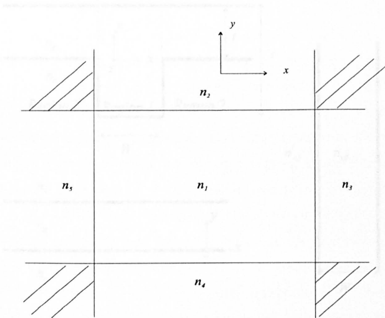
Fig. 1.3 A model for the effective index method
