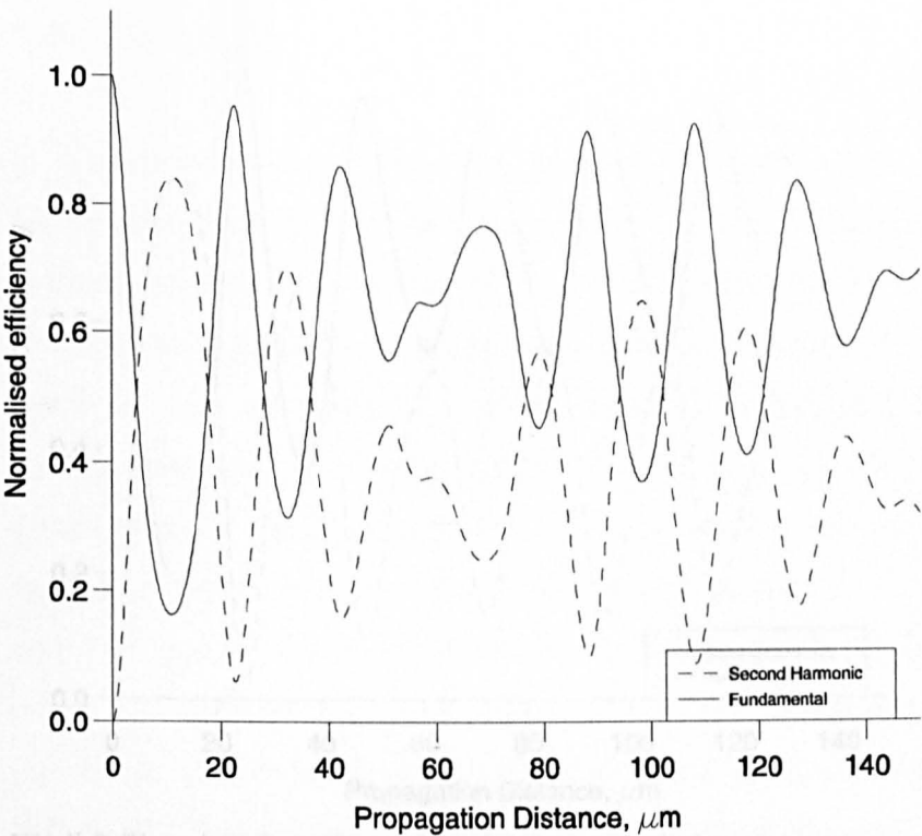
Fig 7.9 Showing the effect of higher intensity in input power
