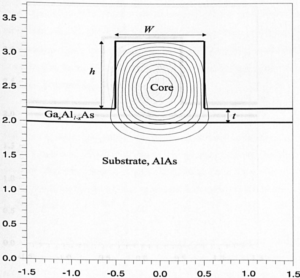
Fig 6.4 Diagrammatic representation of a waveguide structure with confinement of the fundamental wave.
