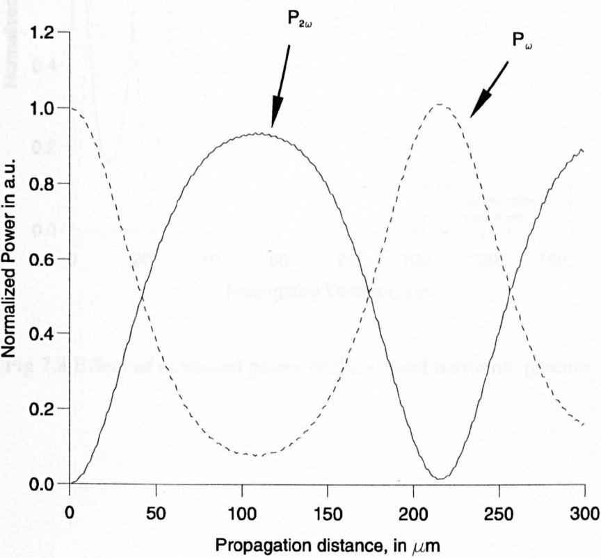
Fig 7.7 Showing the process of quasi phase matching with depletion in the fundamental.
