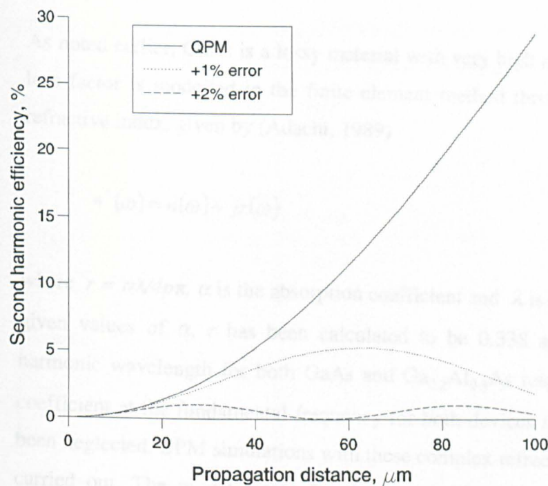
Fig 6.12 Effect of fabrication error on second harmonic output power, a comparison of idealised QPM with assumed error.
