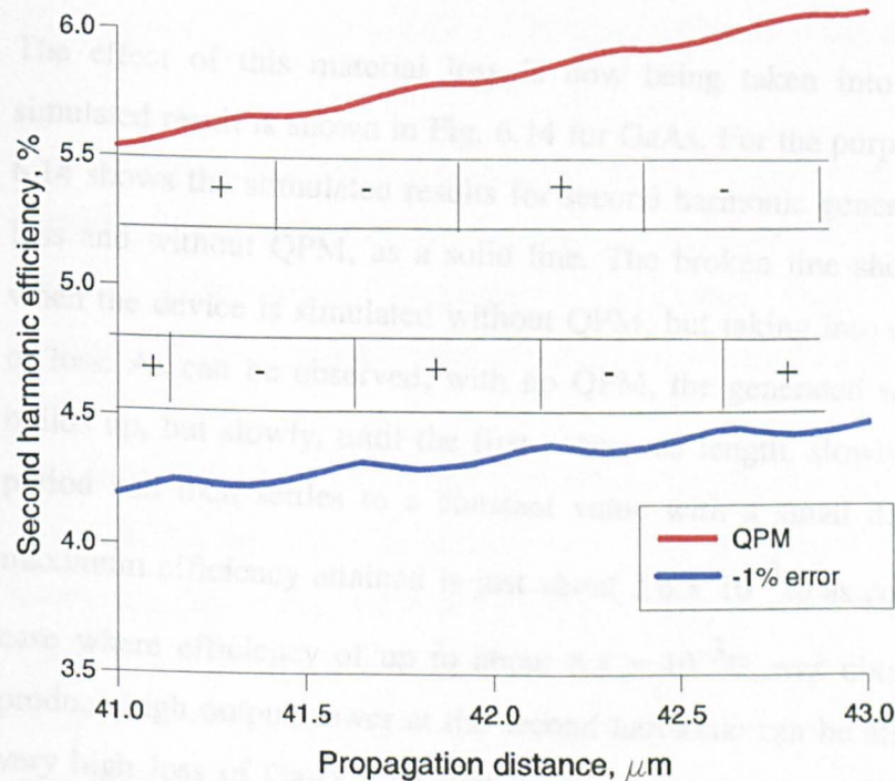
Fig 6.13 A magnified picture of domain mismatch for a -1% error.
