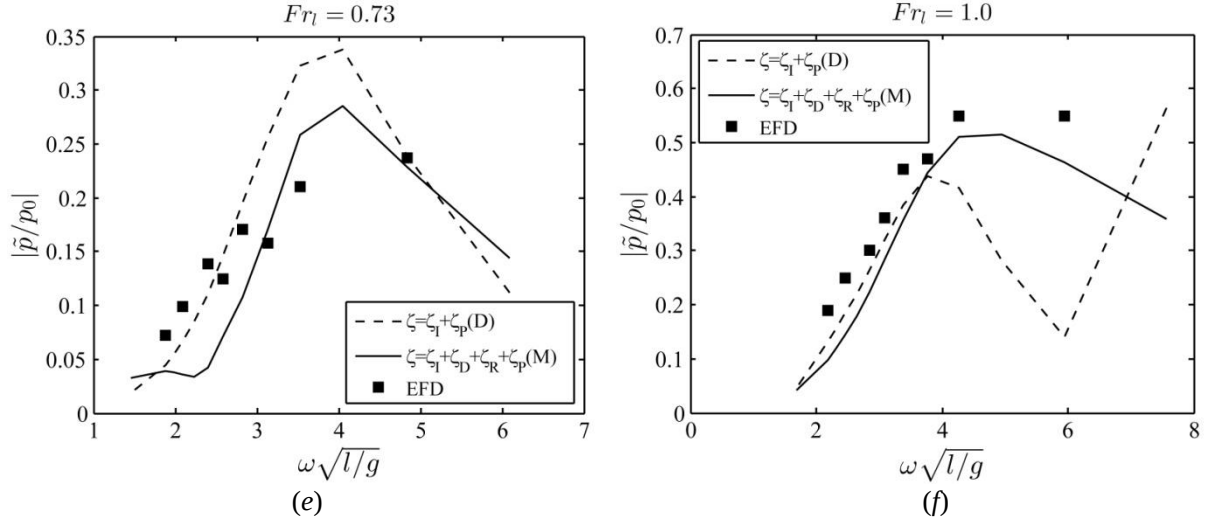
Figure 3. A comparison of numerical results with experimental data marked as ‘EFD’ on seakeeping performance of the PACSCAT under Froude number Fr_l = 0.73 and 1.0 . ‘ \zeta = \zeta_I + \zeta_p(D) ’ represents the numerical results obtained from the model that considers the incident wave and the radiation wave due to fluctuating air pressure on the interface by solving the Dirichlet BVP, while the sidehull induced waves are not taken into account. ‘ \zeta = \zeta_I + \zeta_D + \zeta_R + \zeta_p(M) ’ are obtained from the model that considers all possible waves on the interface, including the incident wave, diffraction and radiation wave of sidehulls, the radiation wave due to fluctuating air pressure by solving the mixed BVP. ‘CFD’ are the CFD results from Yang et al. (2015). (a~b) Heave RAO; (c~d) Pitch RAO; (e~f) Fluctuating air pressure RAO.
