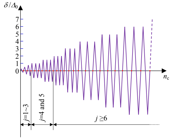
Fig. 5. Loading protocol.
