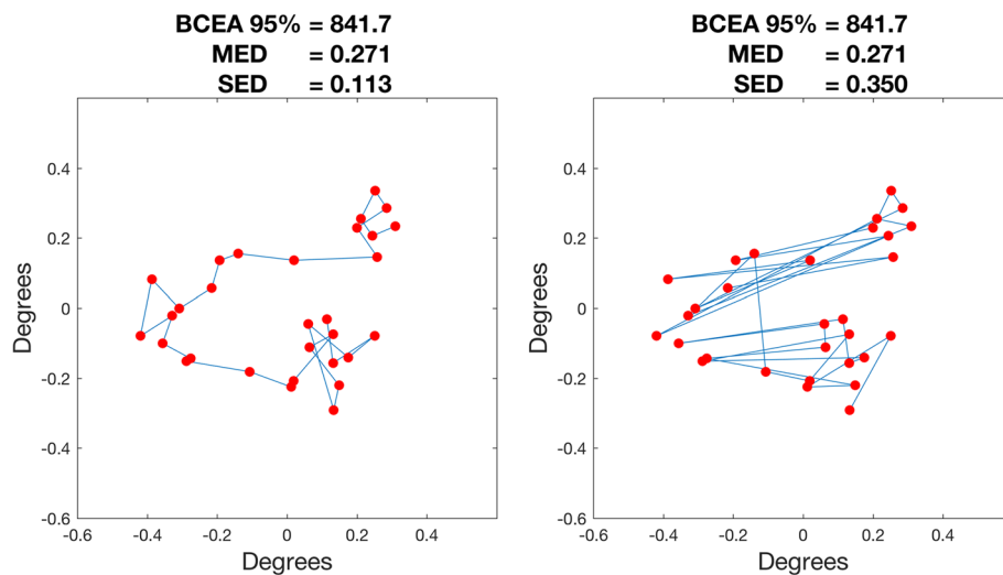
Fig. 1 Schematic representation of the differences between the two proposed MED and SED indices. The left and right tracks represent two fictional fixation patterns ( n = 30 points). The red dots represent the individual displacements of fixation and the blue lines join subsequent locations in the sequence. Both fixation patterns have the same point coordinates (the red dots) but the sequence is different. In the pattern on the left each displacement tends to be very close to the previous location in the sequence. In the pattern on the right, fixation shifts randomly from one point to another. As a result, indices that only account for fixation point locations (the BCEA and the MED) do not change. On the contrary, the SED index, calculated as the average of distances between successive points in the sequence, is greatly increased in the pattern on the right, capturing the continuous movement from one position to the other
