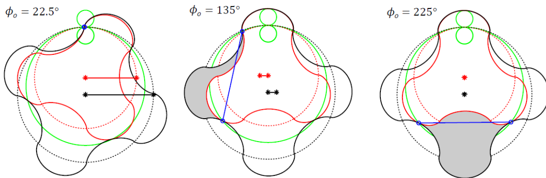
Figure 3: Cross-sectional area of working chamber at different angular positions of outer rotor, \phi_o
