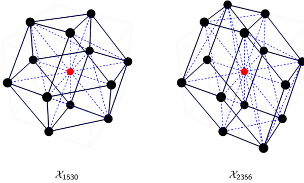
Fig. 15. Toric diagrams for reflexive toric Calabi–Yau 4-folds \mathcal{X}_{1530} and \mathcal{X}_{2356} . The value for V(b_i^*; Y) \chi(\widetilde{X(\Delta)}) for these is the largest amongst all 4319 reflexive toric Calabi–Yau 4-folds
