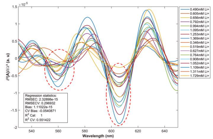
Fig 4. Second derivative spectra of therapeutic concentrations of lithium in blood in the range 530-650 nm after undergoing pre-treatment of baseline and peak shift corrections, Savitsky-Golay filtering and normalization. Prominent bands found at 605 nm and 560 (circled).
