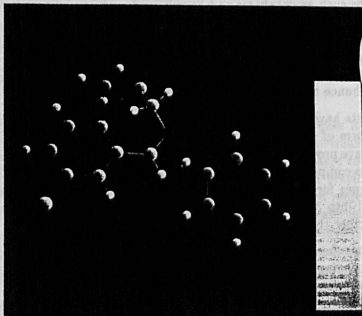
Figure 2.4: Graphical Representation Used in Molecular Modelling
