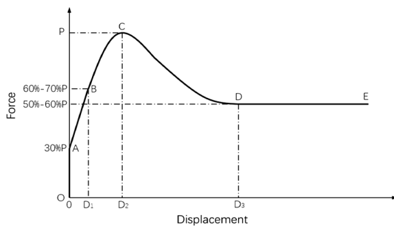
Fig. 8 Force and displacement behaviour curve.
