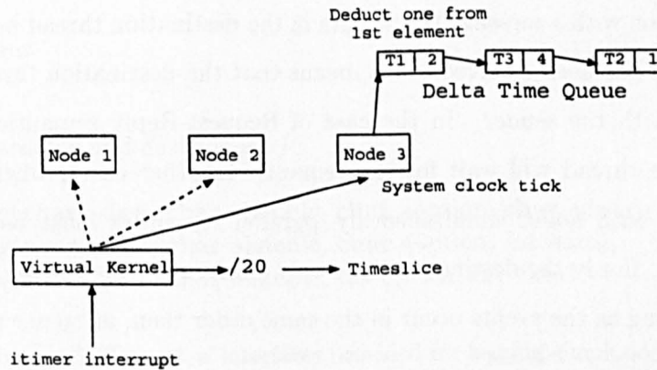
Figure A.7: The use of an 'itimer' to provide per node interrupt timer support for threads
