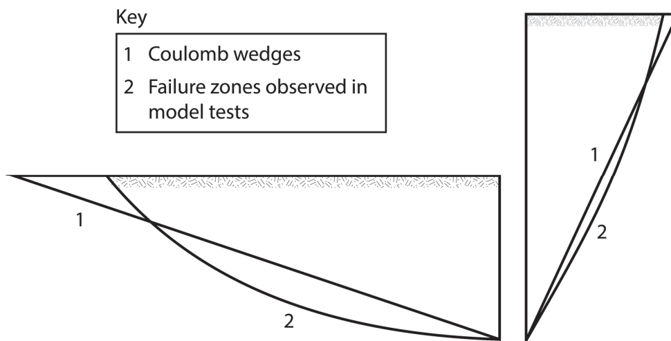
Figure 5. 8 Comparison of failure modes behind and in front of a retaining wall (after Padfield and Mair, 1984).
