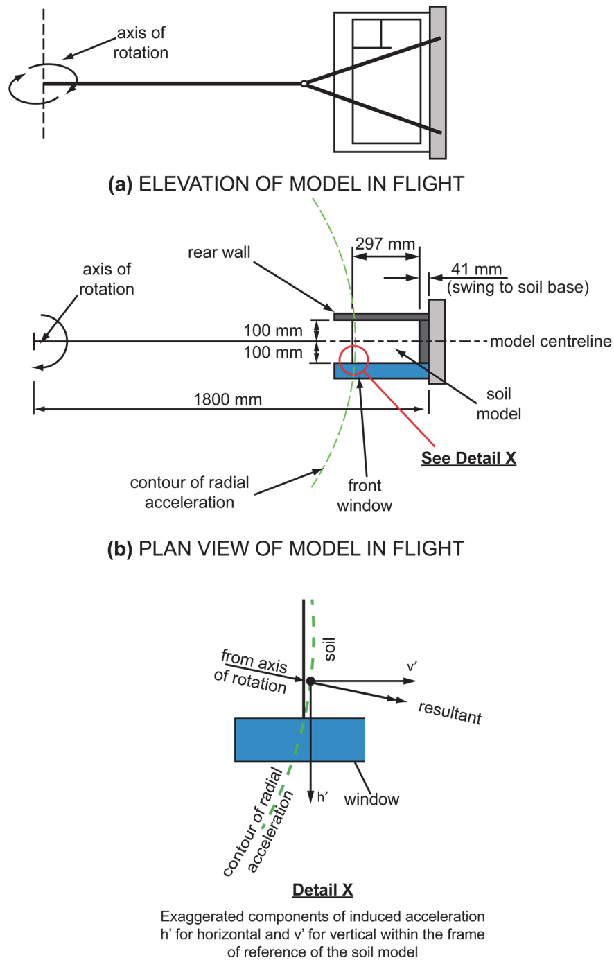
Figure 4. 3 Geometry of a typical model on the Acutronic 661 geotechnical centrifuge at City, University of London showing a) elevation of the model in flight; b) plan view of model in flight with components of induced acceleration (after Grant, 1998).
