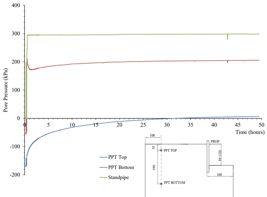
Figure 6. 68 Typical response of the far field PPTs and standpipe PT during consolidation prior to testing.
