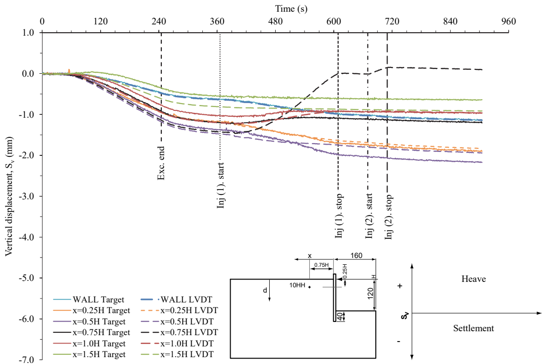
Figure 6.12 Retained surface vertical displacements measured by LVDTs and image processing targets (15 mm below the surface) in test 10HH above the wall and at distances x = 0.25H , 0.5H , 0.75H , 1.0H and 1.5H behind the wall.
