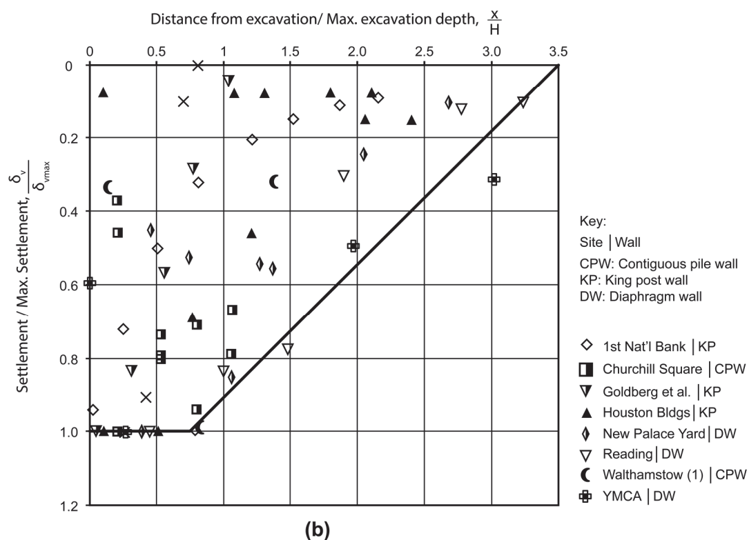
Figure 2. 15 (a) Normalised ground surface displacements due to excavation and (b) settlements normalised against maximum settlement behind the wall in stiff clays (after Gaba et al. , 2017).
