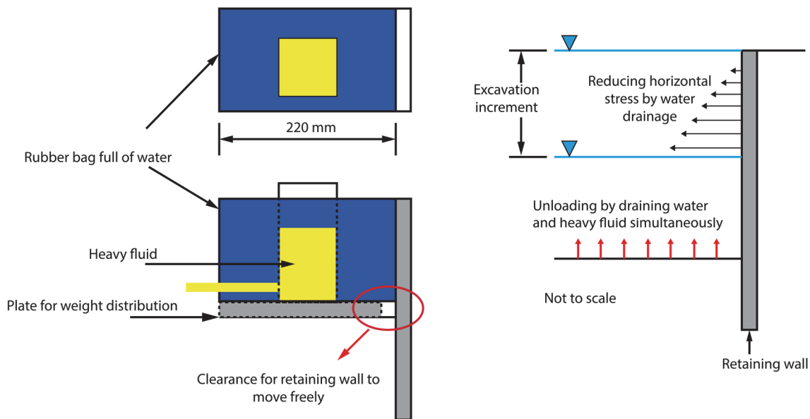
Figure 5.1 Simulation of excavation methods using two fluids adopted by: (a) McNamara (2001) and (b) Elshafie (2008).
