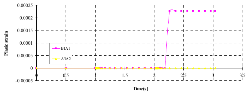
Fig.12 Plastic strain of Beam of B1A1 and A3A2 at level 14 of Case 2
