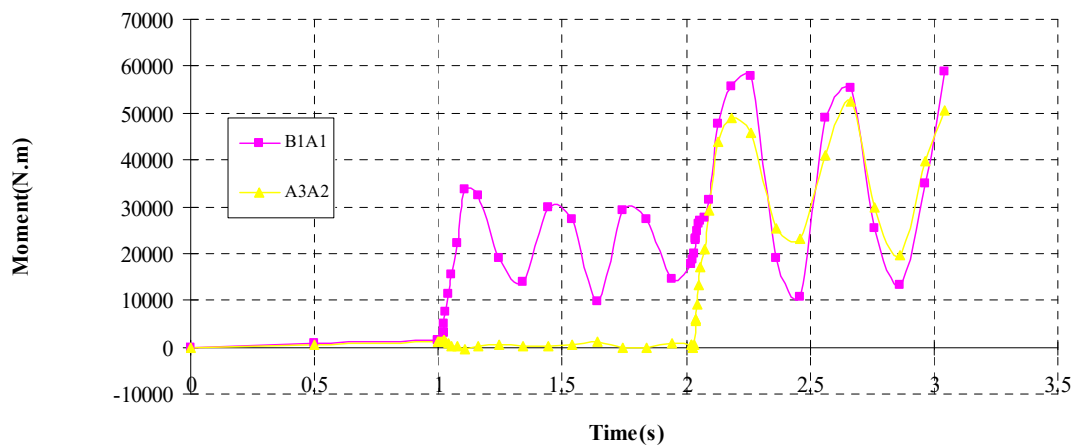
Fig.6 Major Moment of Beam B1A1 and A3A2 at ground level of Case 1
