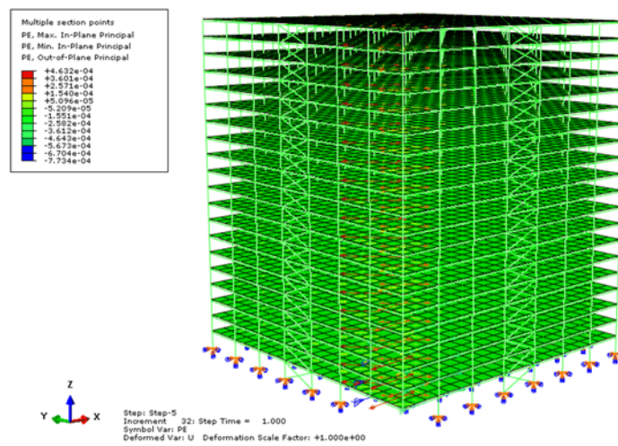
Fig.4 Tensor distribution of plastic strain of concrete slab
