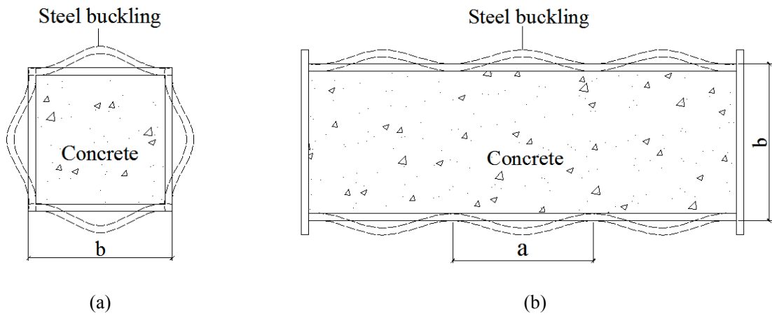
Fig.11 Boundary conditions of plates in square CFST (a) in cross sections; (b) along longitudinal direction
