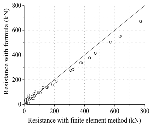
Fig. 13 Verification of formula for elastic buckling strength f'_{cr}
