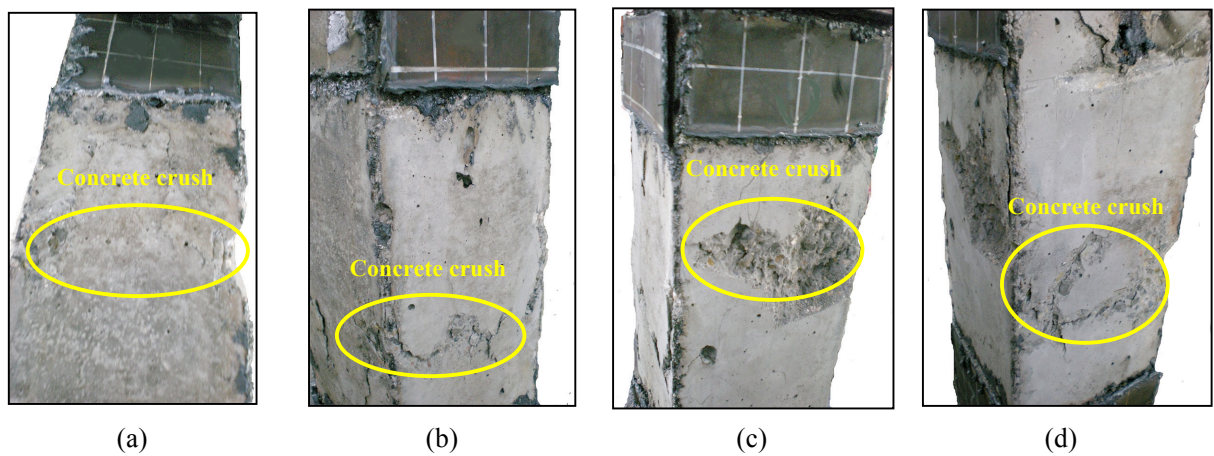
Fig. 8 Concrete failure mode of the S5 specimen (a) Surface 1; (b) Surface 2; (c) Surface 3; and (d) Surface 4
