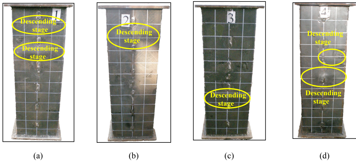
Fig. 7 Buckling mode of the S9 tube (a) Surface 1; (b) Surface 2; (c) Surface 3; and (d) Surface 4
