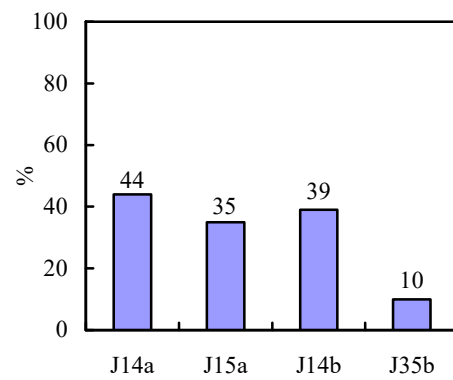
(b) ratio of local indentation dissipated energy to total energy
