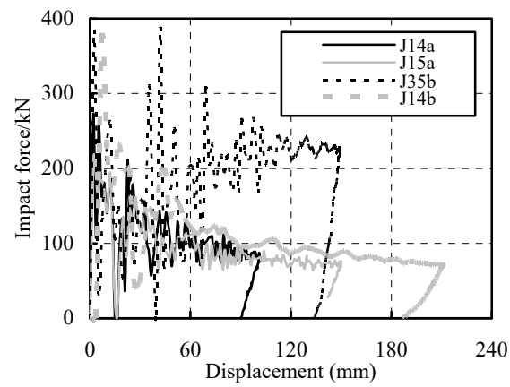
Figure 16 Measured impact load versus displacement curves of Specimens J14a, J14b, J15a and J35b
