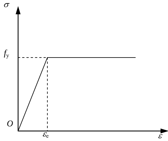
Figure 2 Material model of steel
