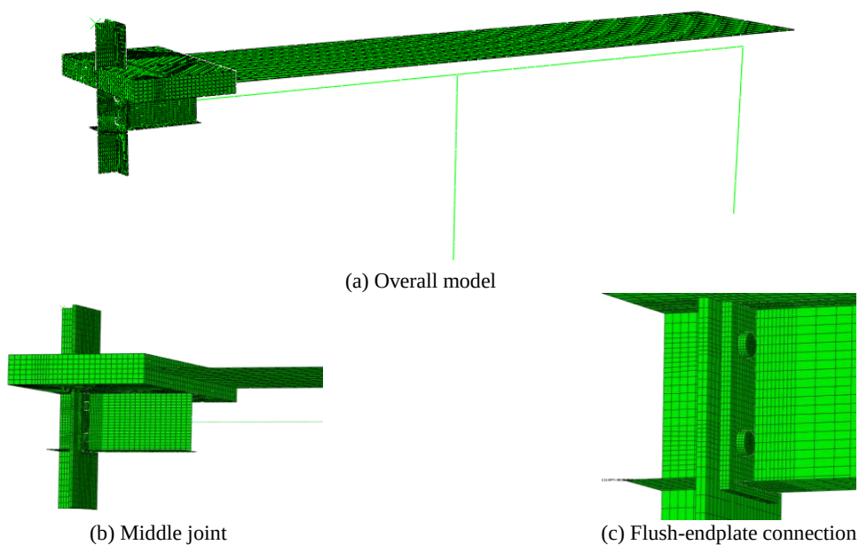
Fig. 8 Finite element model
