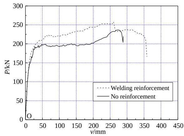
Fig. 16 Analysis result of welding reinforcement
