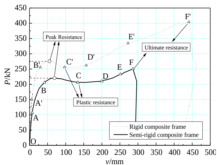
Fig.6 Comparison between rigid composite frame and semi-rigid composite frame
