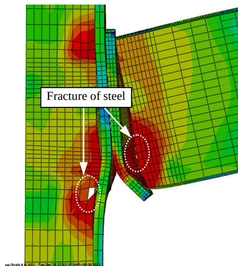
Fig. 14 Fracture of steel corresponding to the ultimate resistance
