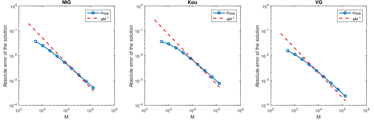
Figure 8: Error convergence for the continuously monitored double-barrier option. The absolute error is worse than that for the single-barrier option but the error convergence conforms to the calculated error bound.
