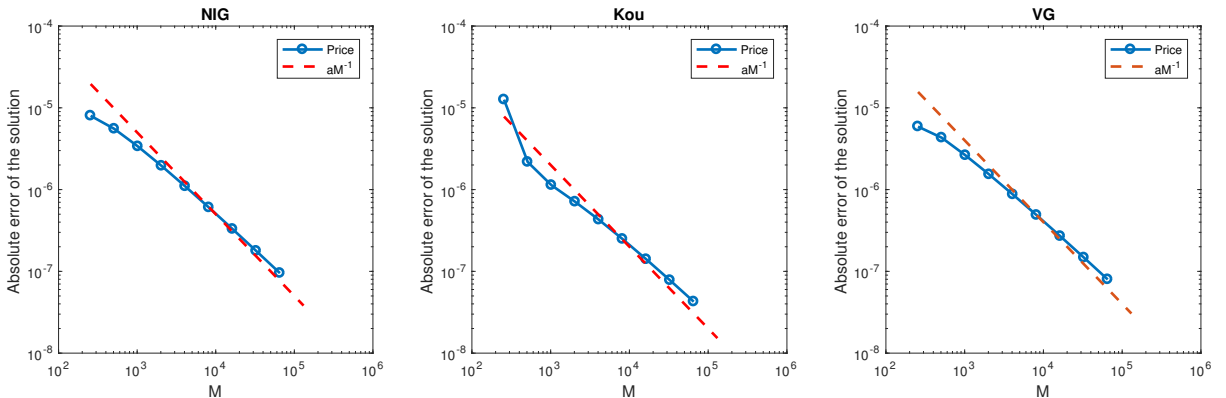
Figure 7: Error convergence for a continuously monitored single-barrier option. The error convergence conforms to the calculated error bound (only the first point of the Kou process deviates slightly from the overall behaviour) and shows the typical sub-polynomial error convergence for higher values of M .
