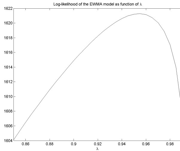
Figure 13: Log-likelihood of the EWMA model with reference to Gasoline prices for the period January 4th, 2010 to August 31st 2015.
