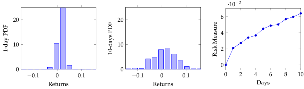
Figure 16: Left panel: Simulated 1-day log-return distribution. Middle panel: Simulated 10-days log-return distribution. Right panel: VaR term structure.
