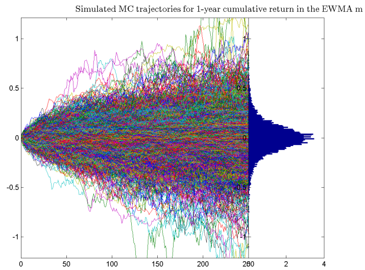
Figure 14: Simulated Paths of the EWMA Model.
