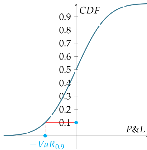
Figure 1: For a continuous r.v., the VaR is determined by the abscissa at which the CDF equals the level 1 - \alpha .
