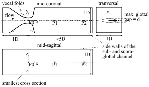
Fig. 2 Geometrical shape of the computational domain with dimensions based on the channel width D (derived from the tracheal diameter of about 0.02m), the glottal cross section is depicted in fully opened configuration with the maximum glottal gap d , P_0 to P_2 are defined for the evaluation of flow quantities
