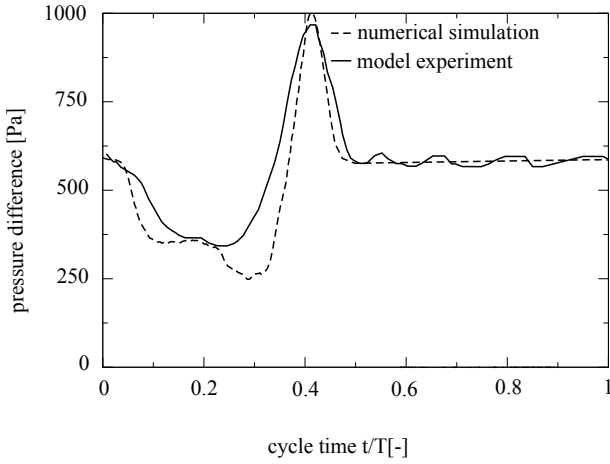
Fig. 10 Temporal evolution of the trans-glottal pressure difference between the points p_{up} and p_{down} sketched in figure 1, compared for experimental and numerical model
