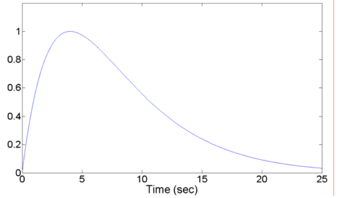
Figure 3. The Bogdanoff-Golberg-Bernard modulating function for t_p = 4\text{sec}
