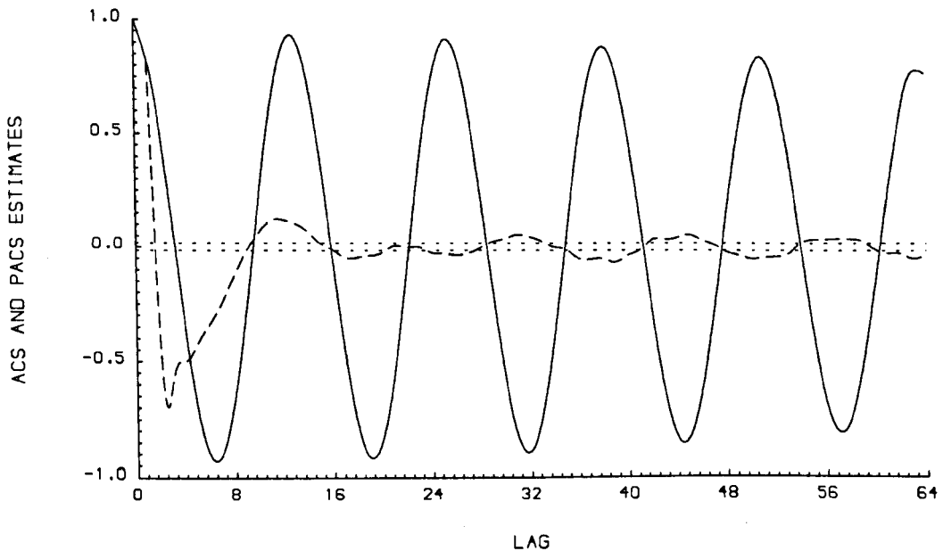
Fig. 2.3 Estimated ACS (continuous line) and PACS (broken line) of the central 500 samples of the fringe pattern in Fig. 1.5, averaged over 30 independent realisations. The dashed lines denote the 95 % confidence limits of the estimates [41, 42, 43].
