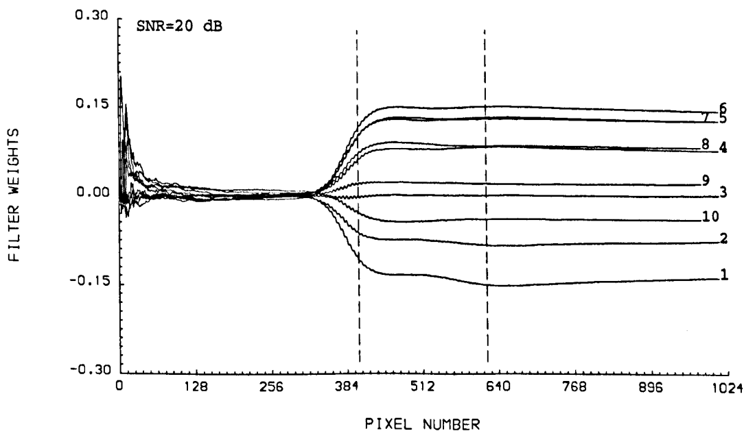
Fig. 4.12 RLS weights with a SNR of 20 dB.
