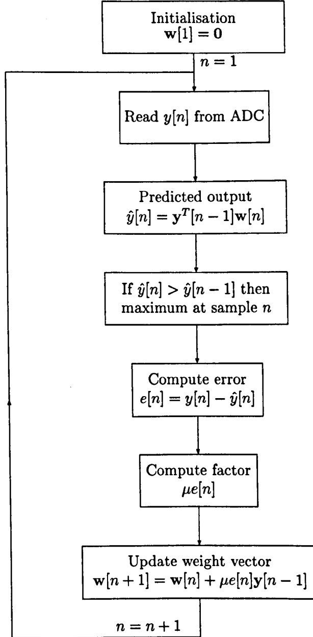
Fig. 3.2 Flowchart for on-line prediction of the WLI output with the LMS algorithm.
