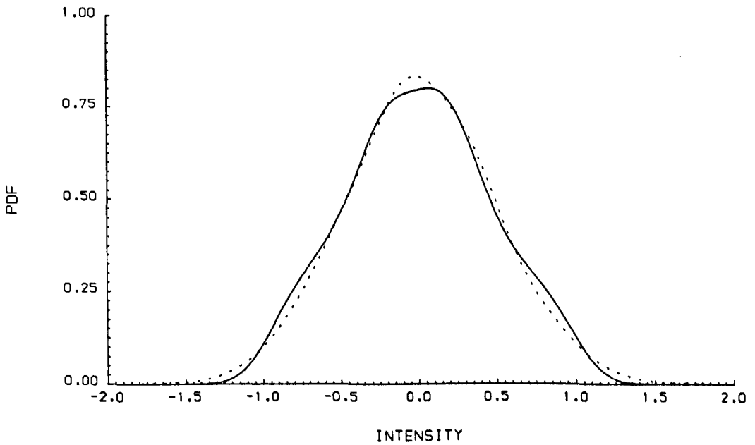
Fig. 7.1 Density of the central 26 fringes of Fig. 4.13, smoothed using a Gaussian window [11]. The dashed curve shows the density of a Gaussian sequence of the same length and variance.
