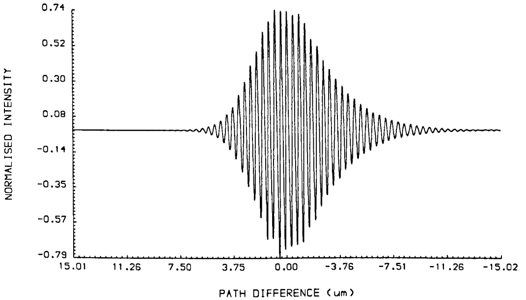
Fig. 4.15 The fringe pattern in Fig. 4.13 filtered by the LMS with p = 32 and \mu = 0.01 .
