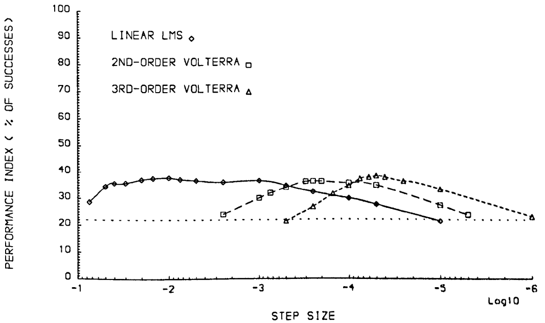
Fig. 7.7 Performance of linear and Volterra filters for the non-linear signal in Fig. 7.3.
