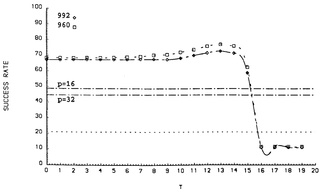
Fig. 5.9 Success rate with the centroid and covariance methods over operating ranges of 992 and 960 pixels. The dashed bottom line refers to the direct visibility method.
