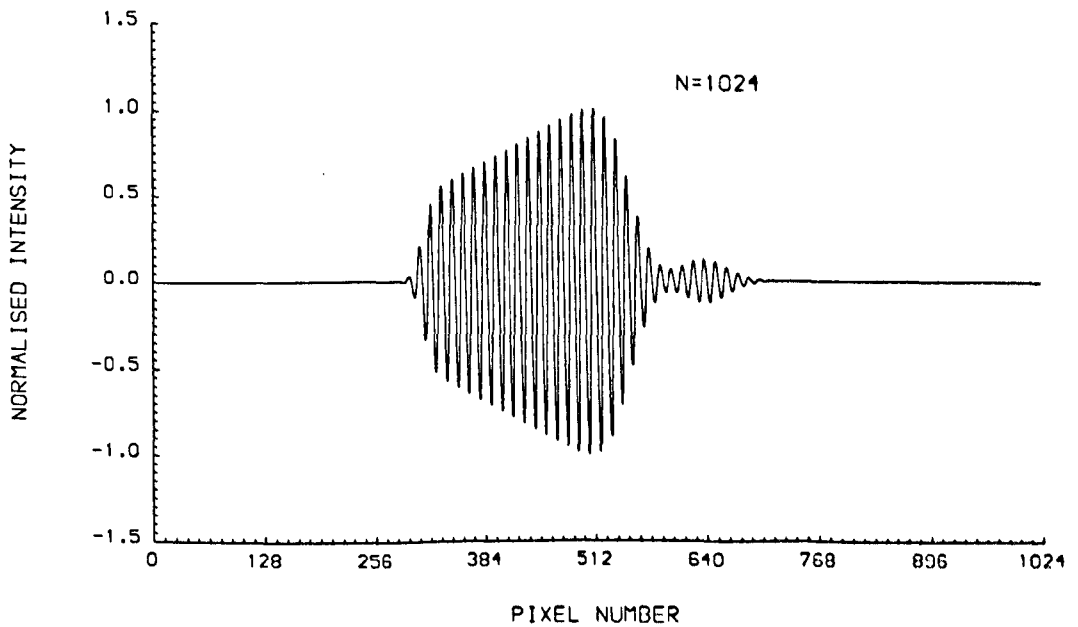
Fig. 7.5 A noise-free fringe pattern modified by chromatic aberrations.
