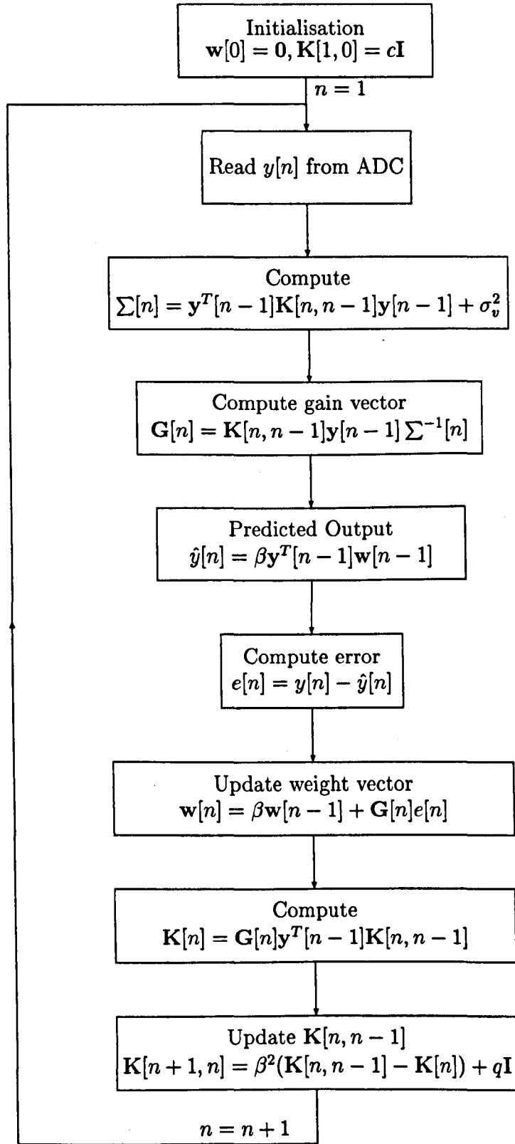
Fig. 3.4 Flowchart for on-line prediction of the WLI output with the Kalman filter.
