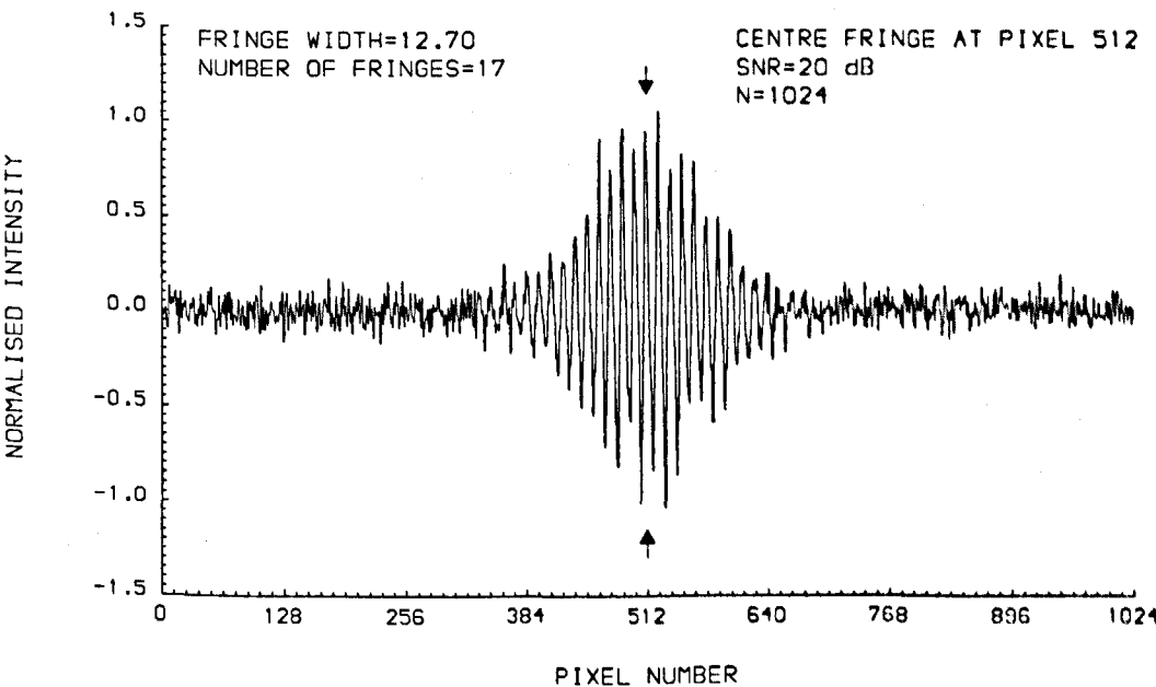
Fig. 7.4 A noise-corrupted fringe pattern distorted by a cubic non-linearity.
