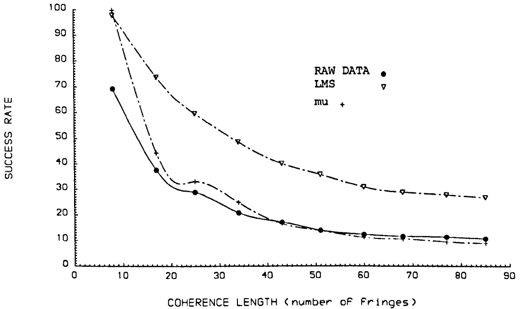
Fig. 4.18 Success rate against coherence length for a SNR of 26 dB (5 % noise) and p = 16 . Also shown is \mu_0 (amplified 555 times).
