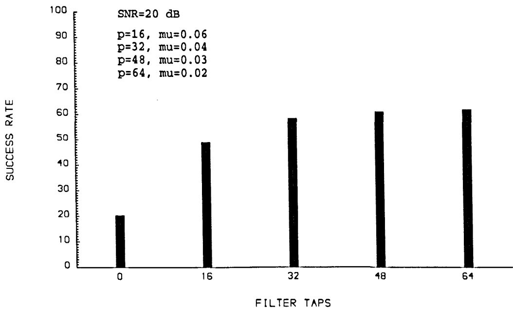
Fig. 4.2 Maximum success rate (out of 500 trials) against filter order at 20 dB.
