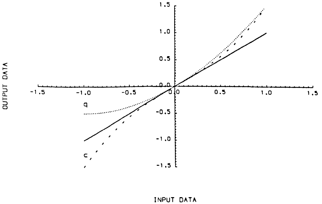
Fig. 7.2 Two common ADC non-linearities: q) quadratic; c) cubic.
