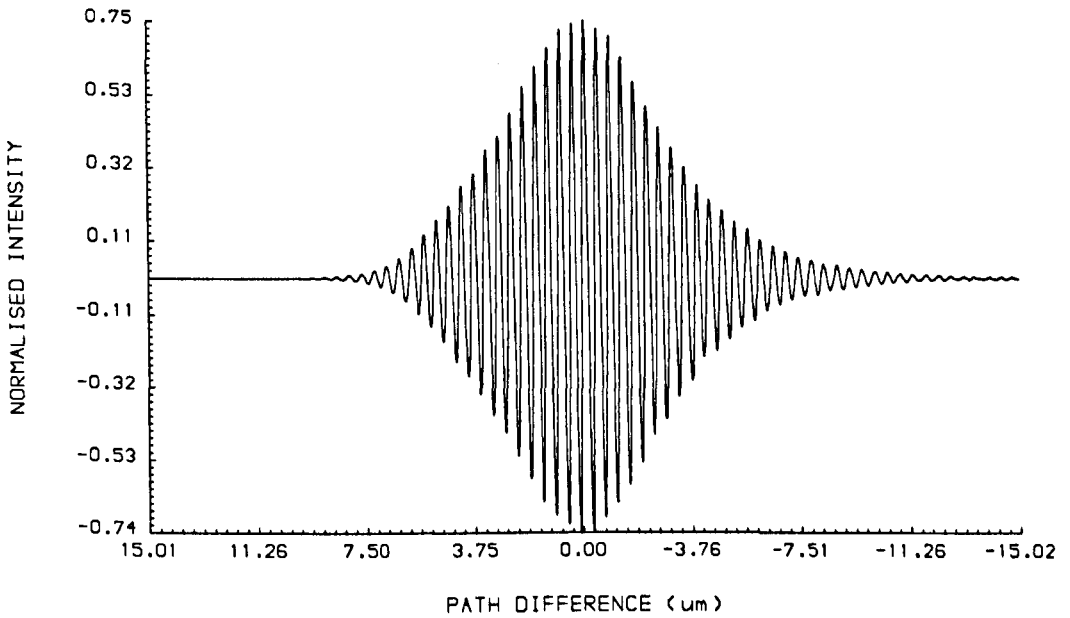
Fig. 4.14 The fringe pattern in Fig. 4.13 filtered by the LMS with p = 32 and \mu = 0.1 .
