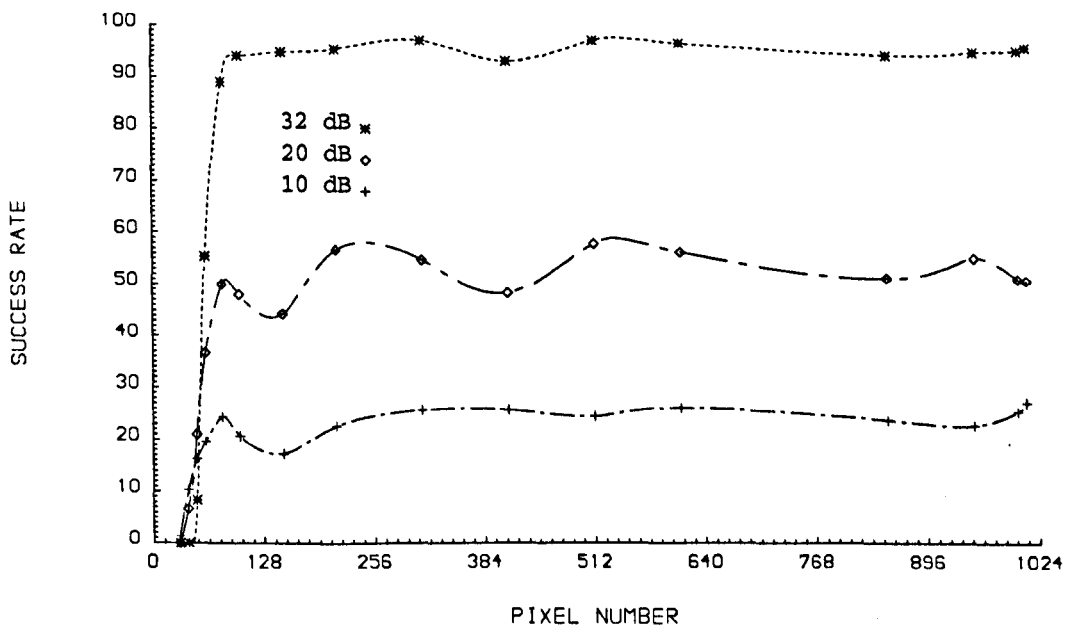
Fig. 4.4 Success rate (out of 300 trials) with the LMS algorithm against central fringe position, with p = 32 and \mu optimised for the central pixel on the CCD array.
