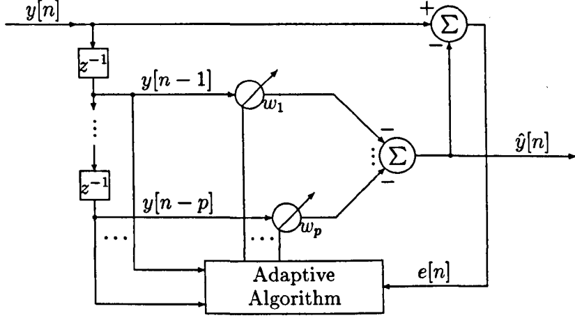
Fig. 3.1 FIR adaptive transversal filter.
