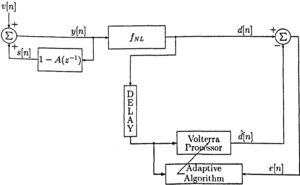
Fig. 7.6 AR model signal generator and FIR adaptive non-linear filtering.
