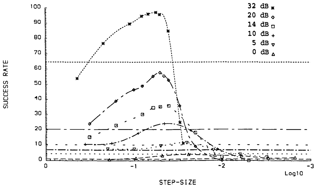
Fig. 4.3 Success rate (out of 500 trials) against \mu and SNR, with p = 32 . The horizontal lines refer to the direct visibility method.
