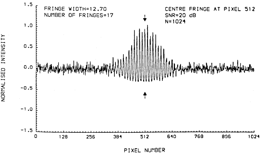
Fig. 7.3 A noise-corrupted fringe pattern distorted by a quadratic non-linearity.
