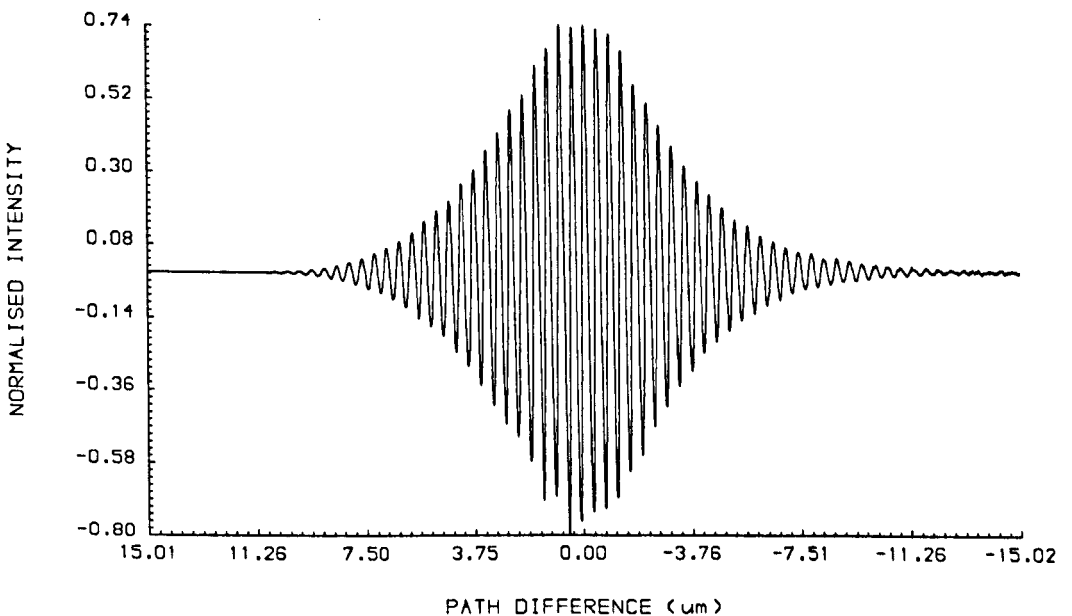
Fig. 4.16 The fringe pattern in Fig. 4.13 filtered by the RLS with p = 32 and \lambda = 1.0 .
