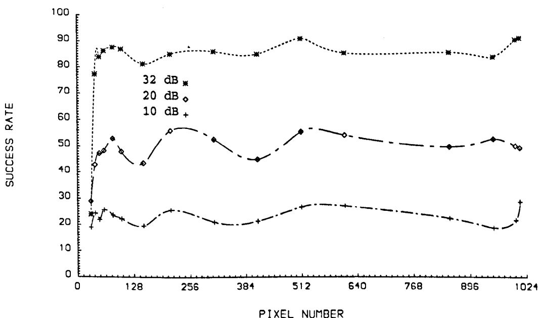
Fig. 5.2 Success rate with the thresholded technique against central fringe position, with p = 32 and \mu optimised for the central pixel on the CCD array.
