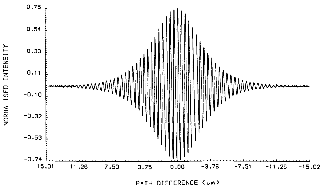
Fig. 4.17 The fringe pattern in Fig. 4.17 filtered by the RLS with p = 32 and \lambda = 0.8 .
