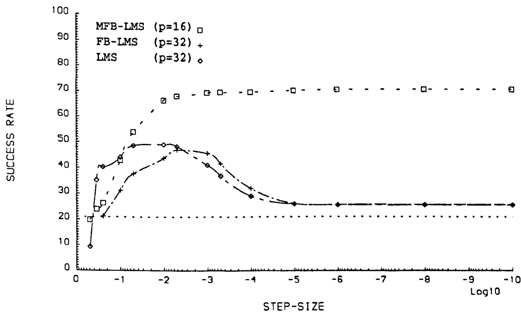
Fig. 5.10 Success rate with the LMS predictors over an operating range of 992 pixels. The dashed bottom line refers to the direct visibility method.
