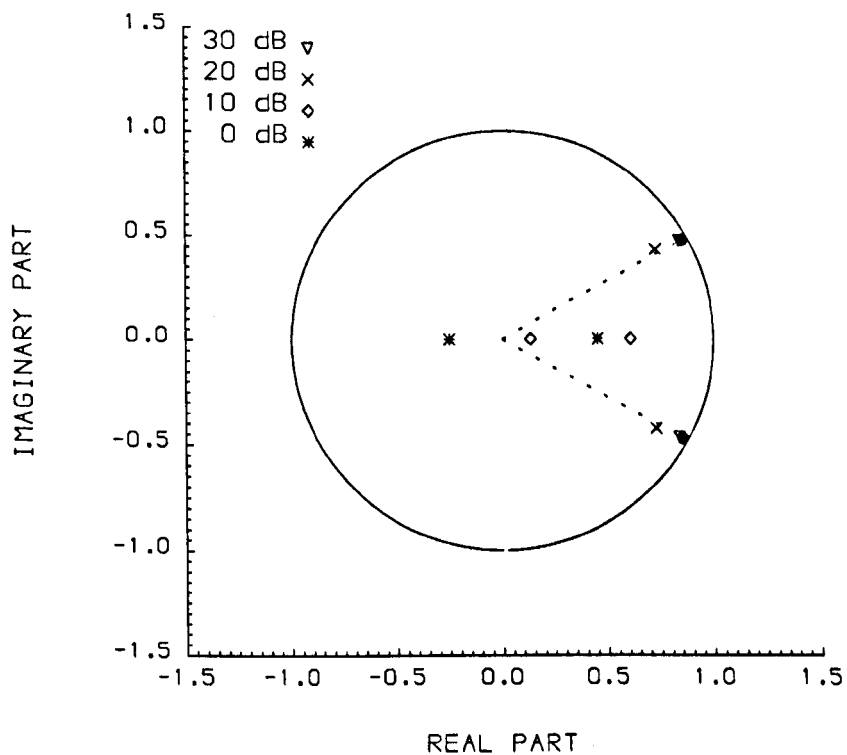
Fig. 5.3 Position of AR(2) model poles against SNR. The SNR = \infty case is shown with bullets.
