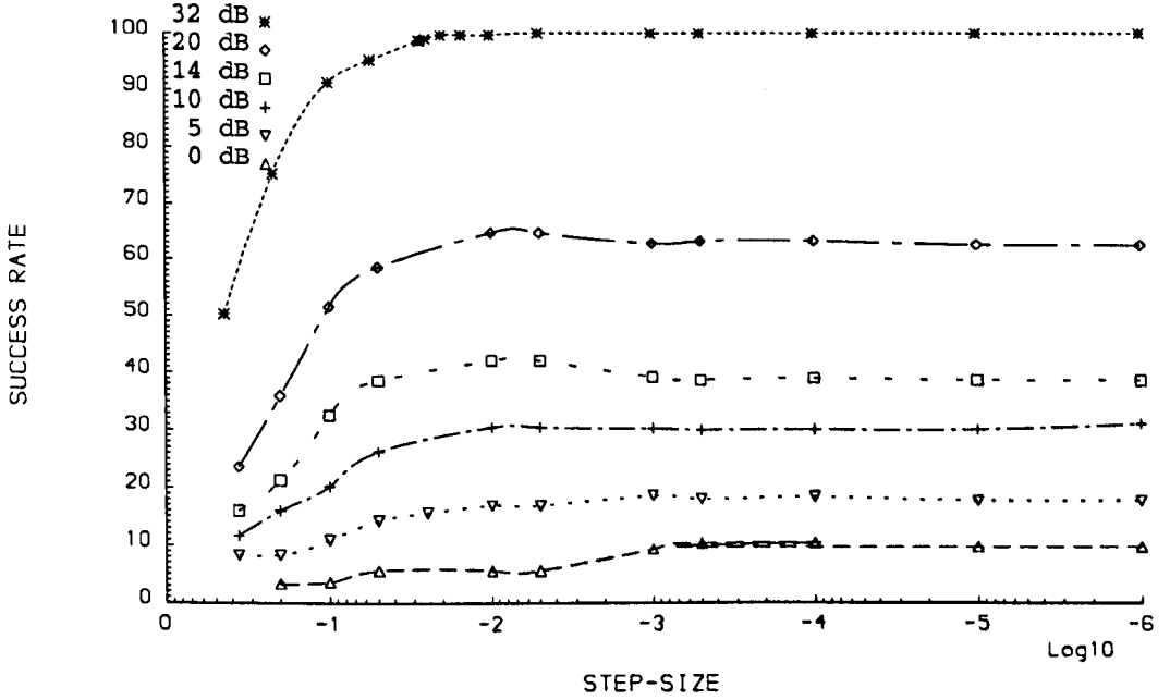
Fig. 5.5 Success rate with the thresholded MFB-LMS against \mu and SNR out of 500 simulated scans with p = 16 .
