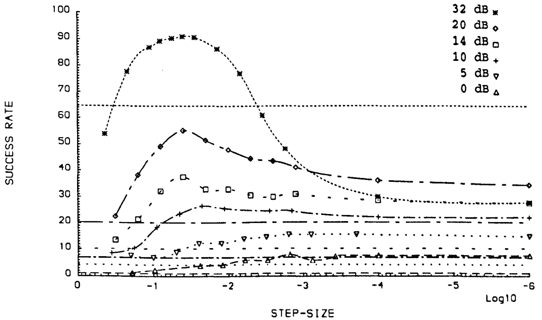
Fig. 5.1 Success rate with the thresholded technique against \mu and SNR, with p = 32 . The horizontal lines refer to the direct visibility method.
