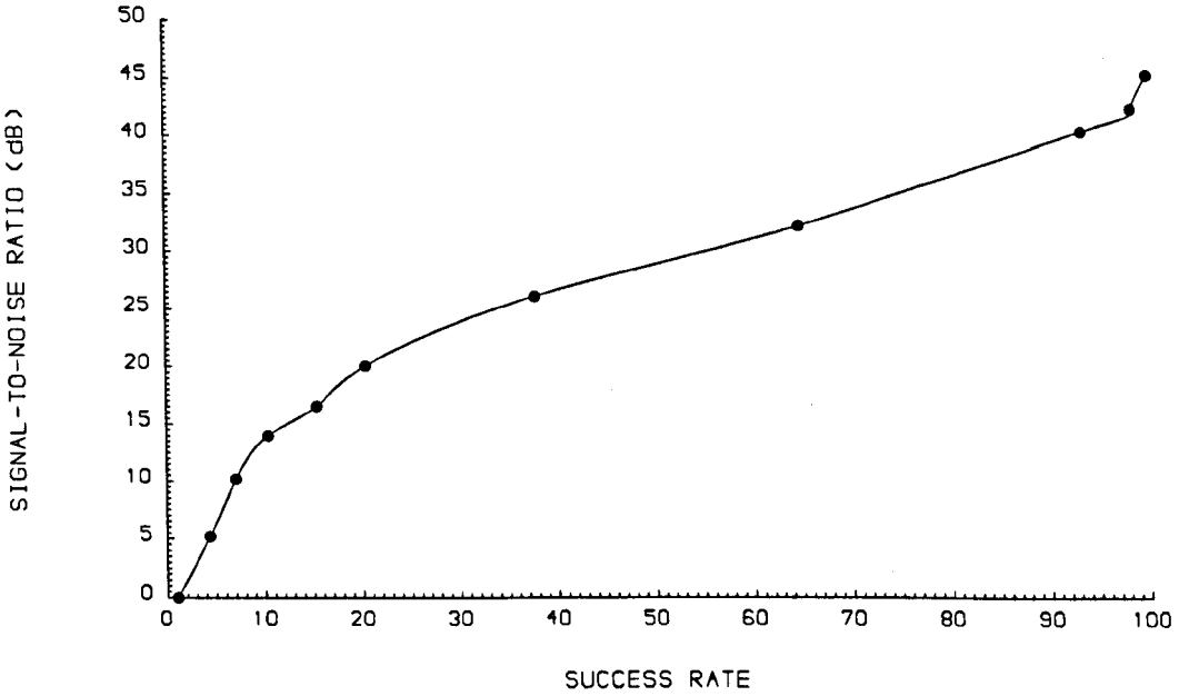
Fig. 1.6 Success rate from direct observation of the visibility profile for various SNRs.
