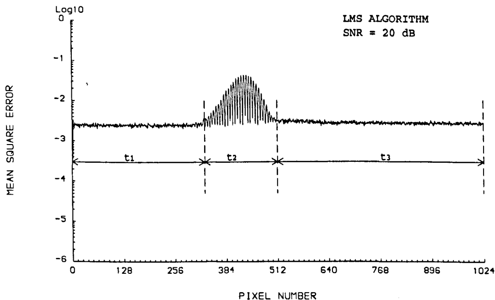
Fig. 4.6 LMS MSE with a SNR of 20 dB. The noise variance was -2.6 on a log scale.
