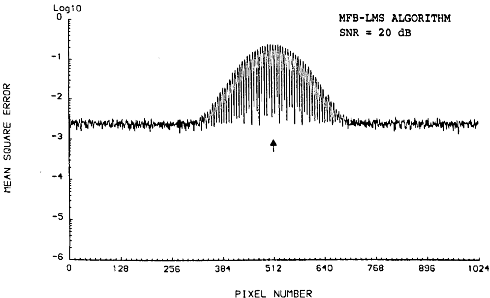
Fig. 5.7 MSE across the CCD array with the thresholded MBF-LMS algorithm and \mu = 10^{-6} .
