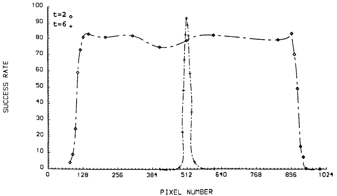
Fig. 5.8 Success rate (out of 300 trials) with the centroid method against central fringe position.
