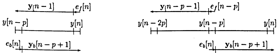
Fig. 5.4 Schematic diagram showing the difference between the original FB-LMS (left) and the modified form (right).
