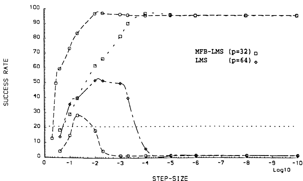
Figure 5.11 Success rate with the LMS predictors over an operating range of 960 pixels. In circles is the rate with weights fixed during the sensing phase.
