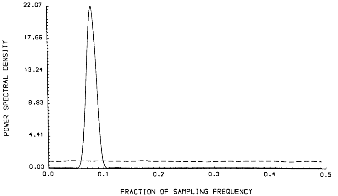
Fig. 2.2 Estimated spectrum of the central 500 samples of the fringe pattern in Fig. 1.5, smoothed with the Parzen window [40] and averaged over 30 independent realisations. The broken line represents the spectrum of a pseudo-random white Gaussian process.
