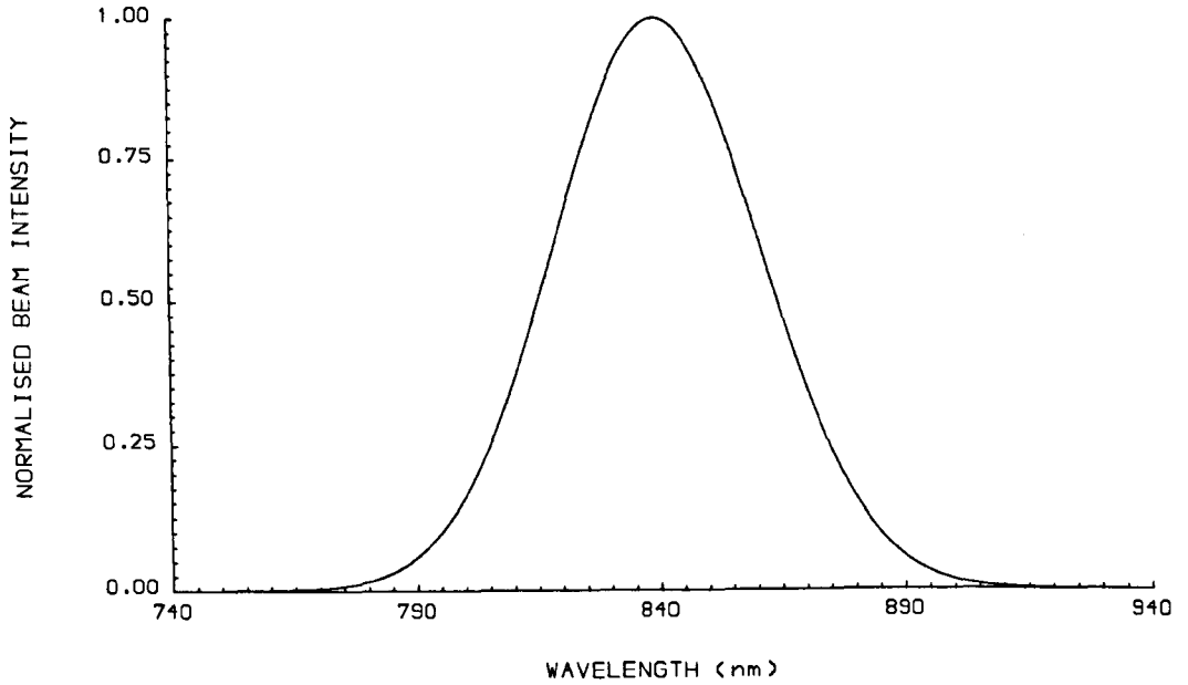
Fig. 1.2 Typical spectrum of an AlGaAs LED, emitting at a central wavelength of 840\text{ nm} with a spectral half-width of 49.4\text{ nm} .
