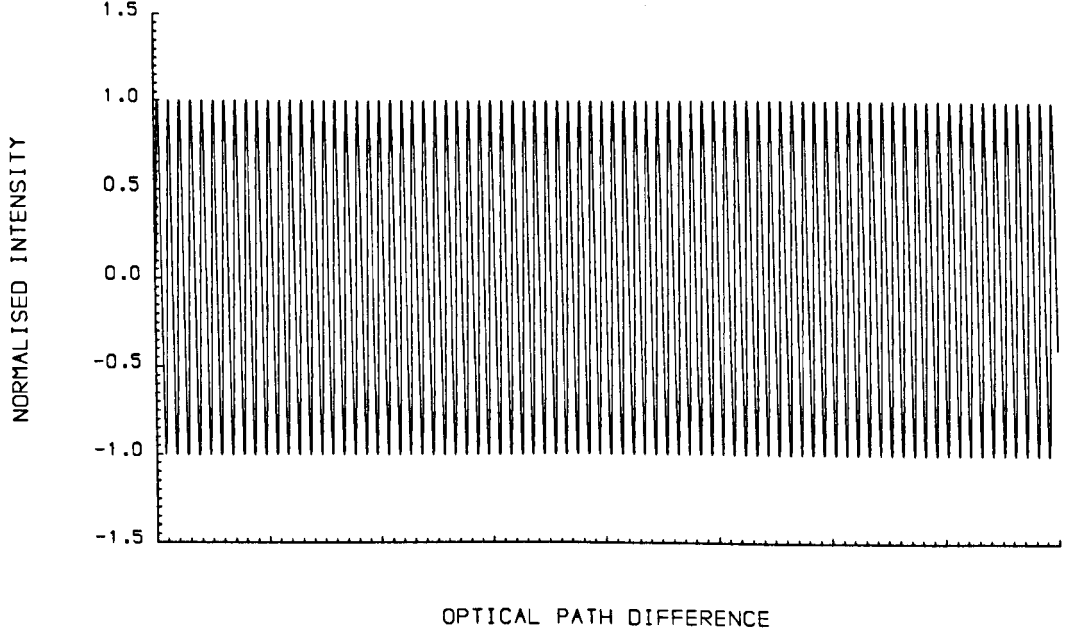
Fig. 1.1 Output intensity with a He-Ne laser source. L_c = 1000 \text{ m} , corresponding to 1.58 \times 10^9 fringes.
