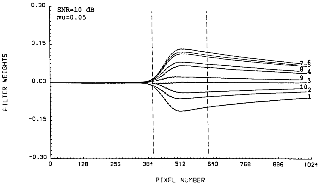
Fig. 4.10 LMS weights with a SNR of 10 dB.
