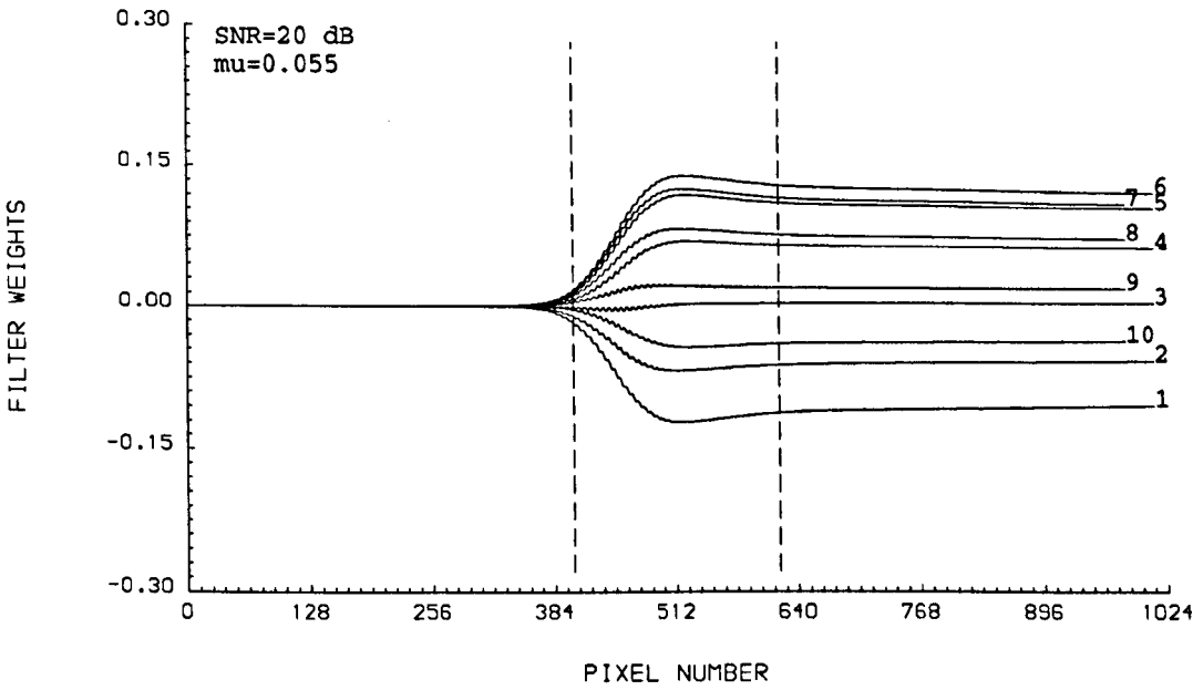
Fig. 4.9 LMS weights with a SNR of 20 dB.
