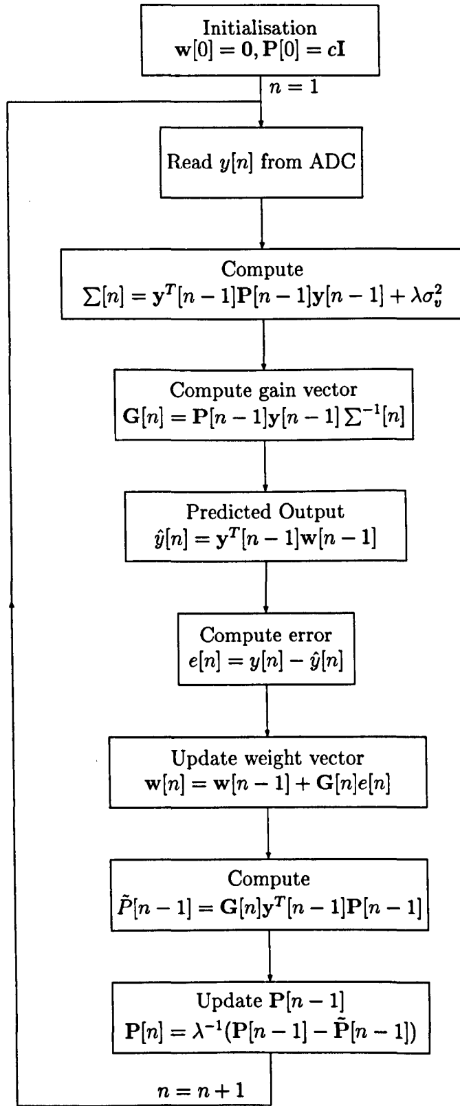
Fig. 3.3 Flowchart for on-line prediction of the WLI output with the RLS algorithm.
