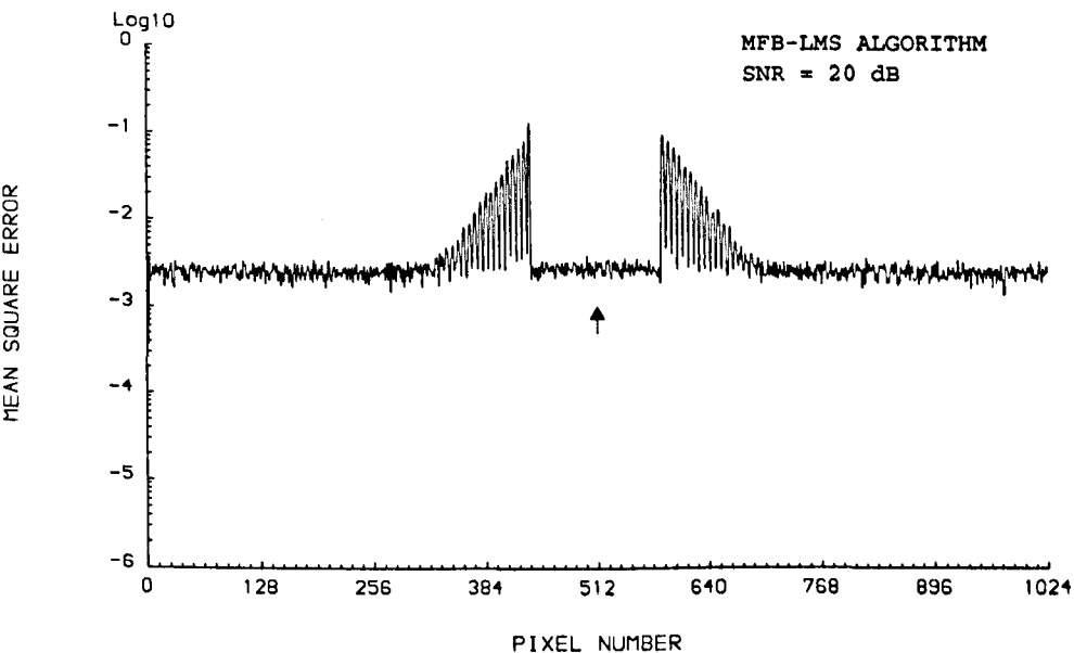
Fig. 5.6 MSE across the CCD array with the thresholded MBF-LMS algorithm and \mu = 10^{-3} .
