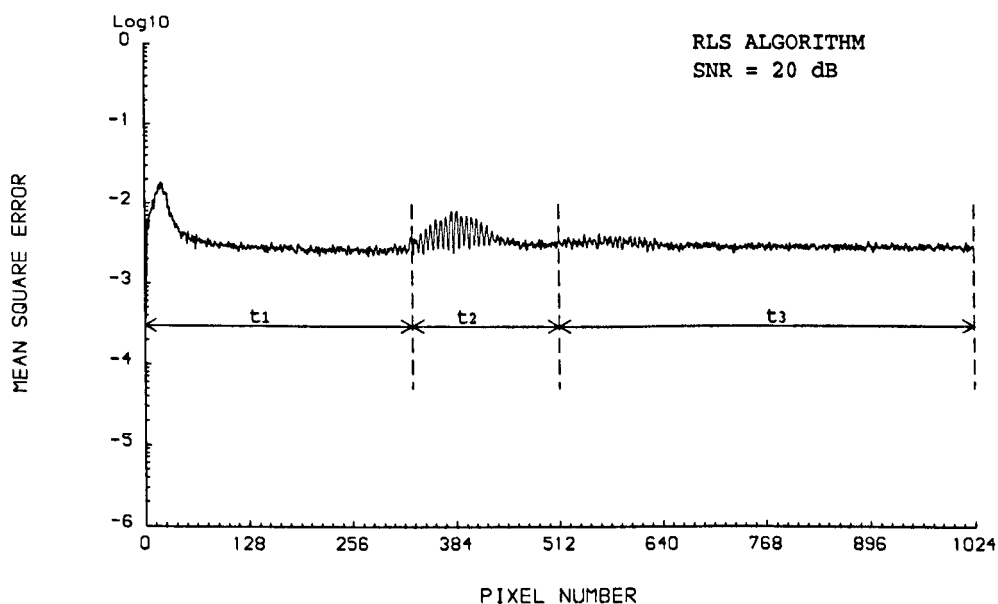
Fig. 4.11 RLS MSE with a SNR of 20 dB. The noise variance was -2.6 on a log scale.
