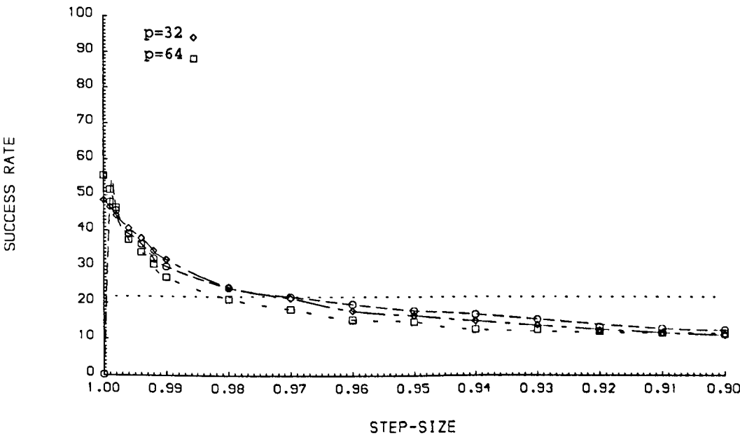
Fig. 5.12 Success rate with the RLS predictor over operating ranges of 992 pixels ( p = 32 ) and 960 pixels ( p = 64 ). In circles is the rate with the 64 weights fixed during the sensing phase.
