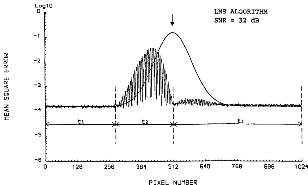
Fig. 4.5 LMS MSE across the CCD array with a SNR of 32 dB. The noise variance was -3.8 on a log scale. The superimposed fringe visibility profile is not to scale.
