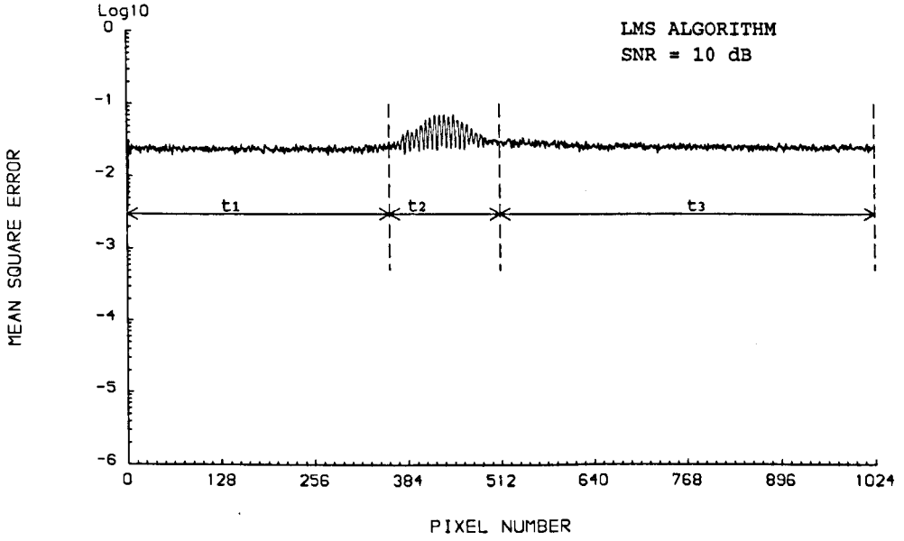
Fig. 4.7 LMS MSE with a SNR of 10 dB. The noise variance was -1.6 on a log scale.
