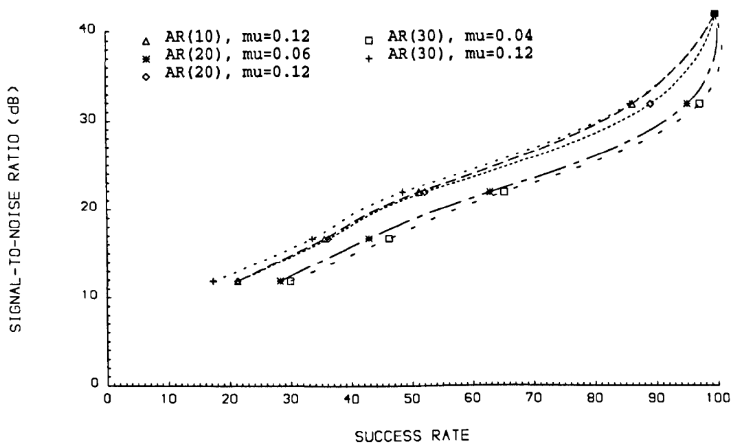
Fig. 4.1 Sub-fringe success rate (out of 500 trials) with the LMS algorithm.
