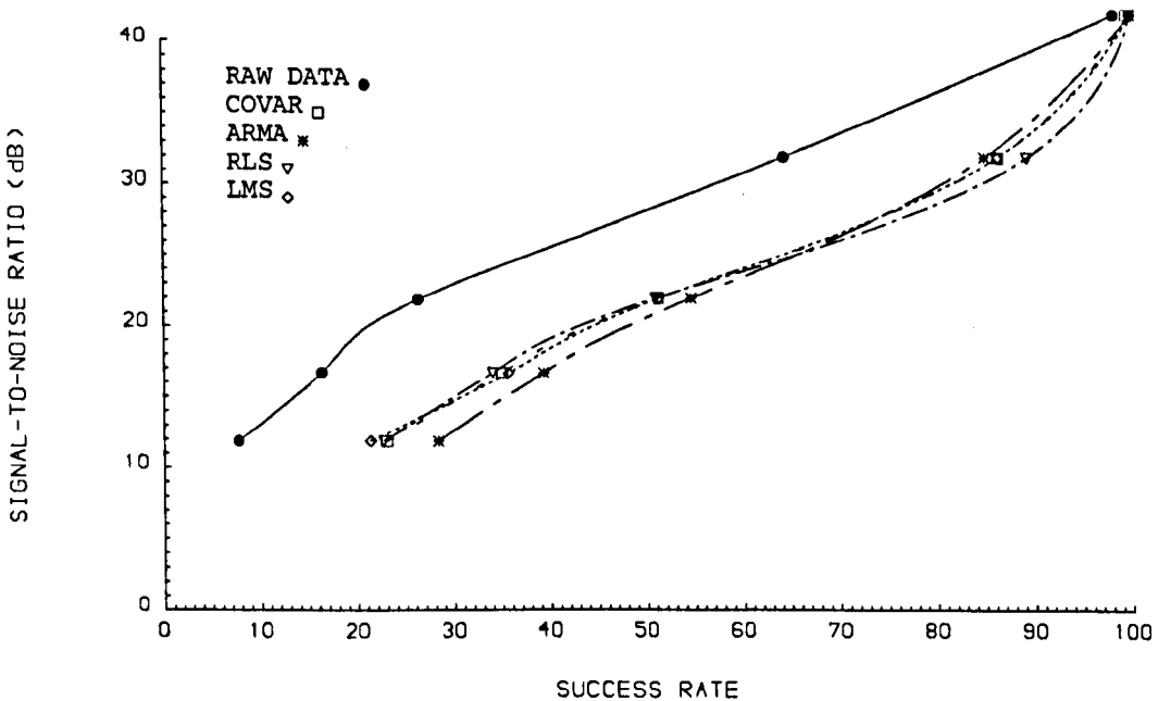
Fig. 3.5 Sub-fringe success rate with batch and adaptive algorithms out of 500 scans.
