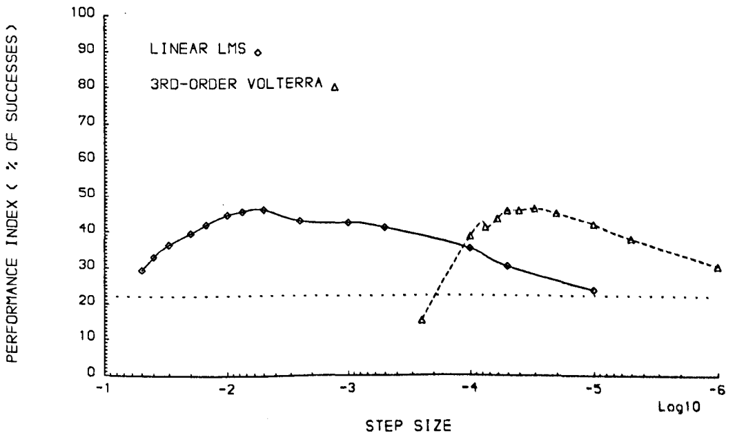
Fig. 7.8 Performance of linear and Volterra filters for the non-linear signal in Fig. 7.4.
