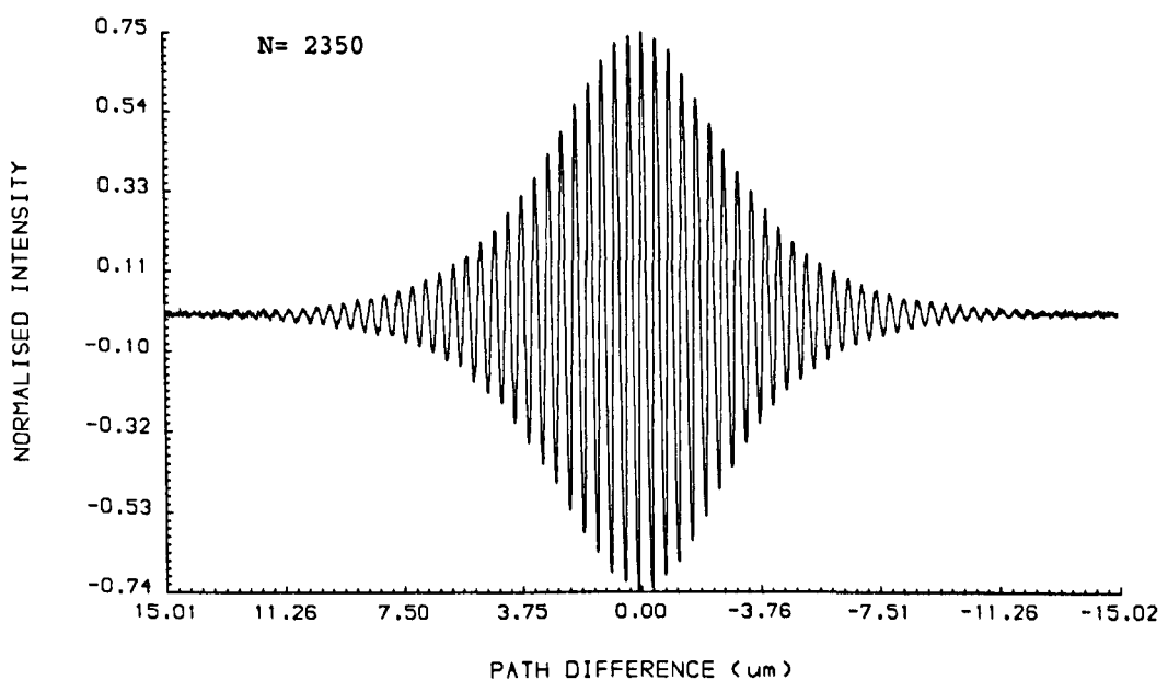
Fig. 4.13 Experimentally obtained white-light fringe pattern using a broad-band source and a mechanical scanner (after pre-processing).
