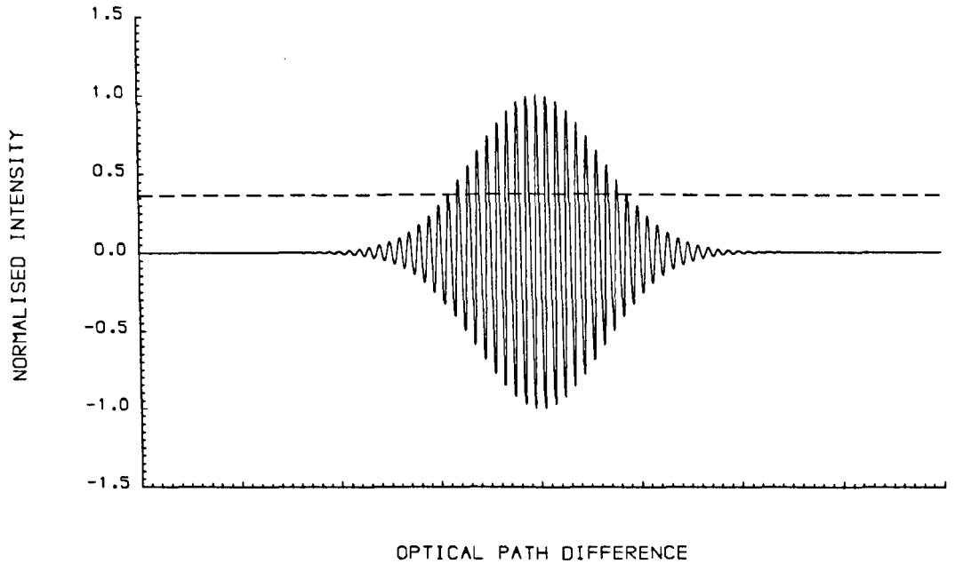
Fig. 1.3 Output intensity of an interferometer with a LED source, obtained by adding 201 wavelengths spaced by 1\text{ nm} and in phase at \delta L = 0 , with intensities as in Fig. 1.2. L_c = 14.3\text{ }\mu\text{m} , corresponding to 17 fringes. The dashed line delimits the 1/e intensity points.
