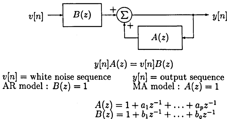
Fig. 2.1 ARMA process driven by white noise.
