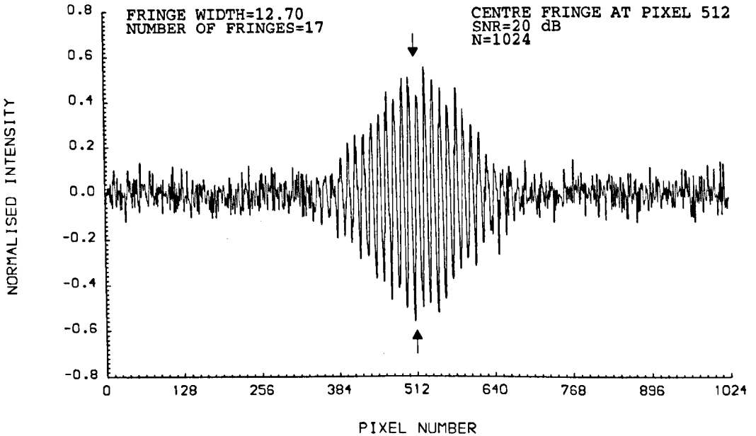
Fig. 1.5 Simulated output intensity of a WLI system with additive noise at 20 dB. The arrows point at the central fringe.
