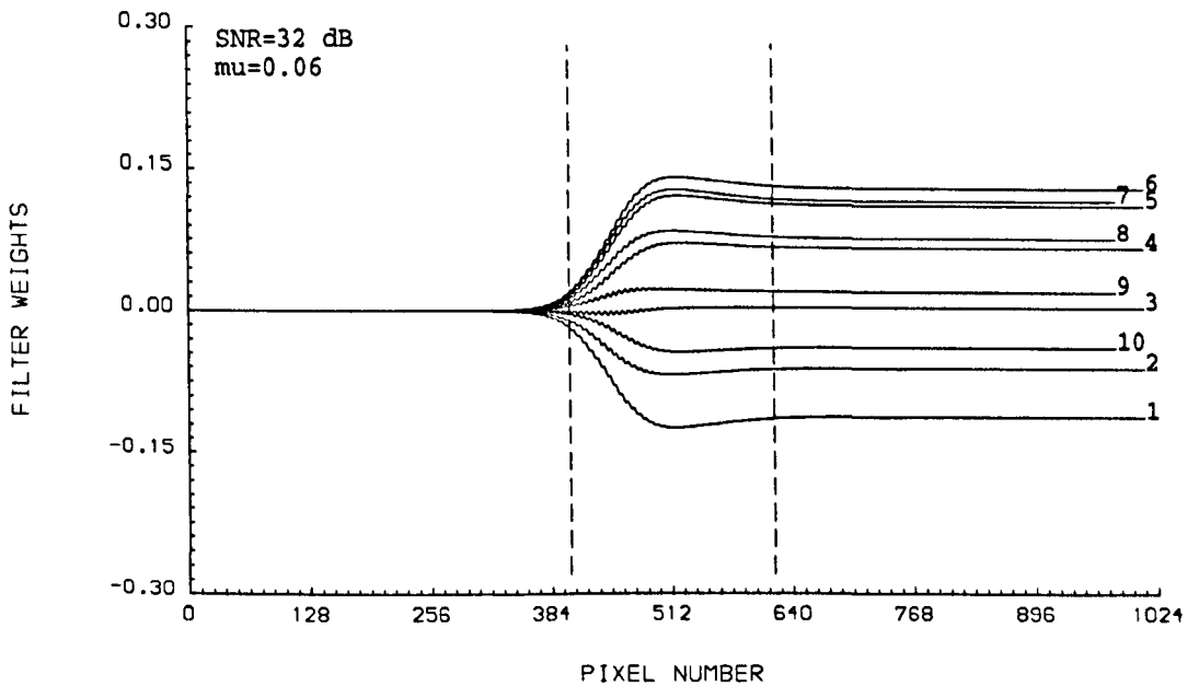
Fig. 4.8 LMS weights with a SNR of 32 dB. The dashed lines delimit the coherence region.
