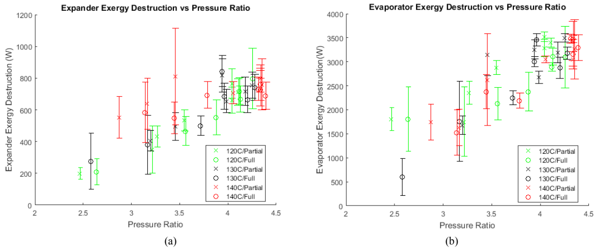
Figure 5: (a) Effect of pressure ratio, heat-source temperature and generator load on expander exergy destruction. (b) Effect of pressure ratio, heat-source temperature and generator load on evaporator exergy destruction.
