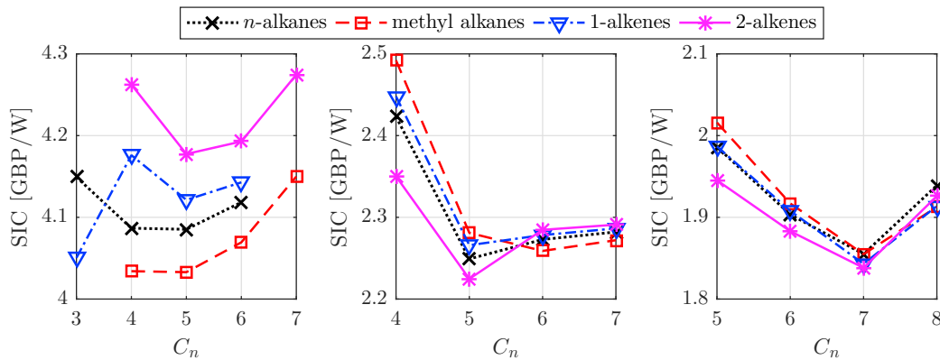
Fig. 4. Specific investment cost (SIC) in £/W for each optimal cycle previously identified in Figure 1. From left to right: T_{hi} = 150, 250, 350\text{ °C} .
