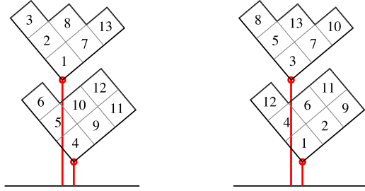
Figure 1. The tableau \mathbf{s}, \mathbf{t}^\lambda \in \text{Std}((3, 2, 1), (3, 2, 2)) .
