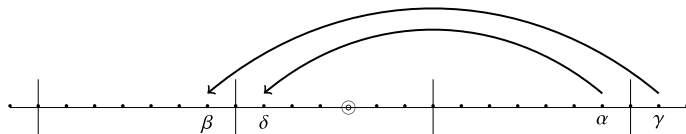
Figure 7. Some simple homomorphisms from affine vertices. This is the projection of \mathbb{E}_{3,2}^\oplus onto the line \mathbb{R}\{\varepsilon_2, \varepsilon_5\}/(\varepsilon_2 + \varepsilon_5) .
