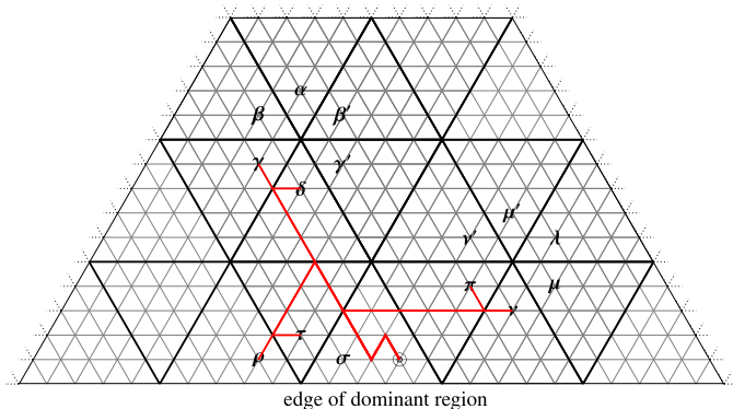
Figure 10. The six elements of \text{Path}^+(-, \mathfrak{t}^\nu) in the geometry of type A_1 \subseteq \widehat{A}_2 . Each of the pairs (\alpha, \lambda) , (\beta, \mu) , (\gamma, \nu) , and (\delta, \pi) are related by an affine vertex reflection (as are their primed versions) and so these pairs are generic sets as in Section 10.3. The pairs (\mu', \rho) , (\nu', \tau) , (\pi, \sigma) are all generic sets as in Section 10.3.
