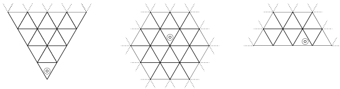
Figure 9. Geometries of type A_2 \subseteq \widehat{A}_2 , \widehat{A}_2 , and A_1 \subseteq \widehat{A}_2 , respectively. These tile one sixth of \mathbb{R}^2 , the whole of \mathbb{R}^2 , and one half of \mathbb{R}^2 , respectively.
