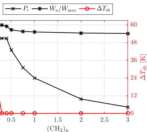
Fig. 7. The variation in the optimal reduced pressure P_r , the normalised power output \dot{W}_n/\dot{W}_{\text{max}} and the optimal amount of superheating \Delta T_{\text{sh}} as a function of the number of -\text{CH}_2- groups for the 1-alkene family and a heat-source temperature of T_{\text{hi}} = 150 °C.
