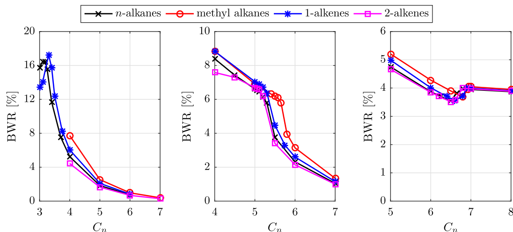
Fig. 17. The back-work ratio (BWR) as a function of the number of carbon atoms C_n obtained for each heat source temperature and hydrocarbon family; from left to right: T_{hi} = 150, 250 and 350\text{ °C} .
