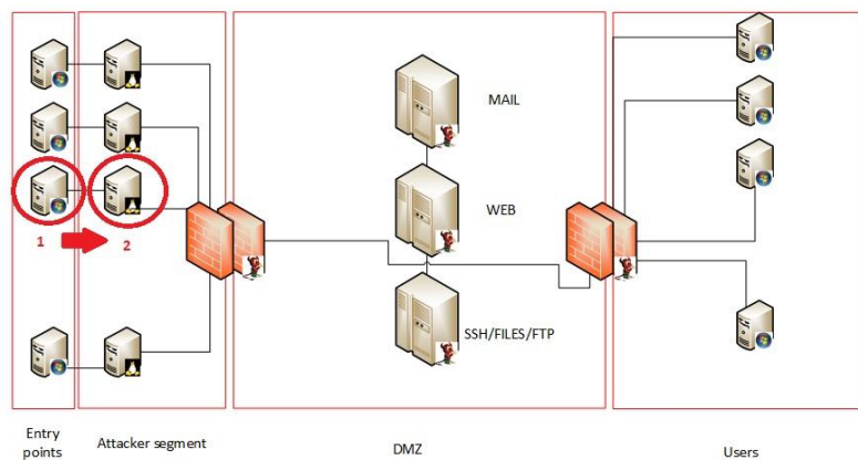
Figure 4.30 New vulnerability experiment infrastructure
