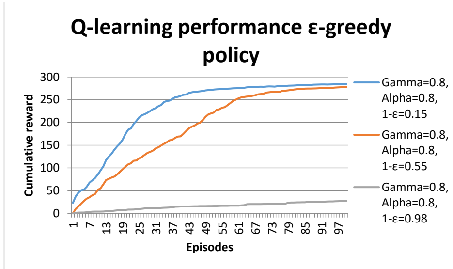
Figure 4.39 \epsilon -greedy Q-learning performance with Gamma=0.8, Alpha=0.8, 1- \epsilon =0.15/0.55/0.98
