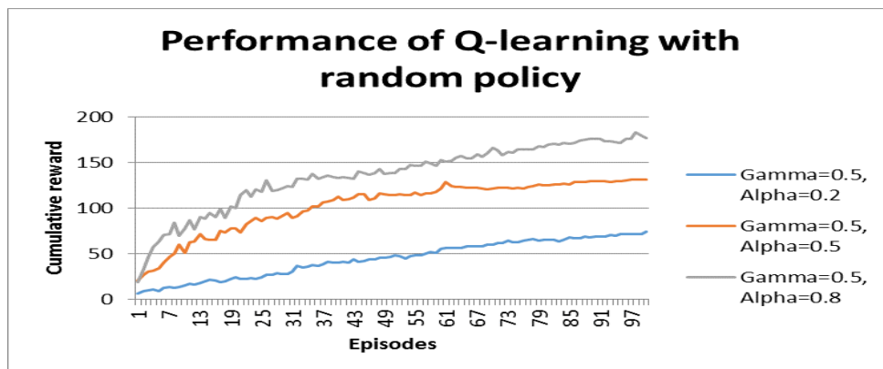
Figure 4.25 Performance of random policy Q-learning 100 episodes: \Gamma=0.5 , \alpha = 0.2/0.5/0.8
