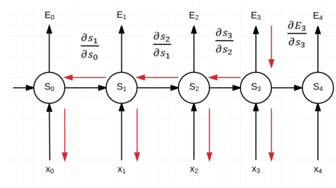
Figure 3.6 Gradient calculation for weight W
