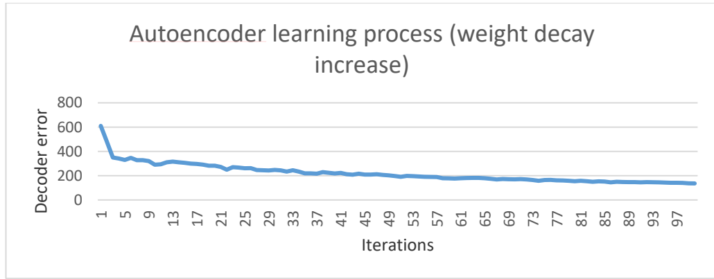
Figure 4.46 Autoencoder learning process ( \lambda_1 = 0.1 )
