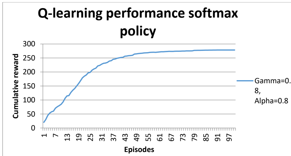
Figure 4.40 Softmax policy Q-learning performance with Gamma=0.8, Alpha=0.8
