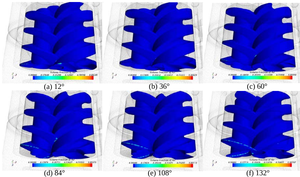
Figure 9 Cavitation distribution at 630rpm and 0.85MPa under different rotation angle
