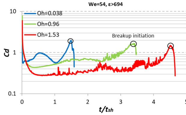
Figure 17. Temporal evolution of drag coefficient for cases 2, 14 and 15 (various Oh numbers).
