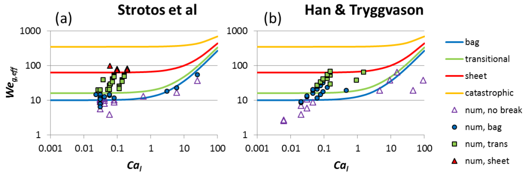
Fig.6: Results of the present model in the We_{g,eff} - Ca_I plane for (a) simulations of the authors' group and (b) simulations of (Han and Tryggvason, 2001).
