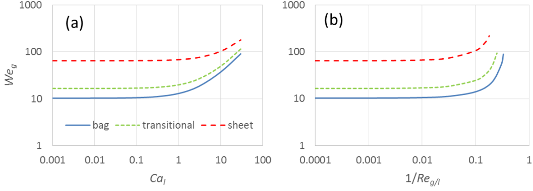
Fig.4: Results of the present model in (a) the We_g - Ca_l plane and (b) the We_g - 1/Re_{g/l} plane.
