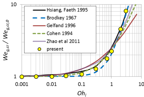
273 274 Fig.2: Results of the present model for the bag breakup regime in the We_g - Oh_l plane. 275 The corresponding results from other correlations are also shown.
