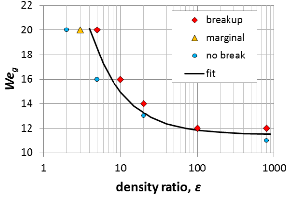
Fig.8: Effect of density ratio on droplet breakup for Ca_l=0.03 , Re=400 .
