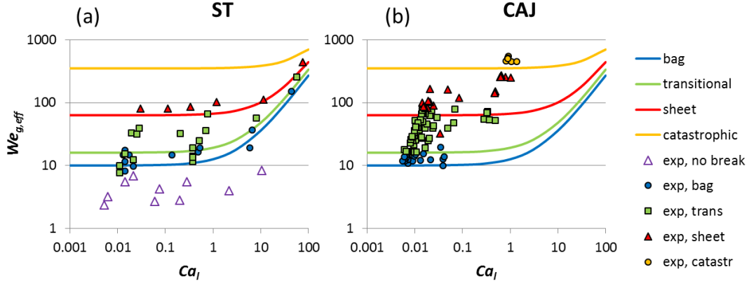
Fig.5: Results of the present model in the We_{g,eff} - Ca_l plane for (a) Shock Tube and (b) Continuous Air Jet experiments.
