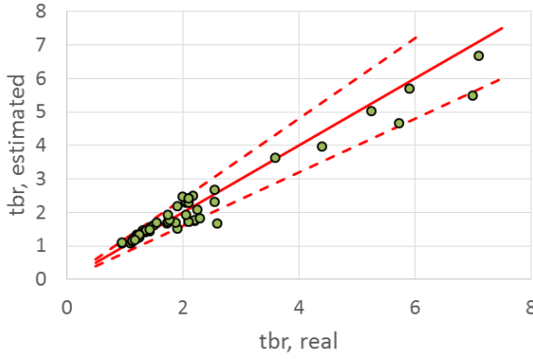
Fig.9: Prediction of breakup initiation time with eq. 28. The error lines of \pm 20\% are also shown.
