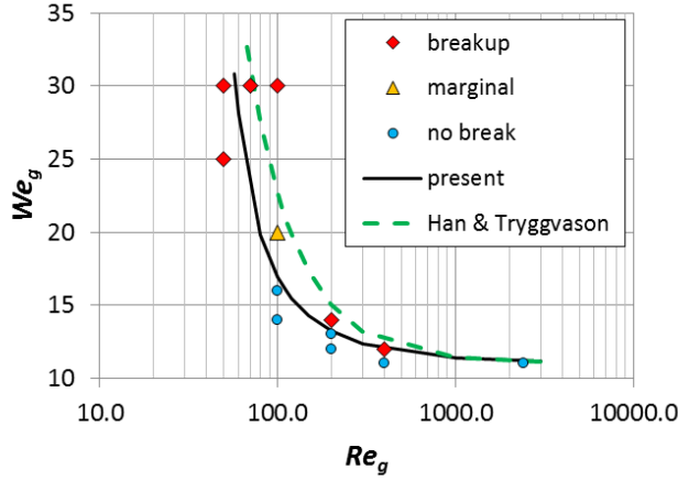
Fig.7: Effect of gas viscosity ( Re_g number) on droplet breakup for Ca_l=0.03 , \varepsilon=800 . A curve representing the corresponding results of (Han and Tryggvason, 2001) for \varepsilon=10 , is also shown.
