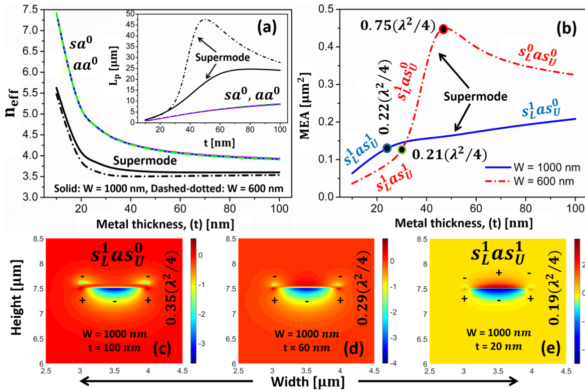
Fig. 8. SPP modal characteristics its evolutions with metal thickness ( t ) for a metal nanowire with a small index-difference ( n_{\text{substrate}} = 3.5 and n_{\text{superstrate}} = 3.3 ) in the cladding. The main and inset of (a) show the n_{eff} and L_p variations of long range supermode, sa^0 and aa^0 modes for fixed W = 1000 nm and 600 nm shown by the solid and dashed-dotted lines, respectively. The solid blue and dashed-dotted lines in (b) depict the modal effective area (MEA) of supermodes for W = 1000 and 600 nm, respectively. (c), (d) and (e) denote the H_x field evolution of the long range supermode for three different metal thickness, t = 100 , 60 and 20 nm, respectively. W is fixed at 1000 nm. The operating wavelength is kept fixed at 1550 nm.
