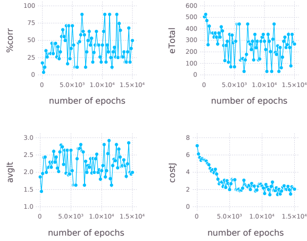
Figure 5: P1 training results under \mathcal{L} -interpretation
