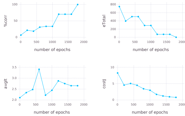
Figure 4: P1 training results under C*-interpretation
