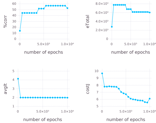
Figure 13: P4 training results under C*-interpretation
