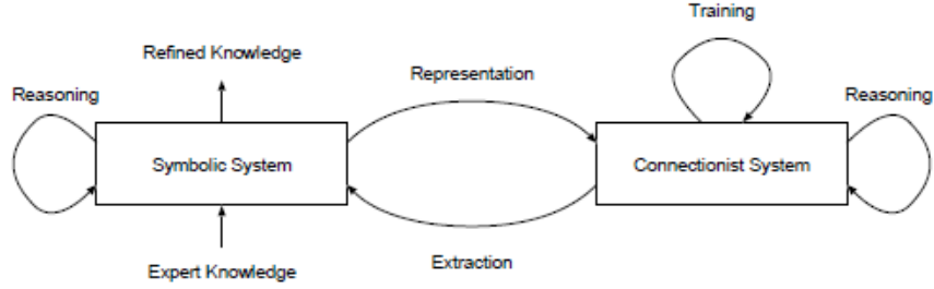
Figure 1: A conceptual overview of the neural-symbolic cycle (as introduced in [11]).
