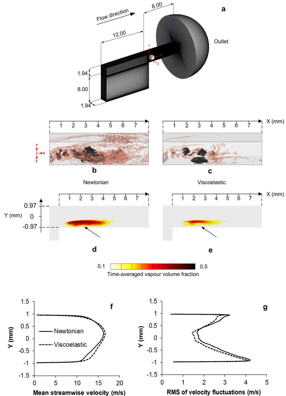
Figure 5. Computational domain and numerical results showing the effect of viscoelasticity on the nozzle flow and cavitation. (a) Computational domain, the blue rectangle indicates the flow visualization region, nozzle dimensions given in mm, (b,c) show the cavitation structures (dark colour) and vortex structures (translucent red color) in the nozzle for the Newtonian and the viscoelastic fluid, cavitation structures are presented by isosurface of 50% vapour volume fraction and vortex structures are presented by isosurface of second invariant of the velocity gradient at 2 \times 10^9 \text{ s}^{-2} , (d,e) time averaged vapour volume fraction in the mid-plane of the nozzle, cavitation suppression by viscoelasticity is particularly visible close to the nozzle wall where the cavity cloud is clearly detached from the wall, (f) time-averaged streamwise velocity at the nozzle exit, it is evident that the velocity is enhanced by the viscoelastic fluid, (g) RMS of velocity fluctuations at the nozzle exit, viscoelasticity can suppress turbulence and reduce the level of velocity fluctuations.
