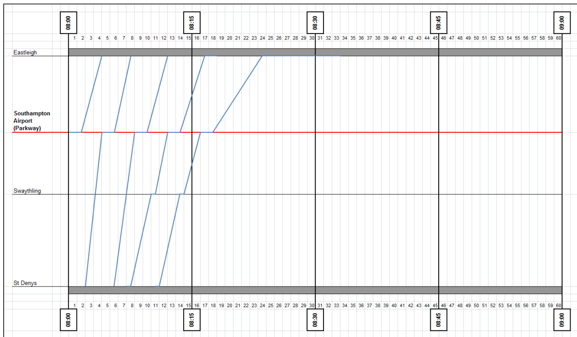
Figure 6: Compressed Timetable Graph for Southampton Airport (Parkway)
