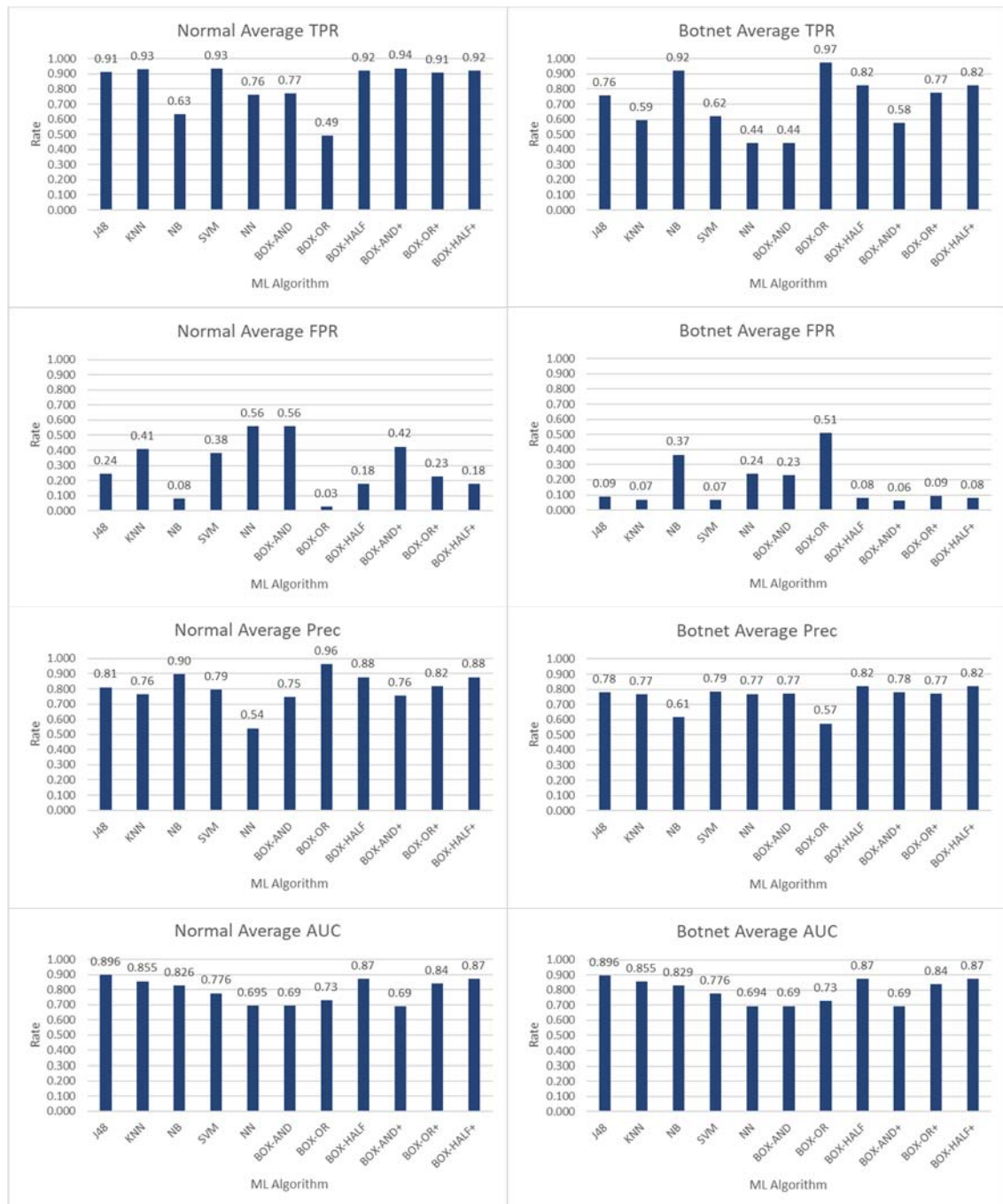
Figure 4-26 - Average performance of malware family dataset
