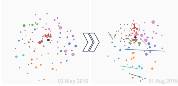
Figure 6: Rotation (B9): from May to August 2016, we see a great deal of movement in nodes' positions relative to each other, suggesting that the underlying correlation structure has changed substantially. Many financials stocks are closely bunched (B3; red dotted line), indicating strong correlations within that group.
