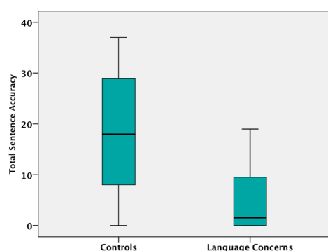
a) Boxplots
