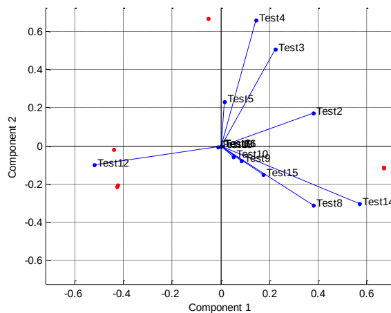
Figure 6.16: The WSs' Original Penetration Test Results against the First Two PCs
