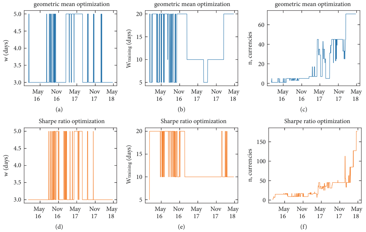
FIGURE 10: Method 2: parameters optimisation. The sliding window w (a, d), the training window W_{\text{training}} (b, e), and the number of currencies n (c, f) chosen over time under the geometric mean (a, b, c) and the Sharpe ratio optimisation (d, e, f). Analyses are performed considering prices in BTC.
