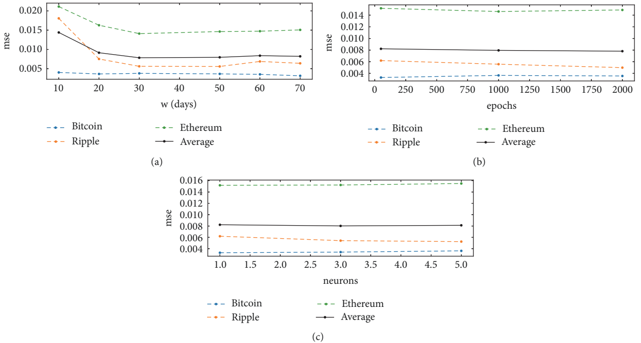
FIGURE 11: Method 3: parameters optimisation. The median squared error of the ROI as a function of the window size (a), the number of epochs (b), and the number of neurons (c). Results are shown considering prices in Bitcoin.
