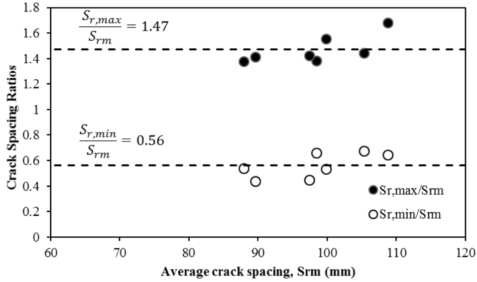
Fig. 17. Ratios of maximum and minimum to average crack spacing vs. average crack spacing in shear tests
