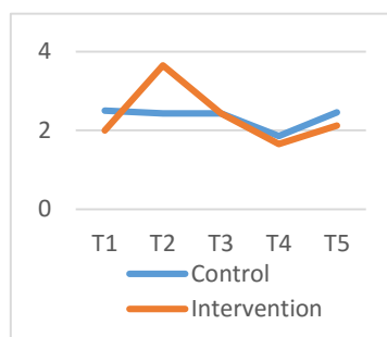
Graph 6: Total Illness Focused Strategies Used during Scenarios
