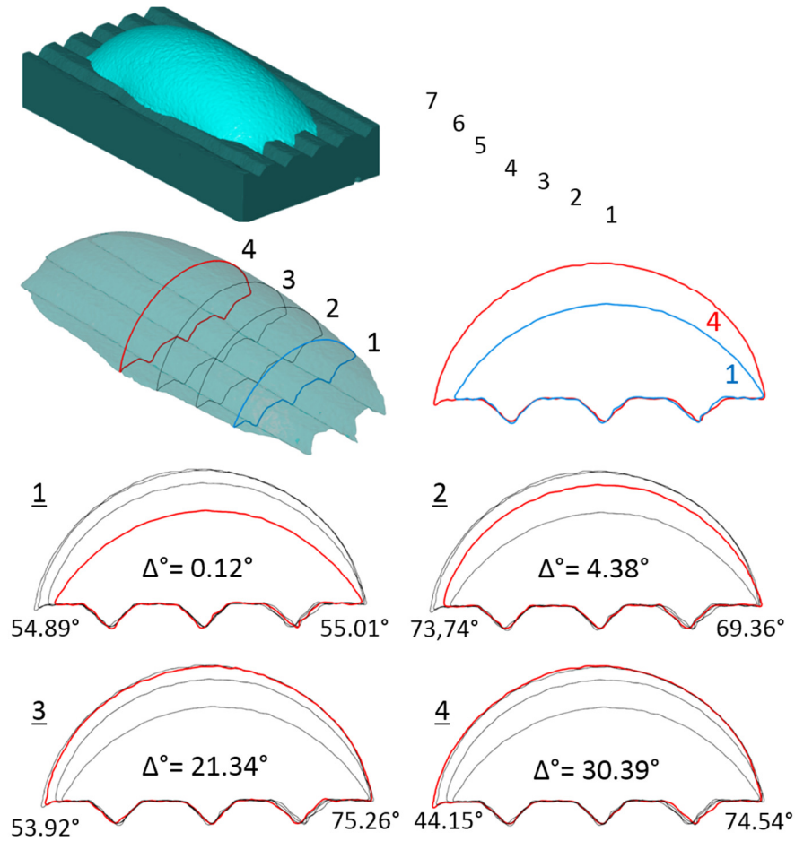
Figure 2-20 1 st row-left – drop and surface stl surfaces \frac{3}{4} view. 1 st row, right - only drop stl surface displayed in red with numbered sections (black lines) produced by planes perpendicular to the grooves. 2 nd row-left: semi-transparent drop visualization to reveal contours of drop surface sections 1 to 4. 2 nd row right – orthogonal view of section 1 (blue) and 4 (red) to reveal the pinning behaviour change: section 1 is characterized by strong left-right side symmetry, while section 4, corresponding to the central section of the drop, is highly non-symmetric since the left side of the drop oversteps the edge of the groove while the right side doesn't. 3 rd and 4 th row: orthogonal display of section 1 to 4 with indication of left-right drop contact angle with difference highlighting the non-symmetric behaviour of the drop-surface pinning
