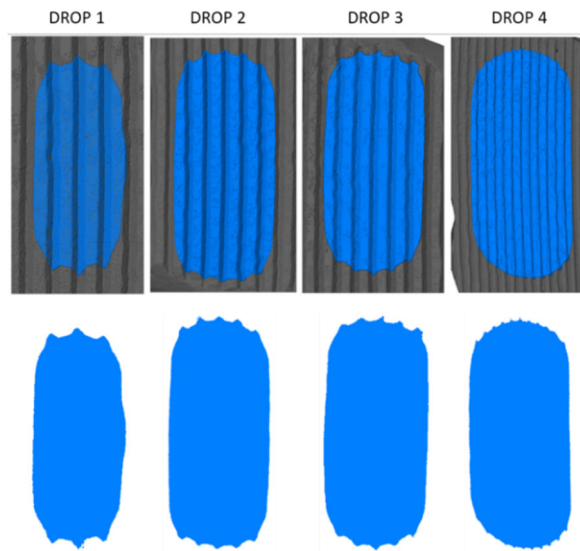
Figure 2-23 top row: 3D drops footprints on the record surface. Bottom row: 2D projection of the only drops footprints.
