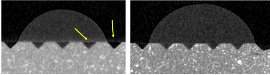
Figure 2-16 Left – section of drop reconstructed volume before application of radiation filtering: the two yellow arrows highlight the position of the artefact caused by the beam hardening showing in the section as a wide horizontal line of pixels with non-correct grey level values. The image has been smoothed to try to minimize via software the detected defect in the first instance. Right – section of a comparable drop reconstructed volume produced after the introduction of the aluminium filter, it can be noted that the beam hardening is diminished.
