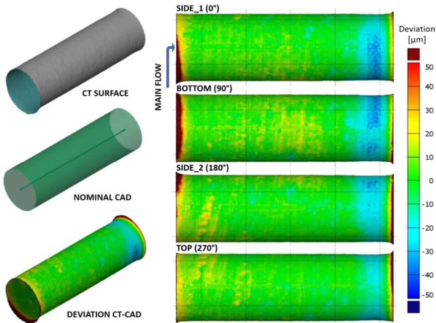
Figure 3-20 Left column from top to bottom – surface geometry of injection channel after running-in reconstructed with microCT; nominal injection channel cylinder; microCT geometry coloured to represent geometrical deviation of reconstructed surface from nominal cylindrical feature.
