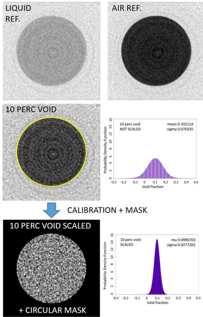
Figure 4-16 (top left) sample slice of liquid reference dataset. (top right) sample slice of air reference dataset. (middle -left) sample slice of 10 percent void dataset before calibration: the probability density function plot of the values inside the channel border, indicated in the image by a yellow circle, is visible on the right of the image. (bottom left) Same sample slice of 10 percent void dataset after calibration and only visual contrast enhancement.
