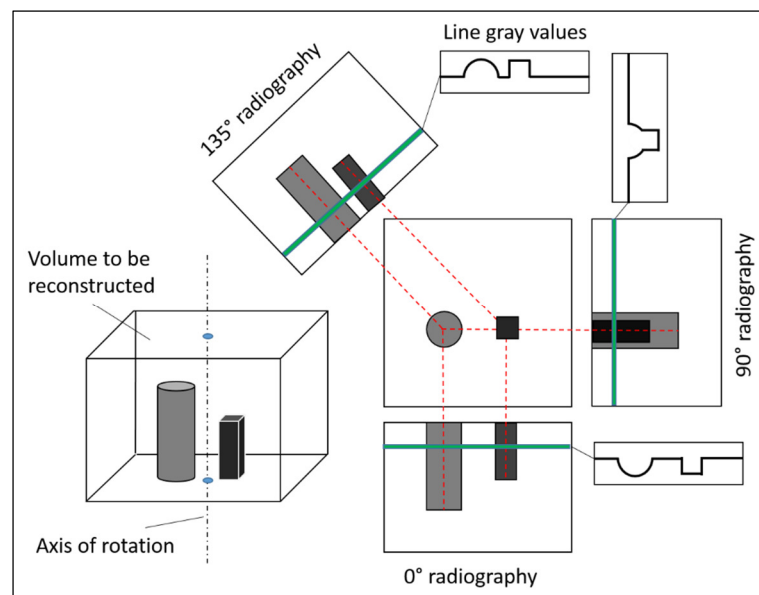
Figure 1-12 Illustration of the object shape and position guess through projections observation: the volume to be reconstructed shown in 3D on the left contains a cylinder and a rectangular cuboid: from the three projections shown on the right it is clearly impossible to guess the correct shape and position of the two objects even though each projection furnish partial data about the desired information.
