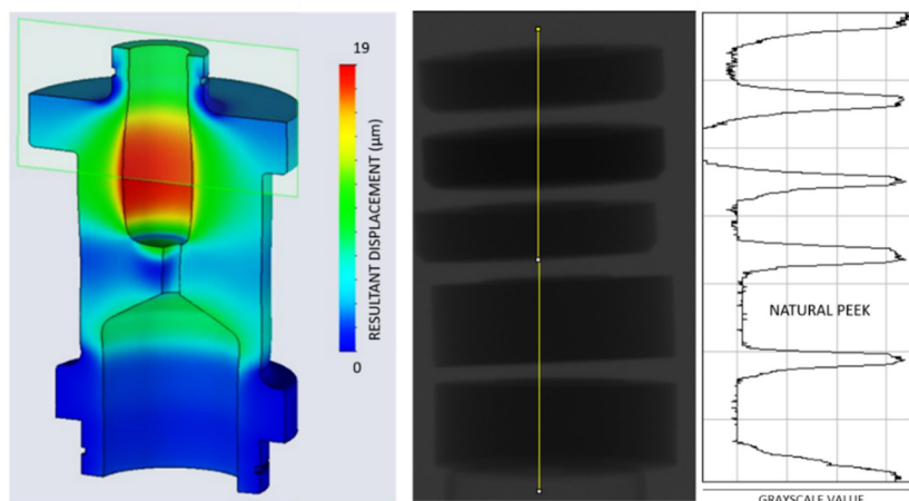
Figure 4-3 Left – Fem analysis of the PEEK test chamber model produced to assess geometrical deformation induced by maximum pressures (100 bar upstream the injection channel and 20 bar downstream). Centre – X-ray radiography of composite materials analysed for X-ray penetrability. Right – Grayscale values corresponding to the yellow line in the central image.
