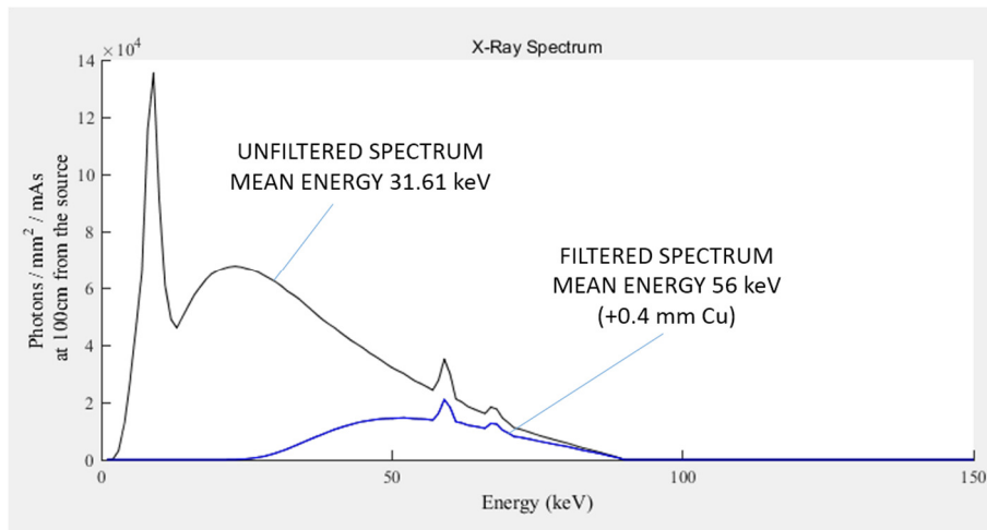
Figure 1-54 Unfiltered (grey line) versus filtered (blue) spectrum.
