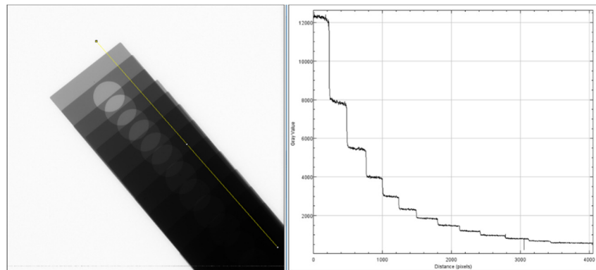
Figure 1-55 (left) radiography of the step wedge created with a tack of metal foil of 0.4 mm thickness and (right) grayscale values plot of the yellow line through its length.
