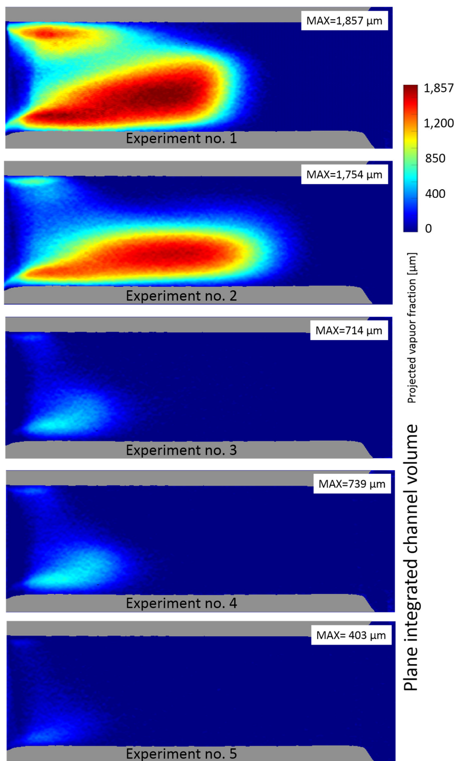
Figure 4-26 Plane integrated images calculated for all experiments
