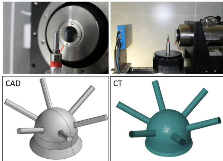
Figure 3-1 Top left: closeup view of injector nozzle placed inside the microCT machine ready to be scanned. The nozzle has been disassembled from the body and the needle has been removed to place the nozzle on top of the sample holder. Top right: complete view of injector nozzle inside the microCT machine. The nozzle distance from the X-ray source allows a magnification which produces a tomography with a 4 \mu\text{m} resolution.
