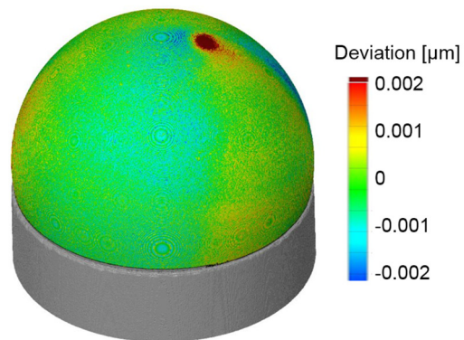
Figure 1-43 Deviation of sphere surface created with all available points to show pole artefact. As it can be seen the mesh deviation points that increase by three times the surface deviation from nominal spherical geometry are concentrated near the tomography rotation axis (dark brown in the figure).
