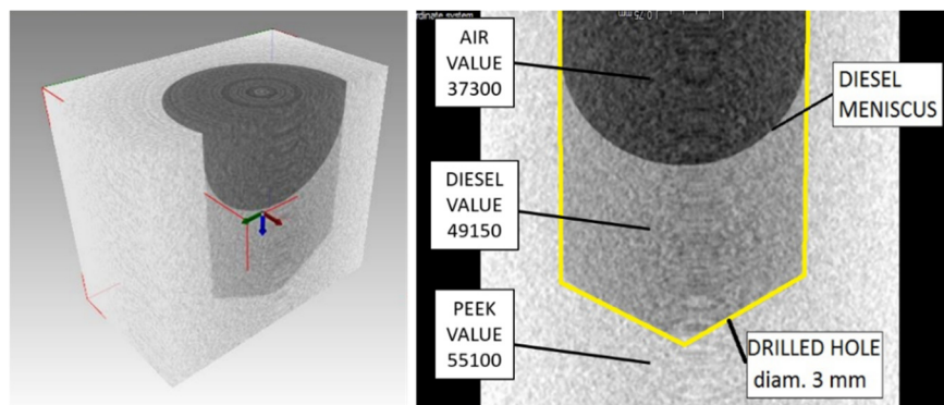
Figure 4-7 Left – 3D tomographic reconstruction of the central part of the sample, sectioned with a middle plane to reveal the inside. Here a drop of diesel is present. Right – orthogonal view of section presenting reconstructed values for air and diesel to assess the possibility to differentiate liquid diesel and diesel vapour, which was considered for simplicity of equal attenuation as air.
