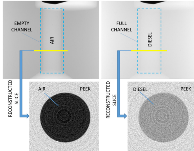
Figure 4-14 (top-left) projection of empty channel and (top-right) projection of channel full of Diesel. (Bottom-left) reconstructed slice of empty channel showing attenuation difference, by means of different grayscale values, between surrounding PEEK material and void channel. (Bottom-right) reconstructed slice of channel full of Diesel liquid.
