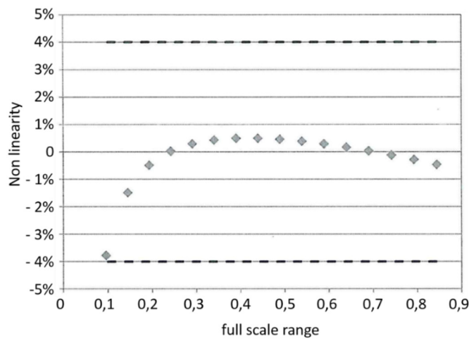
Figure 1-28 Linearity of the detector over its full range scale as communicated by the detector producer.
