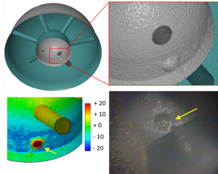
Figure 3-11 Top left – tilted bottom view of the reconstructed nozzle geometry with highlight of the position of the defect detected. Top right – zoomed view of the same geometry presented in the left to better reveal the defect. Bottom left – defect presented with deviation colouring exceeding used scale. Bottom right – picture of the defect produced after cutting the injector in half to reveal the inside.
