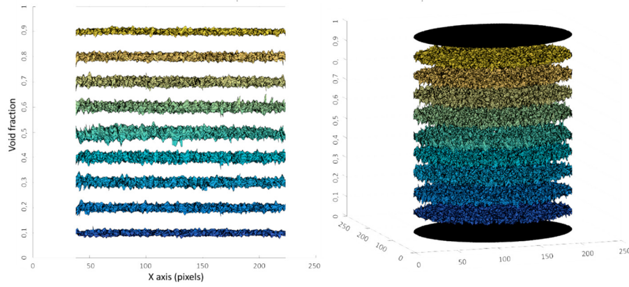
Figure 4-20 Visual representation of the created calibration scale: it can be noted that vapour fractions which are farther from the reference calibration dataset with 0 and 1 void fraction present more uncertainty.
