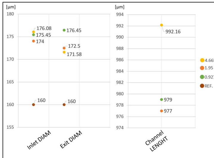
Figure 3-17 Left - Inlet and exit diameters (mean values) for the different tomographic resolution utilised. Bottom, right – mean channel length value for the three tomographic resolution
