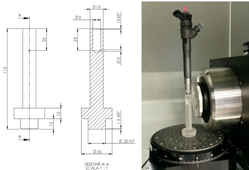
Figure 3-2 Left – CAD drawing of the top mounting sample holder. The only tolerance indicated is the h7 for the base diameter since this must tightly match the diameter of the hollow rotary stage central hole. The tolerance for the top hole where the nozzle sits is not indicated since the nozzle outside shape is conical.
