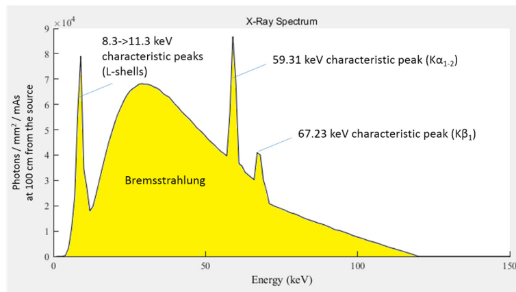
Figure 1-5 Tungsten (W) target spectrum simulated with Spektr software [40].
