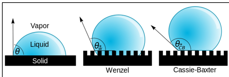
Figure 2-3 A droplet resting on a solid surface and surrounded by a gas forms a characteristic contact angle \theta . If the solid surface is rough, and the liquid is in intimate contact with the solid asperities, the droplet is in the Wenzel state. If the liquid rests on the tops of the asperities, it is in the Cassie-Baxter state. Image from [78]
