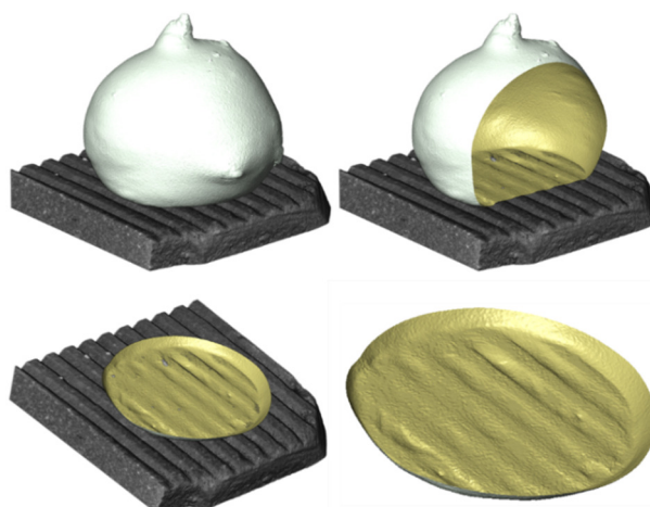
Figure 33 Top-left: 3D rendering of the drop of Hg based amalgam deposited on the patterned record surface. Top right: cut view of the amalgam surface to reveal its inside. Bottom-left: cut view parallel to the surface of the amalgam drop to reveal only its bottom part which interacts with the surface. Bottom-right: close up of the only bottom of the amalgam.
