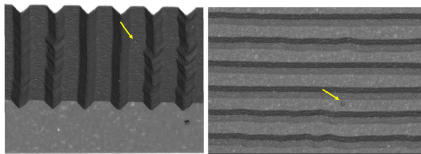
Figure 2-17 left – angled side view of the reconstructed vinyl record surface showing the grooves sides irregularities that produce music when hit by a turntable needle. The yellow arrow highlights the tomography rotation axis artefact. Right – top view of the same record surface.
