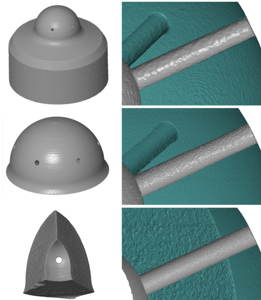
Figure 3-14 Left column – from top to bottom 3D renderings of the reconstructed volumes with three different reconstruction resolutions (4.665 \mu\text{m} , 1.950 \mu\text{m} , 0.927 \mu\text{m} ). Right column – from top to bottom cross cut view of the 3D rendering of reconstructed volumes visualizing one injection channel.
