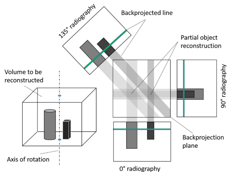
Figure 1-18 Back projection process: each projection line is back projected on the projection plane, which represents an horizontal cross section plane of the reconstructed volume, to reconstruct by summation the shape and material property value of the scanned object.
