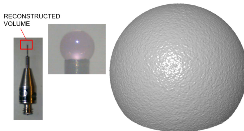
Figure 1-46 (left) overall and zoomed picture of 0.3 mm Renishaw stylus and (right) its rendered reconstruction from CT data.
