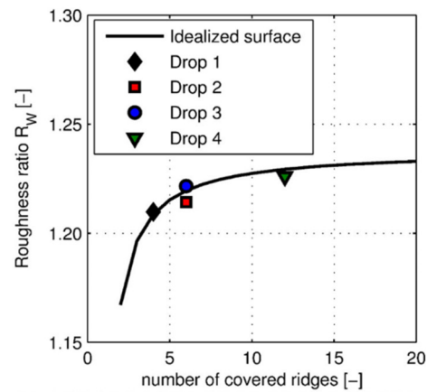
Figure 2-24 black line presents nominal surface Wenzel roughness ratio calculated utilizing the nominal geometry of the record surface, while the single points present the experimental results for the 4 drops of interest. It can be noted that the latter are in good agreement with the theoretical corresponding value. However, the experimental points referring to drop n.2 and n.3, which have very similar volume, are quite distant one from the other, this can be explained with the different way of covering the surface edges of the two drops, which is not represented by the single nominal value. Image from [85]
