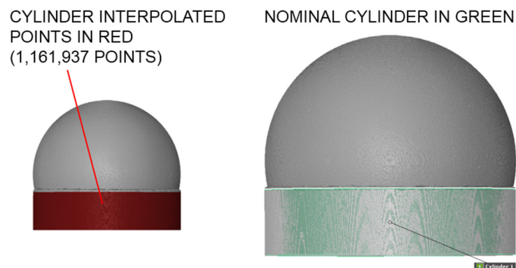
Figure 1-44 (left) in red STL surface cylinder points selected for the calculation of the fitting nominal cylinder. (right) in green nominal cylinder created from the selected points overlaid to the original STL surface shown in grey.
