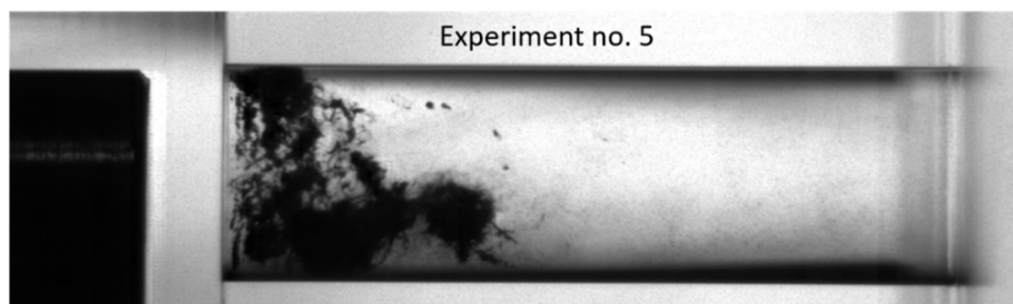
Figure 4-27 Single shot sample shadowgraphy pictures for all experiments
