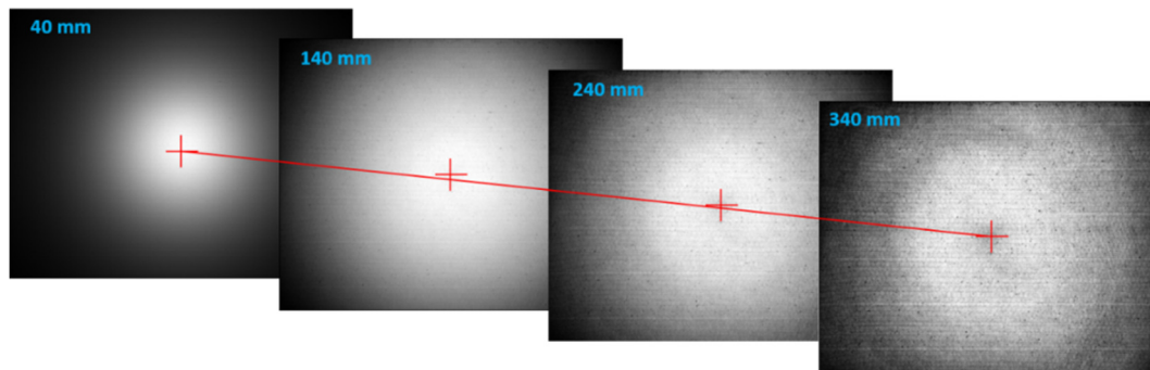
Figure 1-22 Emission axis alignment process: one radiography at each specific distance from the X-ray source is acquired and processed to obtain the emission centre as perceived by the detector. Based on this information the overall emission axis can be calculated and corrected moving the detector if not linear.
