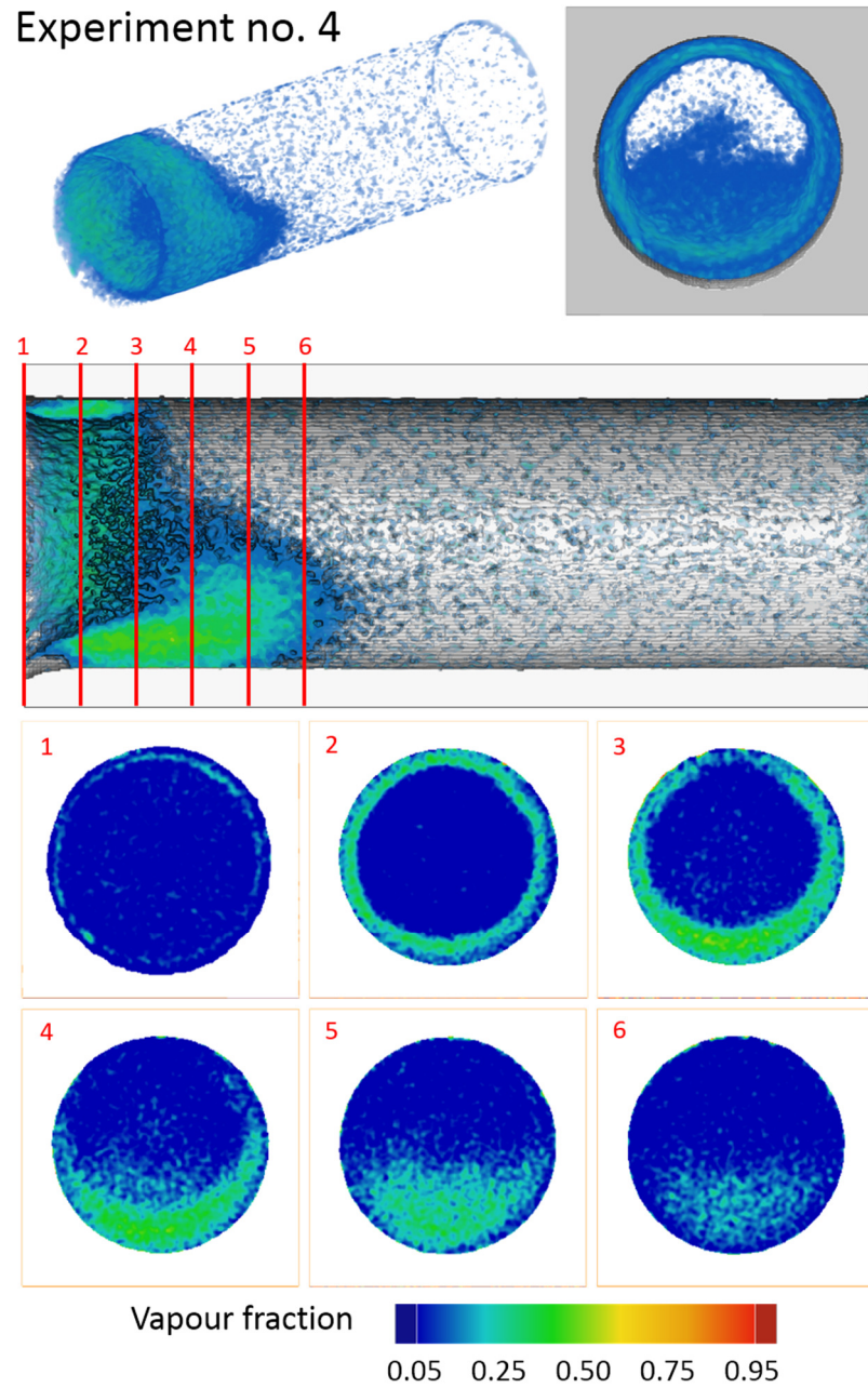
Figure 4-31 3D rendering, front channel view and axial sections for experiment no. 4
