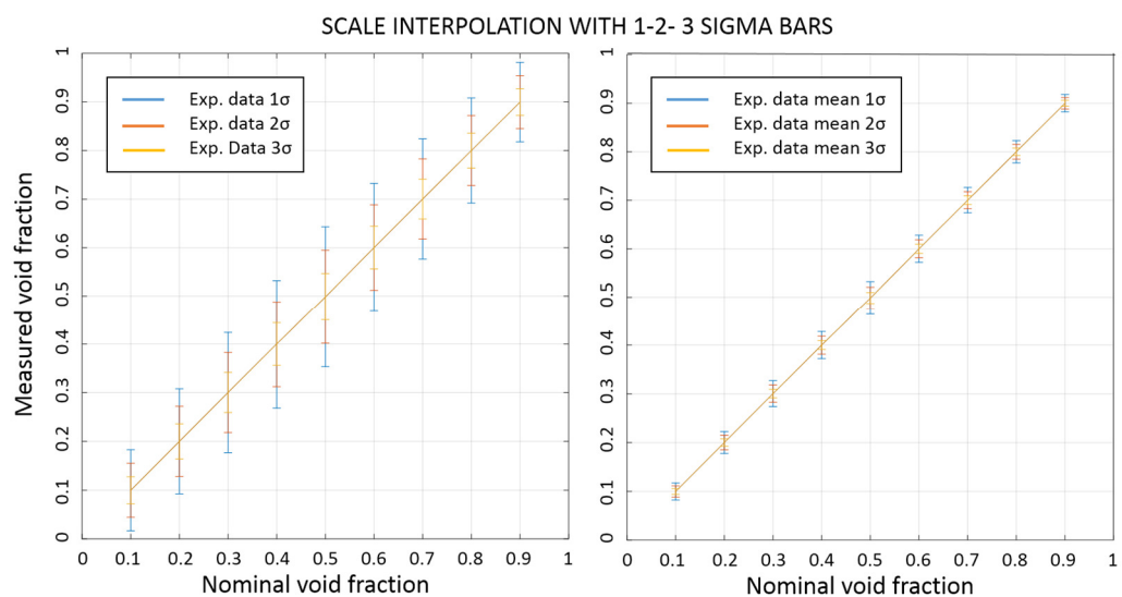
Figure 4-19 Void fraction calibration scale with 3-sigma bars
