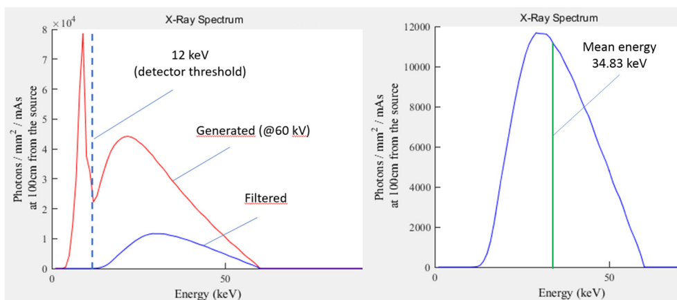
Figure 4-10 Left – Simulated X-ray spectra for an X-ray source voltage set of 60 kV, red line presents generated spectrum as exiting from the X-ray source while blue line presents same spectrum after filtration. Right – zoomed view of the filtered spectrum to better show its quasi Gaussian shape and resulting mean energy.
