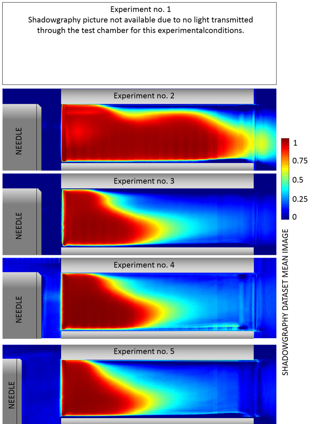
Figure 4-28 Calculated mean image for each experimental shadowgraphy dataset.
