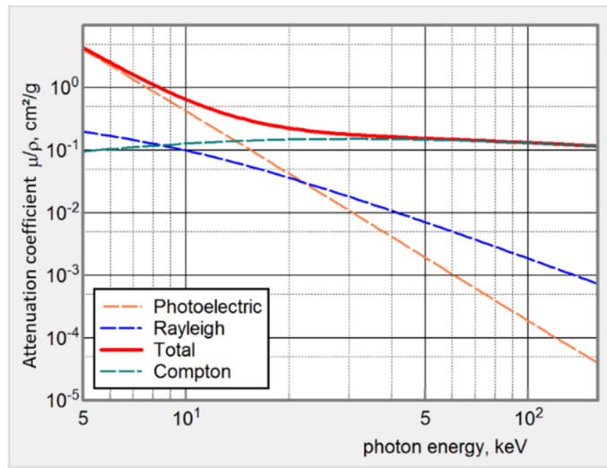
Figure 1-6 Contribution of each X-ray attenuation mechanism calculated for Beryllium and X-rays energies between 5 keV and 160 keV with software XMuDat [41] based on tabulated values of [42]
