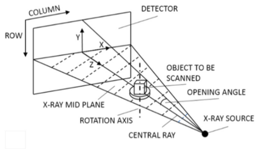
Figure 1-21 Coordinate system of the microCT machine.
