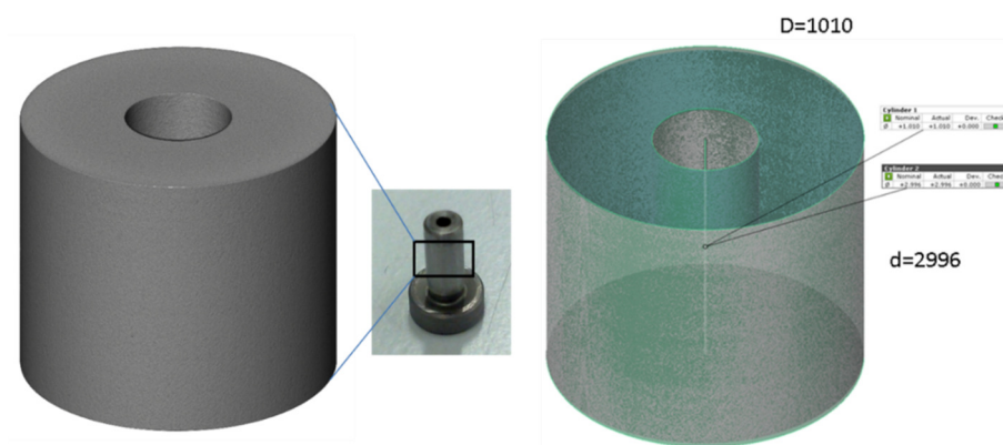
Figure 3-9 Left – 3D rendering of the DIN guide bushing sub-volume reconstructed by microCT. Middle – picture of the real part with reconstructed sub-volume identified by the black square. Right – stl reconstructed surface of inner and outer cylinders utilized for the diameter size calculations: “D” indicates the inner diameter while “d” indicates the outer diameter size.
