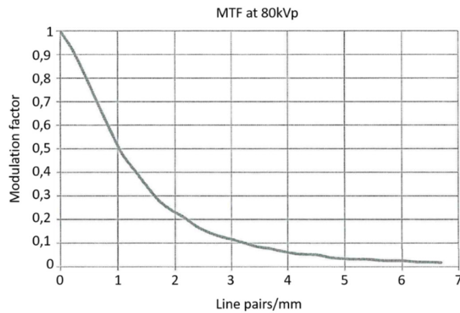
Figure 1-27 Modulation transfer function as communicated by the detector producer.
