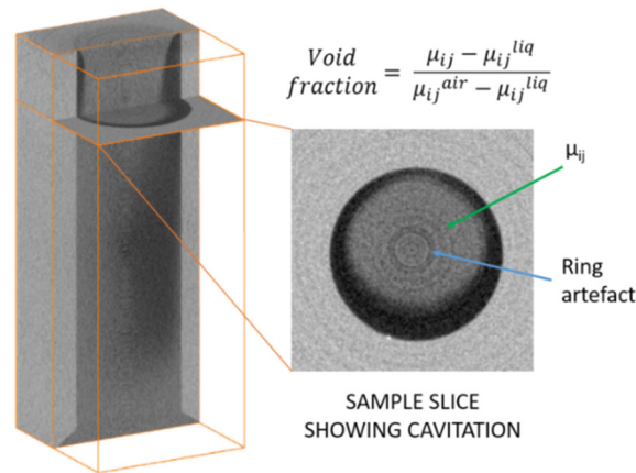
Figure 4-15 (left) axially cut 3D representation of the injection channel of interest with cavitation development (darker area) before application of values calibration and one non-cut slice perpendicular to the axis revealed. (right) Same slice of the reconstructed volume shown flat to reveal ring artefacts and shape of cavitation which is also circular in shape.
