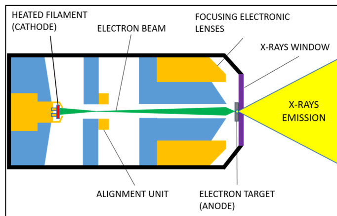
Figure 1-2 Schematic section view of a transmission target X-ray source. From left to right we can find the filament cathode (in red), the produced beam of electrons (in green), the alignment unit and focusing electronic lenses (in orange), the electron target (in grey), the output window (in purple) and the emitted X-ray beam (in yellow).
