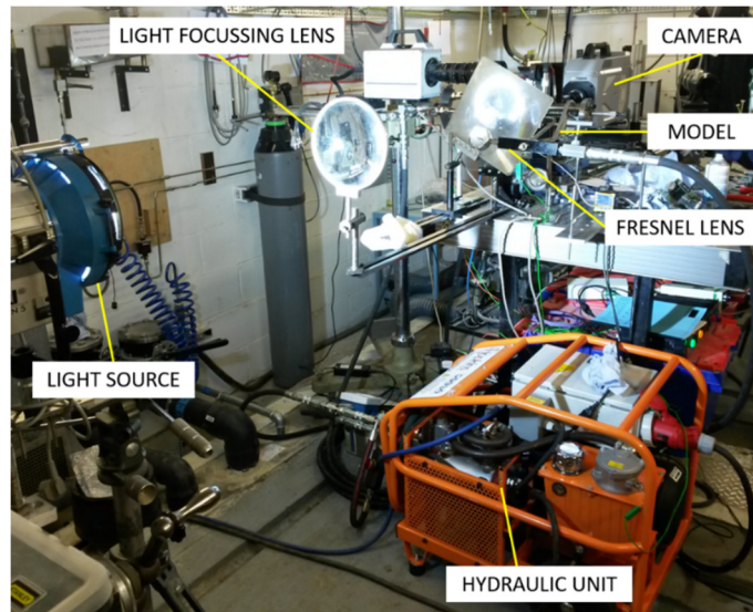
Figure 4-12 Shadowgraphy set-up presenting the components mentioned in the text: light source, focussing lenses, test chamber model and high-speed camera.
