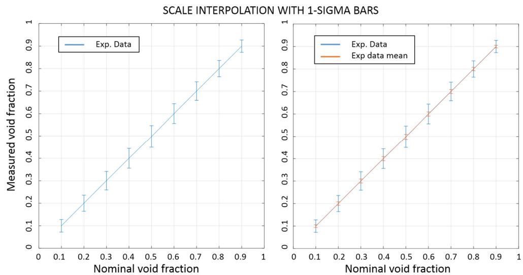
Figure 4-18 Void fraction calibration scale with 1-sigma bars
