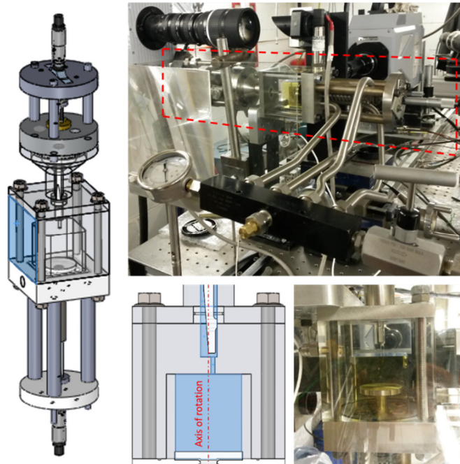
Figure 4-1 Left – 3D CAD image of the test rig as available for the high-speed visualizations. Right, top – Picture of the same rig assembled and utilized: the area surrounded by the red dashed line highlights the rig horizontally mounted on the optical table. Right, bottom – close up CAD and picture of the test chamber, the CAD image presents the hypothetical rotation axis mentioned.
