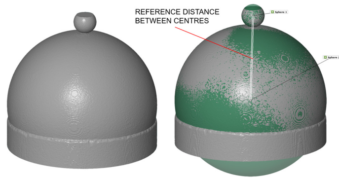
Figure 1-51 (left) stl surface of the two styli reconstructed from the single CT dataset. (right) in green 3-sigma fitting spheres utilized to calculate the distance between the centres, the line connecting the two centres is highlighted as “reference distance”.
