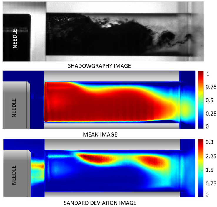
Figure 4-21 Top: high speed shadowgraphy picture of experimental conditions of experiment no.2. Middle: and bottom: Calculated mean and standard deviation images.
