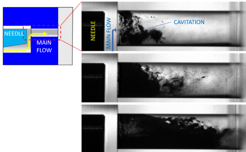
Figure 4-13 Left- schematic view of test injection channel. Right – from top to bottom three shadowgraphy images are obtained with same needle lift equal to 1 mm in different conditions.
