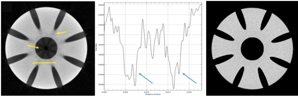
Figure 1-53 (left) axially perpendicular slice of a Diesel injector tip reconstructed with microCT showing streaks artefacts produced by injection holes, yellow arrows highlight modification of calculated attenuation value which is visible for areas inside the injector material and outside (air). (centre) plot of greyscale values indicated by the line in the left image, blue arrows show lower attenuation due to beam hardening streaks. (right) same slice after beam hardening correction application,
