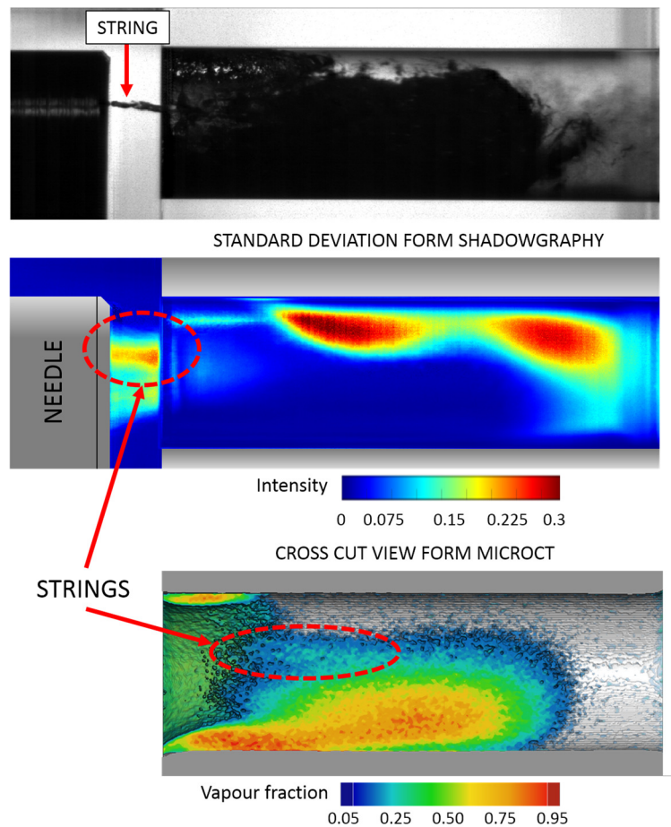
Figure 4-24 Top: shadowgraphy picture revealing the string like vortex between the needle tip and the channel entrance. Middle: standard deviation image revealing the localization of the string like vortices. Bottom: cross cut view of microCT reconstructed volume presenting cavitation structures which may be connected to the presence of string like vortices detected by the shadowgraphy images. All images refer to experiment no. 2.
