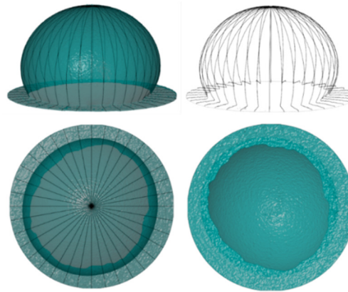
Figure 2-11 top left – stl drop surface visualized in green with radial sections shown in black. top right – visualization of only the radial sections contours (36 of the 120 used). Bottom left and right – top and bottom view of the drop-surface stl clearly showing the non-circular footprint of the drop.
