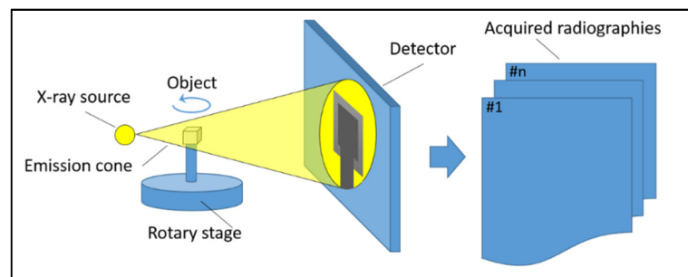
Figure 1-11 Layout of sample tomographic acquisition. From left to right we have the X-ray source, represented with a pointwise emission, the rotary stage with the cubic object to be scanned positioned on a sustaining cylindrical sample holder, the detector where the transmitted radiation is acquired and sampled to be saved in a 2D image file, the stack of acquired radiographies, one for each positional step, ready to be processed for reconstruction
