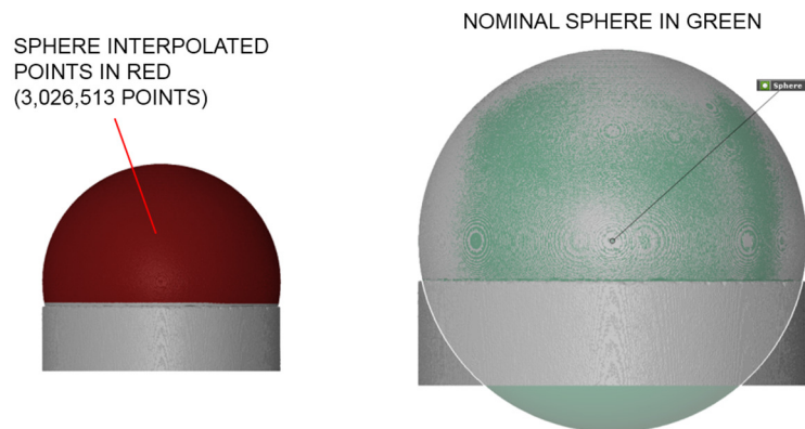
Figure 1-40 (left) in red reconstructed stl surface points selected for the fitting operation. (right) in green nominal fitted sphere overlaid to the original reconstructed stl surface shown in grey.
