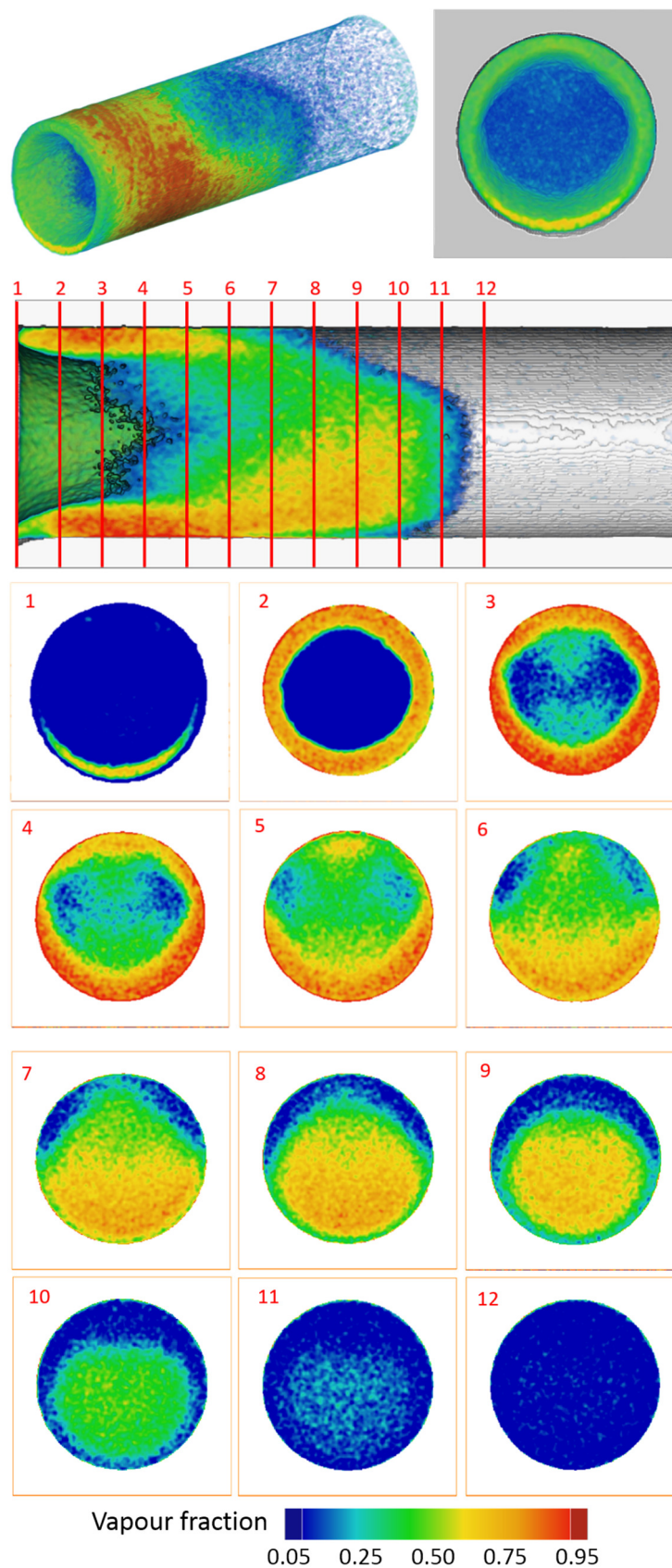
Figure 4-26 (1 of 2) Top: cross cut view of the MicroCT injection channel reconstructed volume presenting a red line every 600 \mu\text{m} . Following numbered images: sections perpendicular to the channel axis produced in the positions located by the previously mentioned red lines. All images refer to experiment no.2.
