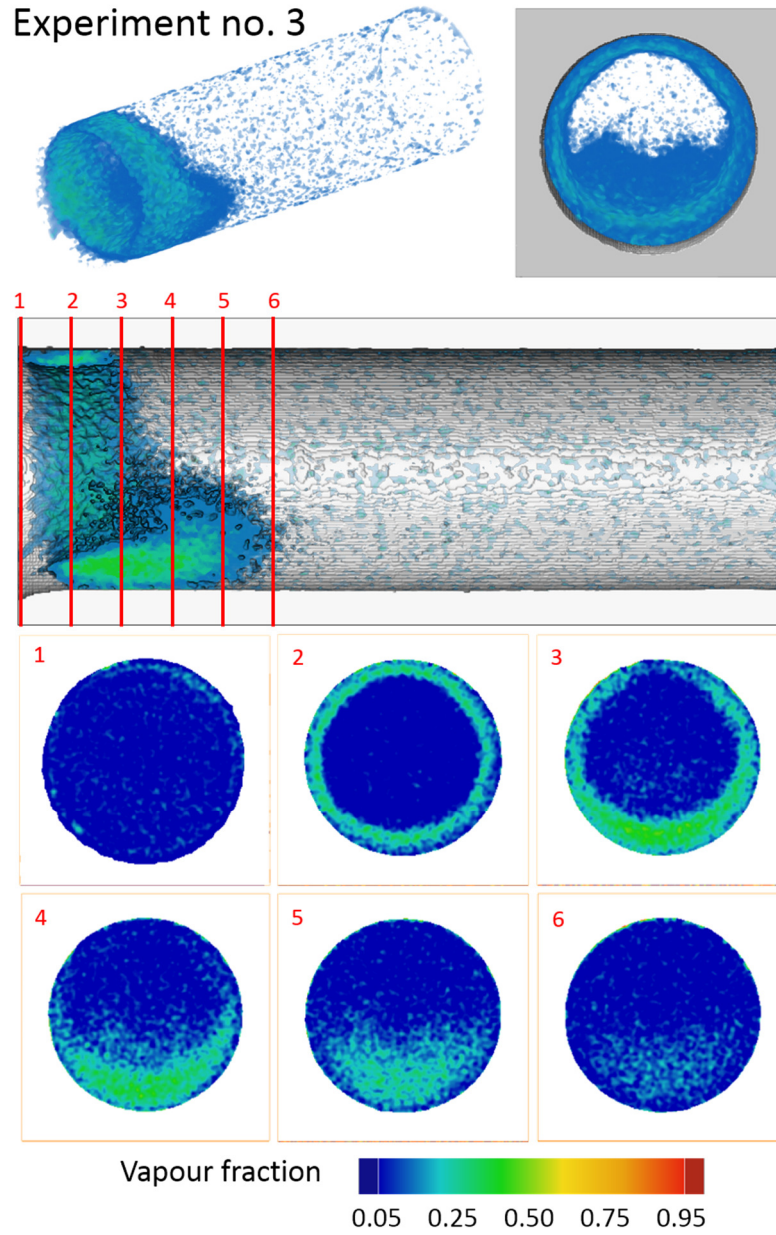
Figure 4-30 3D rendering, front channel view and axial sections for experiment no. 3
