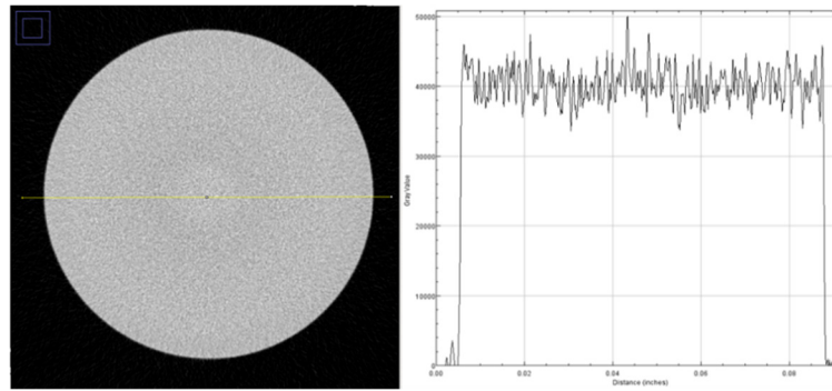
Figure 1-58 (left) same axially perpendicular slice of the sample metal cylinder showing beam artefact correction result. (right) plot of greyscale values vs diameter position of the yellow line over imposed to the cylinder section present in the left image revealing grey values homogeneity improvement due to applied correction.
