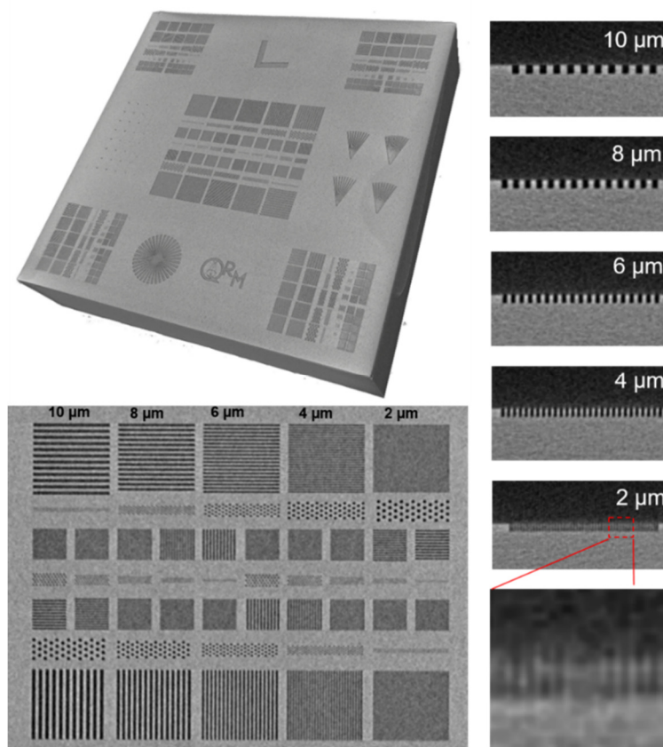
Figure 1-33 (top-left) 3D rendering of the reconstructed volume of the vertical chip of the QRM phantom. (bottom-left) Zoom of the central area of the phantom where it is clearly visible the possibility to distinguish lines of 4 \mu\text{m} with the nominal tomography resolution set at 2.19 \mu\text{m} . (right) from top to bottom cross cut of the 10-8-6-4-2 \mu\text{m} lines to show engraved lines distinguishability down to 4 \mu\text{m} , while the 2 \mu\text{m} apart lines are not clearly identifiable.
