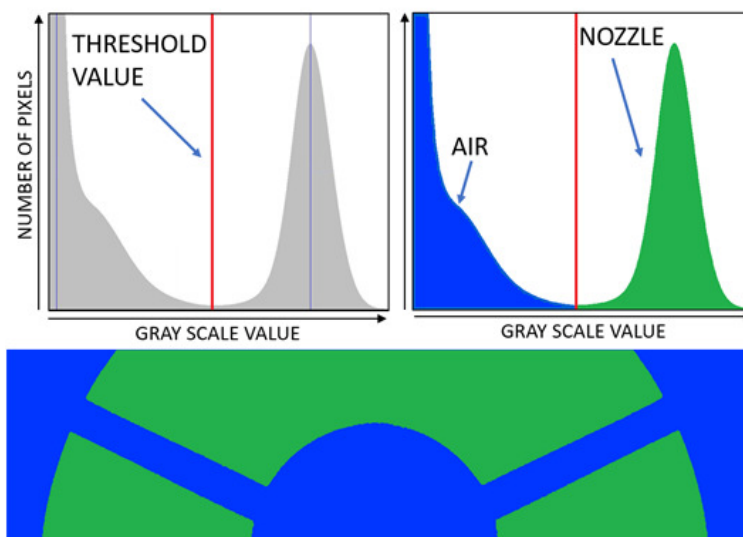
Figure 3-6 Top, left – histogram of the nozzle tomography showing selected threshold value corresponding to the min histogram value between material peaks. Top, right – same histogram presented in the left image but with air and nozzle histogram values assigned colour coded. Bottom – nozzle slice colour coded using threshold value.
