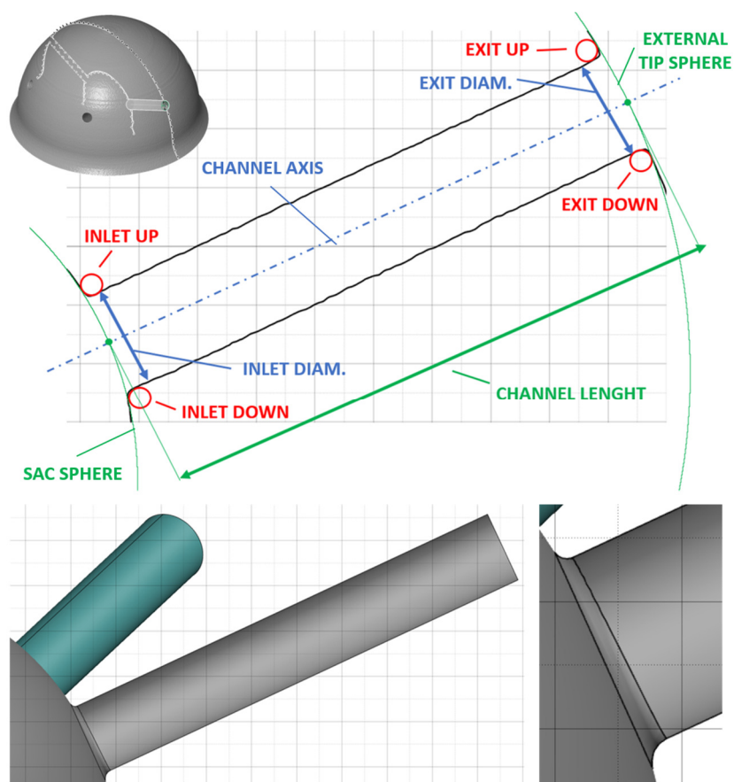
Figure 3-15 Top left – 3D rendering of nozzle tip with geometry section visualized. Top right – orthogonal view of channel cross section with numbers indicating the measured dimensions. Bottom left – cross cut view of the nominal CAD geometry. Bottom right – close up of inlet rounding of the nominal CAD channel geometry.
