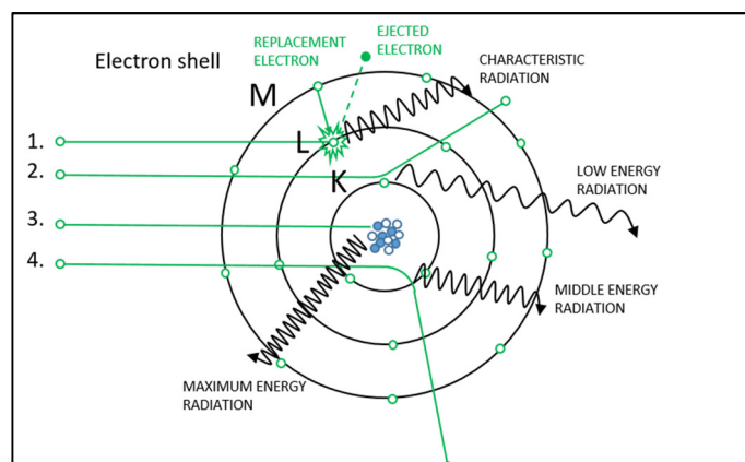
Figure 1-3 Visualization of the production of X-rays through the interaction of electrons with target atoms. Electrons numbered 1 to 4 hit the target from left producing X-rays of energy proportional to the intensity of their interaction with the nucleus and its electrons. Image inspired by an illustration present in [37].
