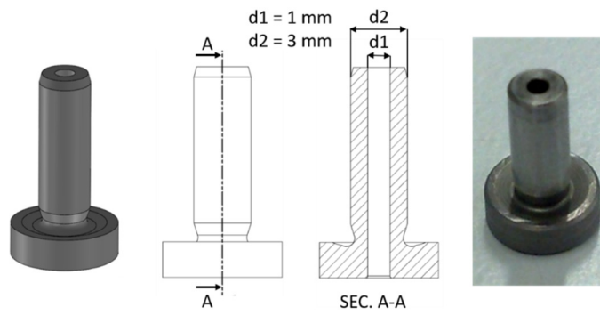
Figure 3-7 3D rendering, drawing and picture of DIN bushing utilised for the dimensional checks.
