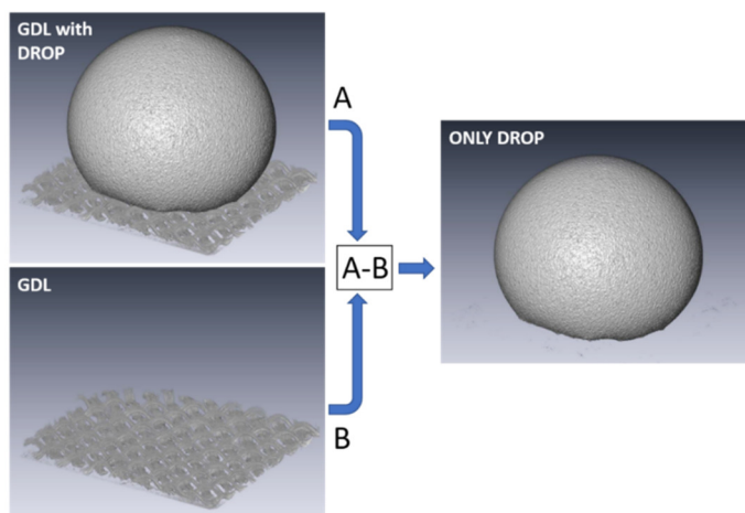
Figure 2-28 Left - rendering of the tomographic results of GDL with DROP (top) and only GDL (bottom) Right – result of the subtraction showing drop volume remaining.
