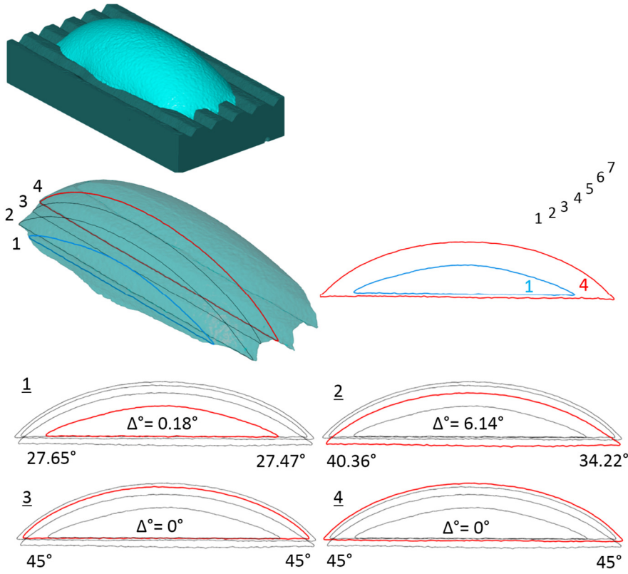
Figure 2-21 1 st row left: drop and surface stl surfaces ¾ view. 1 st row right: only drop stl surface displayed in red with numbered sections (black lines) produced by planes parallel to the grooves. 2 nd row-left: semi-transparent drop visualization to reveal contours of drop surface sections 1 to 4. 2 nd row right – orthogonal view of section 1 (blue) and 4 (red) to reveal the symmetry in the pinning behaviour. 3 rd and 4 th row: orthogonal display of section 1 to 4 with indication of left-right drop contact angle with difference highlighting the symmetric behaviour of the drop-surface pinning.
