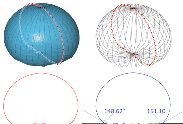
Figure 2-31 Top-left: in blue 3D rendering of the drop surface with radial sections overlapped in black and red, 18 items in total, one section each 10°. Top-right – visualization of the only drop profiles to reveal the complexity of drop surface footprint. Bottom-left: orthogonal view of red single drop profile present in the previous images. Bottom-right: B-spline drop contour profiling and contact angle measurement of red drop profile presented in the previous images.
