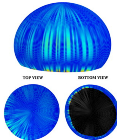
Figure 2-12 Reprinted with permissions from [79]. 3D rendering of the fitted profiles coloured to represent experimental-fitted profiles deviation. Colour from blue (0%) to red (3.85%) is proportional to the dimensionless error \Delta R/R_{max}
