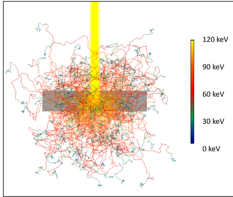
Figure 1-4 Image of the electrons travelling inside the target material produced with software “CASINO” [39].
