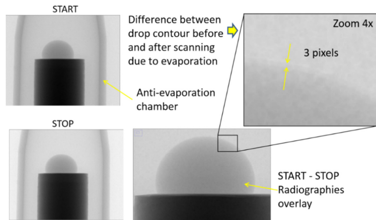
Figure 2-8 a) superposition of reference drop radiographies (before and after tomographic acquisition in the same position). b) zoomed view of the drop contours showing the still present evaporation effect.
