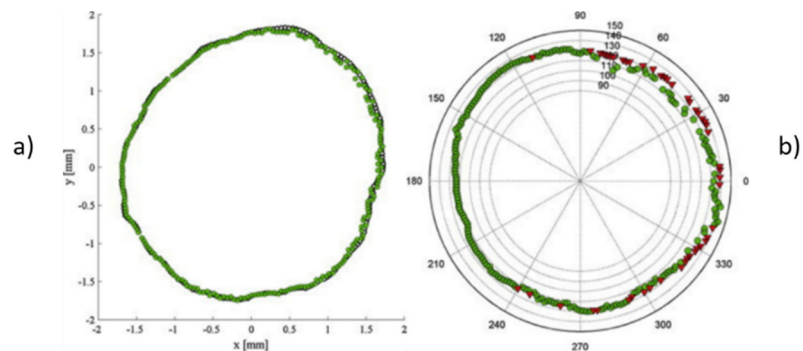
Figure 2-13 a) – b) Reprinted with permissions from [79]. Graphical visualizations of the triple line trajectory and contact angle measurement comparison between experimental and fitted datasets. a) xy plane localized comparison of drop-surface points: green circles represent experimental points while black circles represent fitted data, the maximum distance between analogous points is 72 \mu\text{m} b) contact angle measurements: green dots represent positions where experimental and fitted contact angle measurements are in good agreement, 192 points of the original 240, while red triangles represent point with bad agreement.
