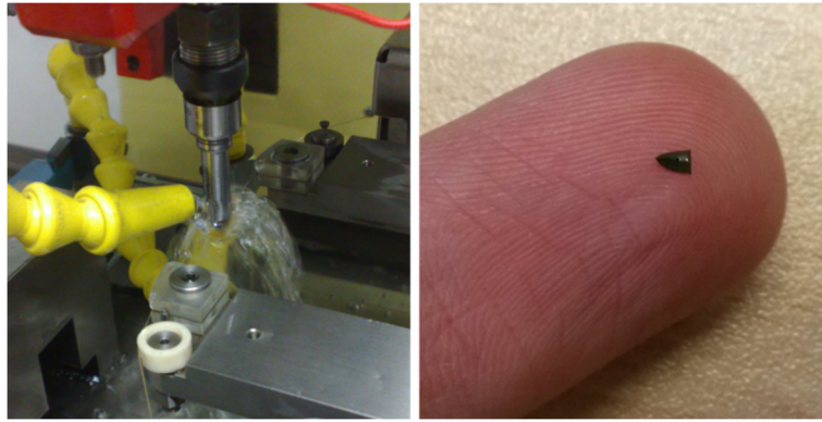
Figure 3-13 Left – 60-degree sector cutting operation inside microEDM machine, the nozzle is being cut by the metal wire which constitutes the eroding electrode; the actual erosion point is visible on the tip of the nozzle as a blue point representing the electrode spark position. Right – 60-degree nozzle tip sector after erosion placed on a fingertip.
