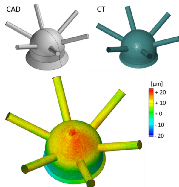
Figure 3-10 Top left – nominal CAD design geometry for the internal volume of the studied nozzle. Top right – reconstructed geometry produced by microCT data. Bottom – over position of CAD and CT geometries with the CT surface colour coded to reflect surface to surface distance.
