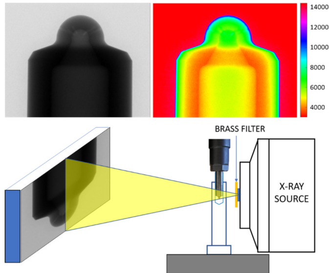
Figure 3-3 Top left – radiography of the nozzle produced with the reported settings. Top right – false coloured radiographic image showing in false colours the intensity of the radiation received by the X-ray detector. Bottom row – schematic view of the tomography set-up to identify the position of the metal filter utilized to filter the incoming radiation.
