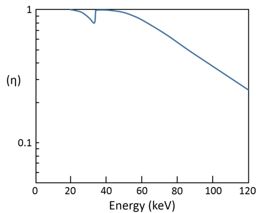
Figure 1-9 Conversion probability of Caesium iodide phosphor doped with Thallium based on incoming X-ray energies from 0 to 120 keV. Source: redrawn from [43].
