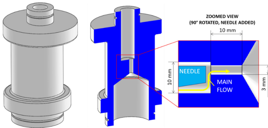
Figure 3-19 Left – external view of 3D CAD model. Centre – section view of CAD model showing internal injection channel position and geometry. Right – zoomed orthogonal view of only injection channel with needle added visualizing flow path and asymmetric needle utilised.
