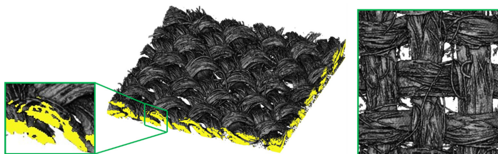
Figure 2-26 Top – 3/4 view of the GDL reconstructed volume, yellow section at sides represents recognized fibre volume: as it can be seen, inside strands, single carbon fibres are merged in one bigger volume. Bottom – higher zoom top view of a small portion of the GDL to further highlight the visibility of some of the carbon fibres protruding from the strands.
