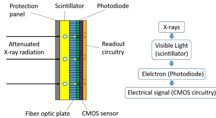
Figure 1-8 X-ray CMOS detector simplified layout. From left to right: incoming X-ray radiation, protection plate (grey), scintillator layer (yellow), fibre optic plate (blue), photodiode (green), CMOS sensor (purple) and electronic readout circuitry (orange).
