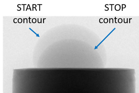
Figure 2-9 Overlay of drop radiography before and after tomographic scan without anti-evaporation cap.
