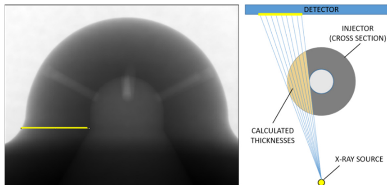
Figure 1-56 (left) radiography of Diesel injector tip without needle with yellow line over imposed to the area utilized for the calculation of the self-wedge map. (right) Illustration of the thicknesses calculation for the object of interest.
