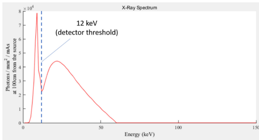
Figure 4-9 Simulated plot generated with Spektr presenting the X-ray spectrum produced by an X-ray source voltage of 60 kV. The absence of the higher Tungsten characteristic peaks is evident, while the lower energies peaks are filtered out by the detector lower energy detection threshold.
