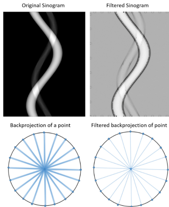
Figure 1-17 Left: unfiltered sinogram (top) and simplified back projection of a point (bottom) showing the image blurring that would results by the back-projection process if the images weren't high-pass filtered. Right: same sinogram image ramp filtered to enhance high frequencies (top) and same back projection of a point with filtered sinogram. It is clear the necessity of the filter enhancing high frequencies.
