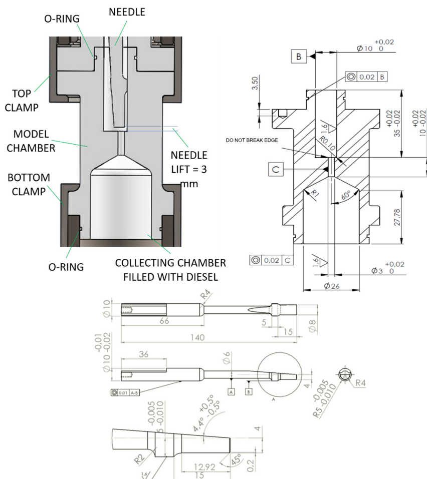
Figure 4-4 Top-left – Section of 3D CAD model showing inner injection channel geometry, sealing O-rings and fixing clamps position. Top-right: 2D CAD drawing of the sample model presenting a section of it showing its design dimensions. Bottom – 2D CAD drawing of the non-symmetric needle.
