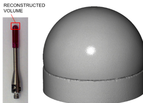
Figure 1-39 (left) picture of 2 mm Renishaw stylus with (right) its rendered reconstruction form CT data.
