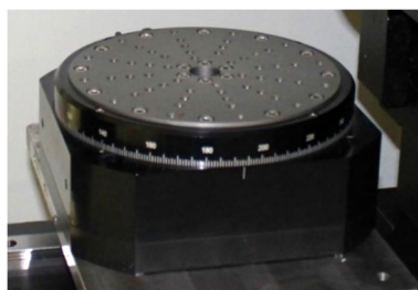
Figure 1-25 Air bearing rotary stage produced by Aerotech utilized to rotate the sample during radiographies acquisitions.
