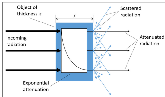
Figure 1-7 Representation of the interaction between an incoming monochromatic X-ray radiation and a homogenous object material.
