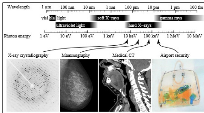
Figure 1-1 (Top) localization of X-ray wavelengths and energies, distinguished as soft and hard X-rays, in the electromagnetic spectrum; (Bottom - from left to right) application of X-rays to determine the arrangement of atoms in the crystalline solids, breast cancer screening radiography, head and neck computed tomography scan, airport security baggage scanning for safety reasons. [38]
