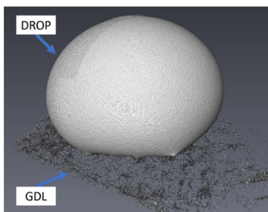
Figure 2-27 Grayscale rendering of thresholding window utilized to determine the only drop volume. It is clearly visible that under the drop, the GDL volume is partially visualized meaning that it will be recognized as drop volume after thresholding operation.
