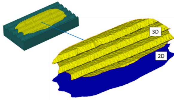
Figure 2-22 Visualization of 3D drop base area extraction (yellow) and its projection on surface parallel plane to calculate the 2D footprint of the drop.
