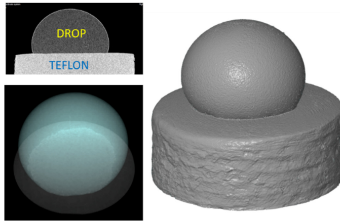
Figure 2-10 Top-left – reconstructed volume section showing attenuation coefficient difference between drop and Teflon. Bottom-left – coloured render with transparency of the reconstructed drop-surface volume. Right – solid 3D render of the reconstructed volume.
