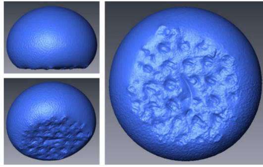
Figure 2-29 Left (top) – side view of the drop volume after thresholding and GDL subtraction. Left (bottom) tilted view of the same drop volume. Right – bottom view of the drop volume showing regularly spaced grooves, determined by the warp and weft surface of the GDL cloth
