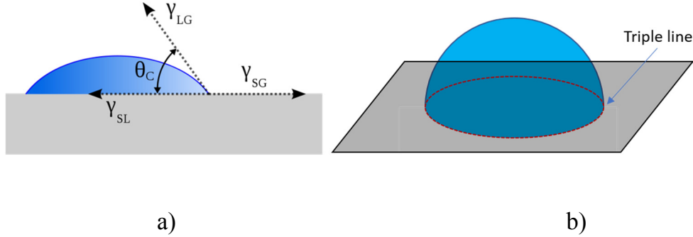
Figure 2-1 a) A diagram that shows the contact angle and interphase-energy between 3 phases (gas, liquid, solid). b) drop triple line highlighted in red. Images from a)[68] b) own.
