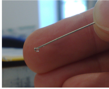
Figure 2-15 Picture of a small drop of Glycerol on top of the needle utilized to place it on the patterned surface.
