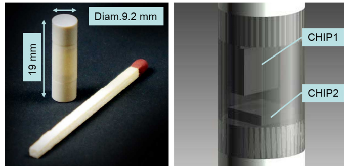
Figure 1-30 (Left) nano-bar phantom positioned near to a match for scale comparison. (right) enlarged view of the middle section of the phantom cylinder revealing the inside with the two chips positioned axially (chip1) and perpendicularly (chip2). Source: image courtesy of QRM GmbH (with own overlays)
