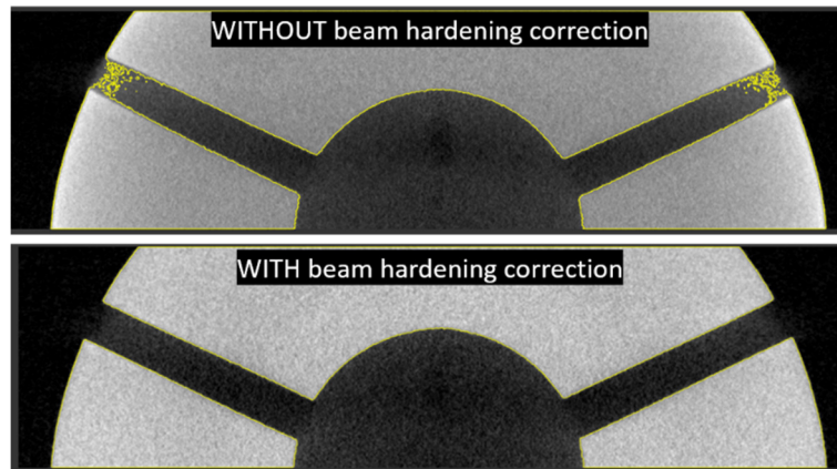
Figure 3-5 Top – thresholding of non-beam hardening corrected nozzle slice: yellow line represents the nozzle area recognized contour. The injection holes' exit is not reconstructed correctly since the pixel value in this position have a higher grayscale value which assigns them to the nozzle material instead that to air as supposed. Bottom – same slice with beam hardening correction; the brighter pixel values of the outer border have been corrected permitting detection of the hole geometry.
