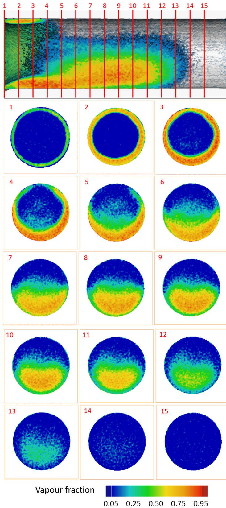
Figure 4-25 (1 of 2) Top: cross cut view of the MicroCT injection channel reconstructed volume presenting a red line every 600 \mu\text{m} . Following numbered images: sections perpendicular to the channel axis produced in the positions located by the previously mentioned red lines. All images refer to experiment no.2.
