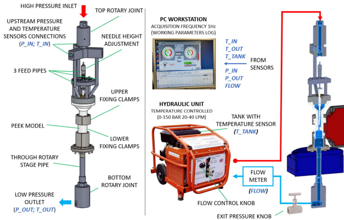
Figure 4-5 Left – microCT customized test rig parts description and localization. Right – Layout of the hydraulic circuit utilised to provide pressurized fluid for the experiment and to monitor interesting experimental conditions.
