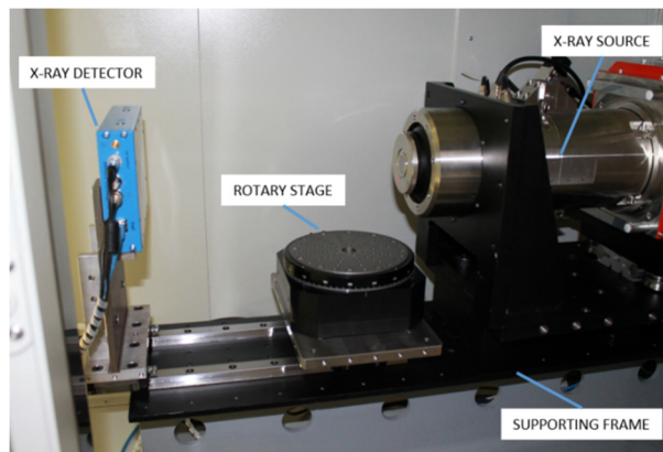
Figure 1-20 Close-up view of the inside of the cabinet with (from right to left) X-ray source, rotary stage and X-ray detector displayed.
