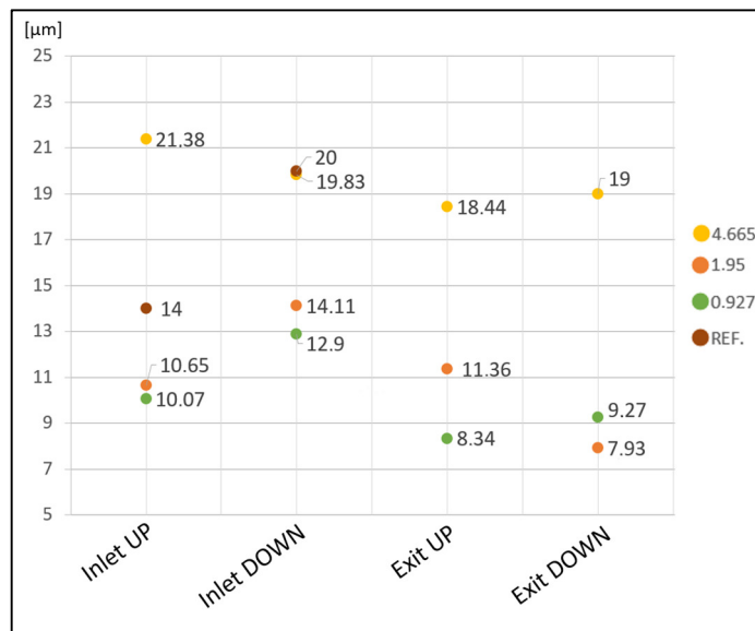
Figure 3-16 Plot of inlet/exit up/down rounding radii (mean values). Tomographic resolution of points is colour coded as per the legend presented in the right part of the image.
