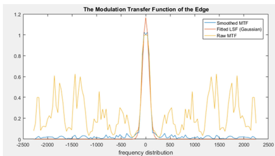
Figure 1-34 Plot of the Modulation Transfer Function (MTF) for the area selected on the reconstructed phantom slice.
