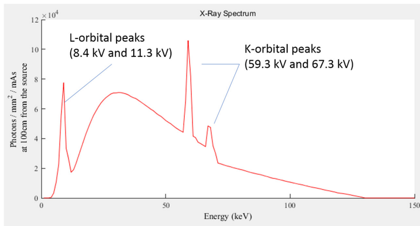
Figure 4-8 Plot of simulated Tungsten (W) target emission spectrum determined by an X-ray source voltage of 130 kV. Plot produced with software Spektr 3.0 [40]. Characteristic peaks are indicated by text and added blue lines.
