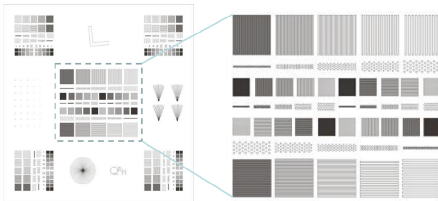
Figure 1-31 : (left) layout of the full engraved area of the two silicon chips contained in the phantom. (right) zoom of the central part of the engraved area showing line and point patterns with width from 10 to 1 \mu\text{m} . Source: image courtesy of QRM GmbH
