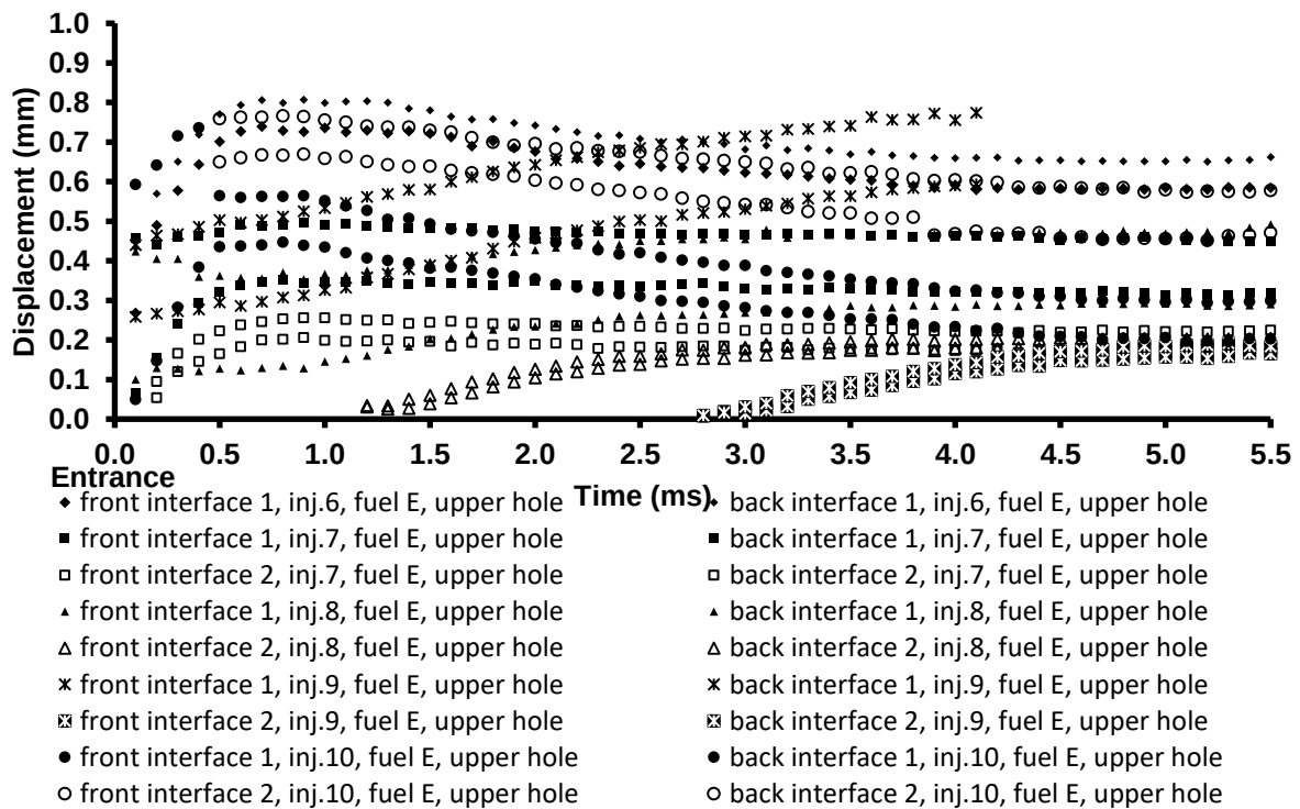
Figure A1.30: Displacement vs. time graph, fuel E, 350bar, inj. 6-10, upper hole.
