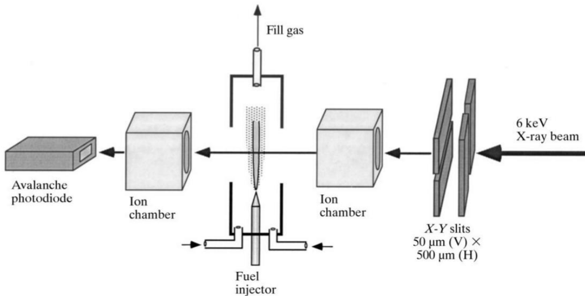
Figure 2.29: Schematic of X-ray absorption experimental setup 142 .
