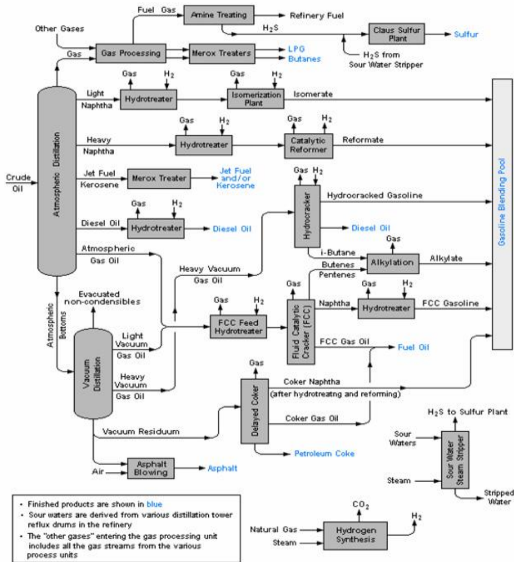
Figure 2.1: Basic schematic of a crude oil refinery system 18 .
