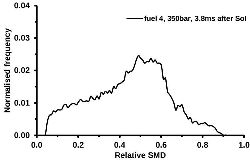
Figure 5.48: Relative SMD distribution produced by fuel 4 at 350bar (3.8ms after Sol).
