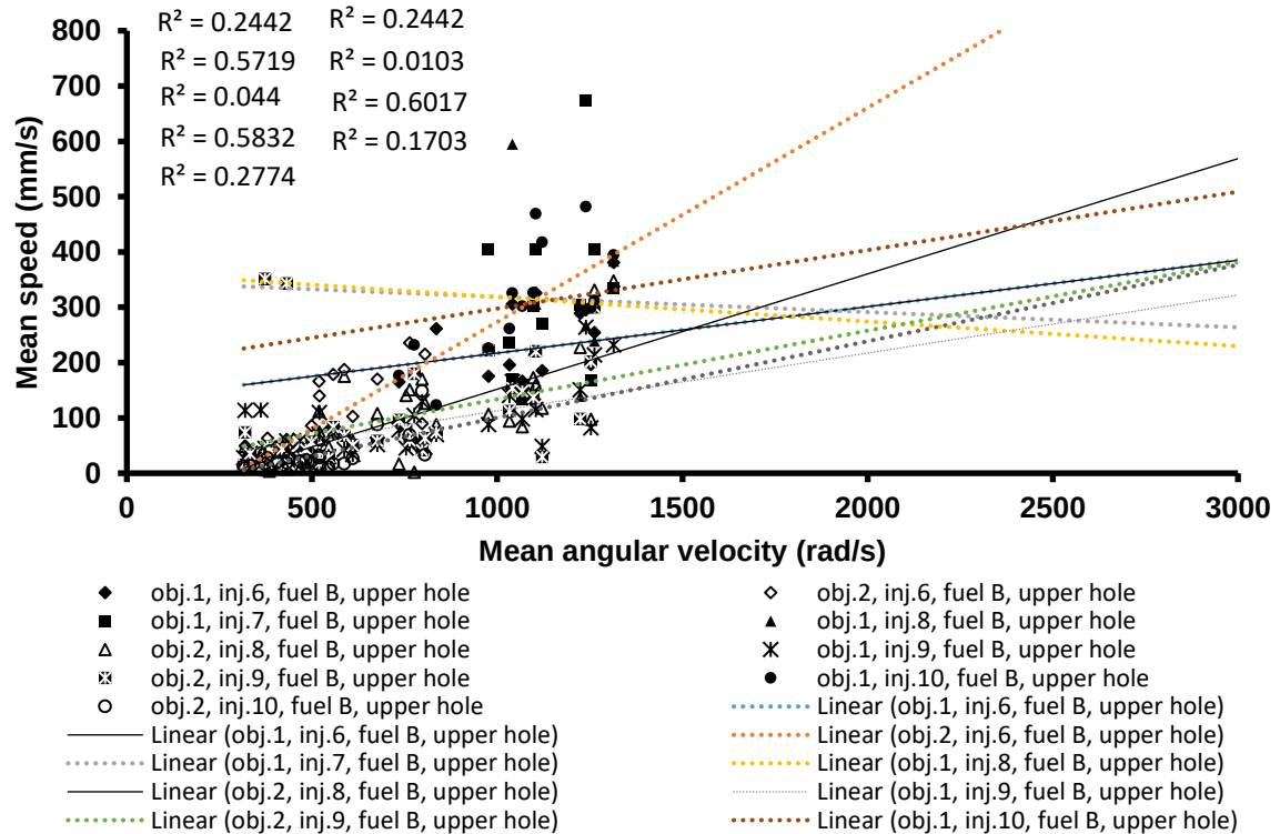
Figure A2.6: Mean speed vs. mean angular speed graph, fuel B, 350bar, inj.6-10, upper hole.
