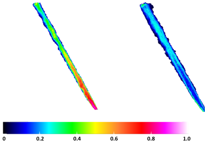
Figure 5.47: False coloured mean image (left) and STD image (right) produced by fuel 3 at 3.8ms after SolI and at 350bar.
