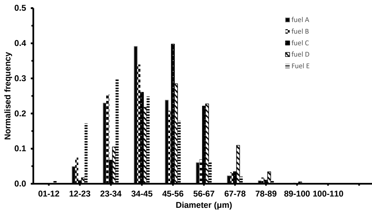
Figure 4.34: Normalised bubble size distribution for fuels A-E at 6.2ms after the needle return.
