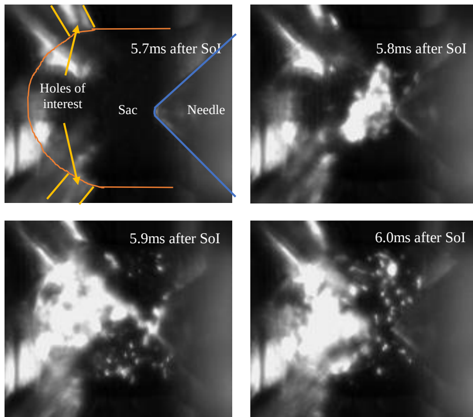
Figure 4.4: Images captured between 5.7ms and 6.0ms after the SoI showing the bubble formation in the sac due to needle sheet cavitation (fuel A, 350bar) 16 .
