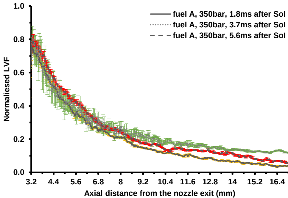
Figure 6.2: LVF distribution along the fuel A spray central axis produced at 350bar as a function of needle lift.
