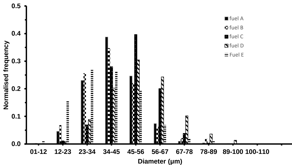
Figure 4.33: Normalised bubble size distribution for fuels A-E at 4.2ms after the needle return.
