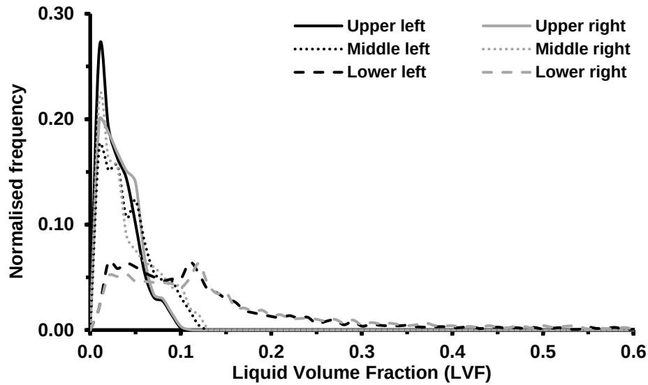
Figure 6.23: LVF distributions obtained from the upper, middle and lower segments of fuel 2 at 3.8ms after SoI, 350bar.
