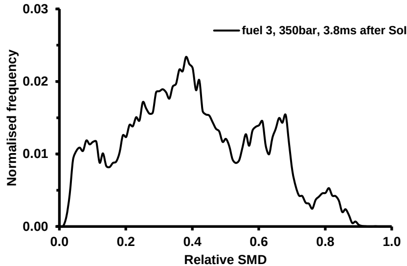
Figure 5.46: Relative SMD distribution produced by fuel 3 at 350bar (3.8ms after Sol).
