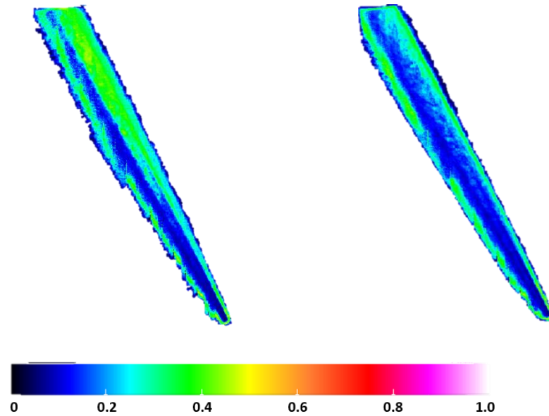
Figure 5.14: False coloured STD image produced at 3.7ms after SoI in case of 250bar (left hand side) and 350bar (right hand side) showing the variation of the relative SMD of the spray droplets.
