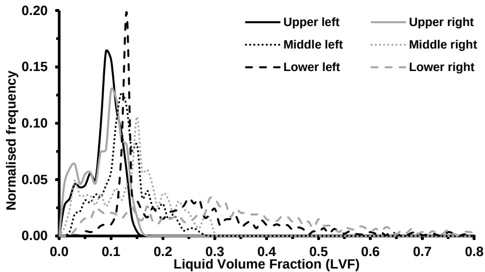
Figure 6.11: LVF distributions of the upper, middle and lower spray segments produced by fuel A at 250bar (3.7ms after SoI).
