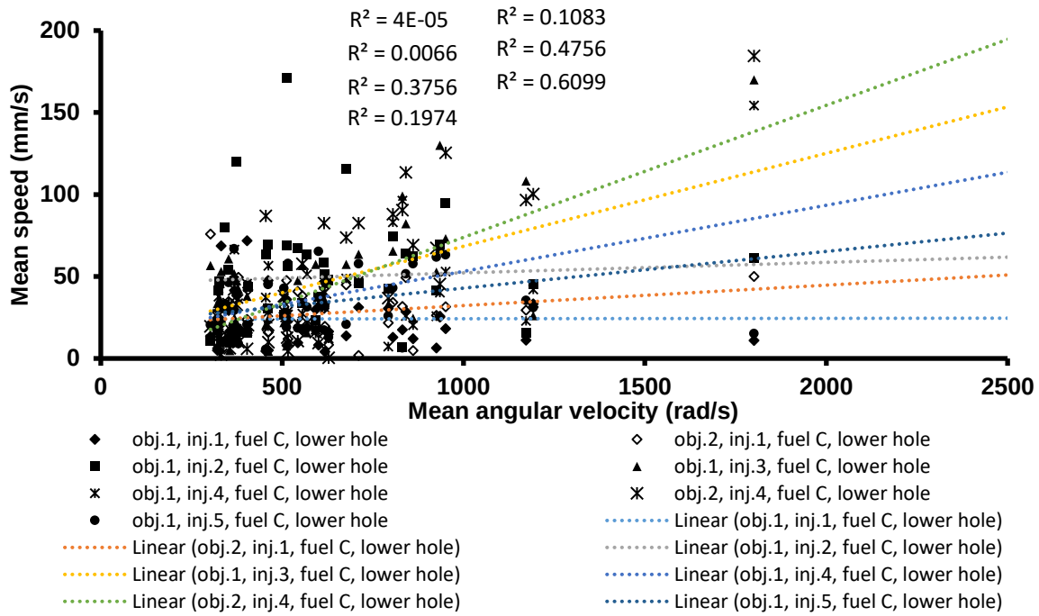
Figure A2.9: Mean speed vs. mean angular speed graph, fuel C, 350bar, inj.1-5, lower hole.
