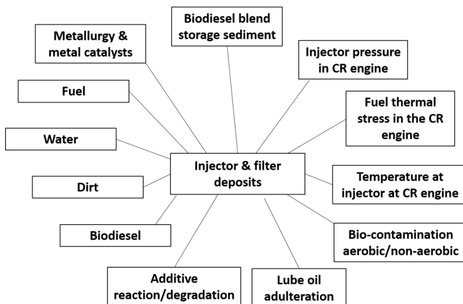
Figure 2.13: Possible causes of FIE deposits 79 .
