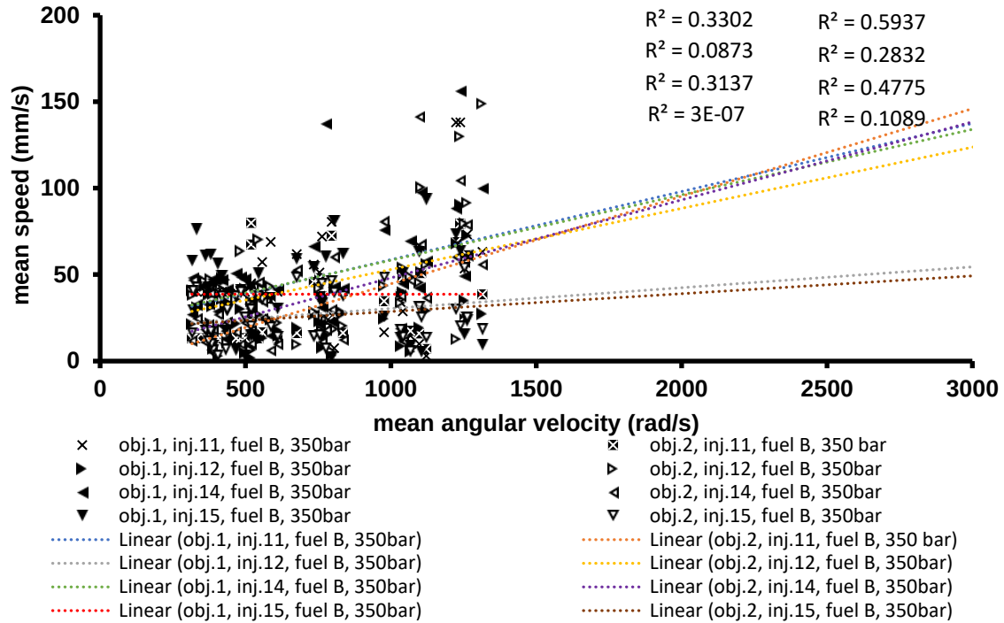
Figure A2.3: Mean speed vs. mean angular speed graph, fuel B, 350bar, inj.11-15, lower hole.
