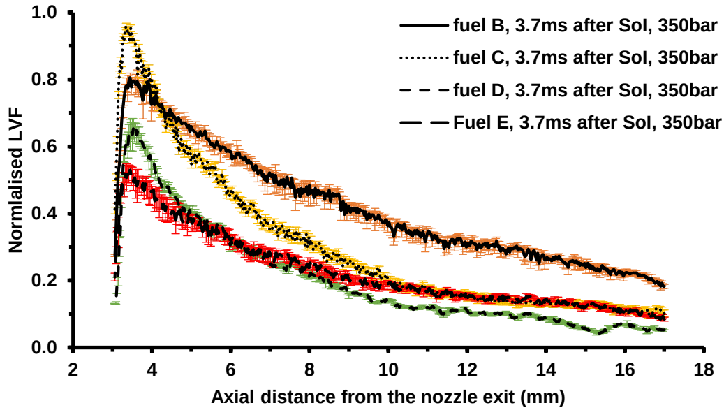
Figure 6.5: LVF distributions along the spray axis obtained from fuels B-E at 350bar (3.7ms after Sol).
