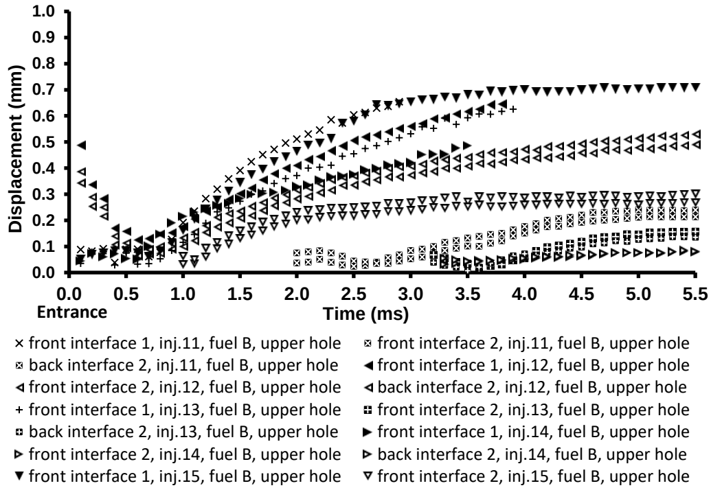
Figure A1.7: Displacement vs. time graph, fuel B,350 bar, inj.11-15, upper hole.
