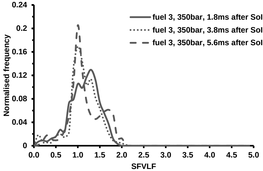
Figure 4.48: SFLVF distributions produced by the mean images obtained from fuel 3 at 350bar (1.8ms, 3.8ms and 5.6ms after Sol)
