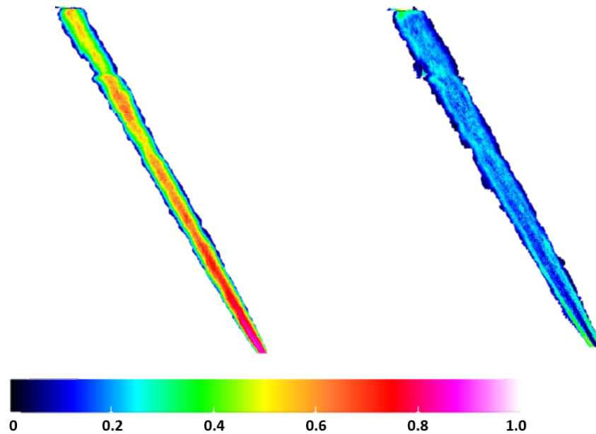
Figure 5.49: False coloured mean image (left) and STD image (right) produced at 3.8ms after Sol in case of fuel 4 at 350bar, showing the relative SMD distribution and variation along the spray.
