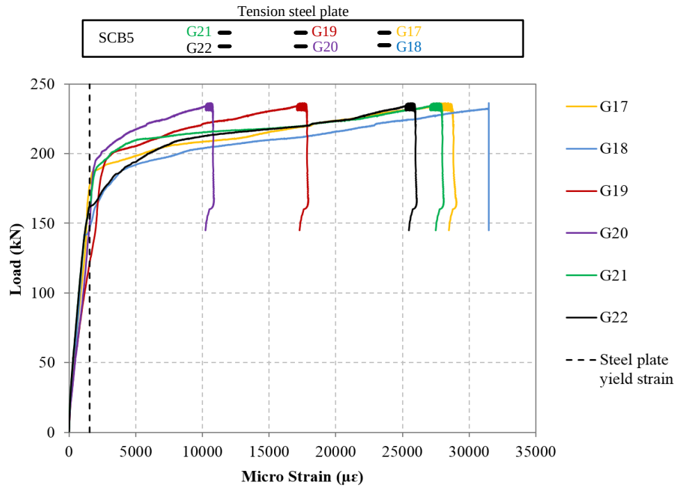
Figure 5.46. Measured strain in tension steel plate for SCB5
