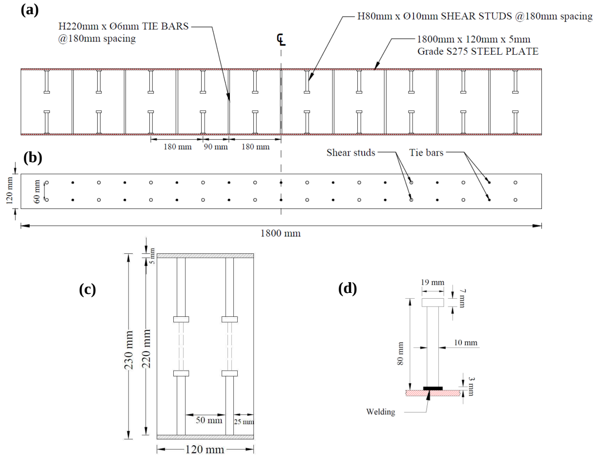
Figure 4.6. SC beam dimensions: (a) SC beam elevation; (b) shear stud and tie bar layout on both steel plates; (c) SC beam section; (d) shear stud details
