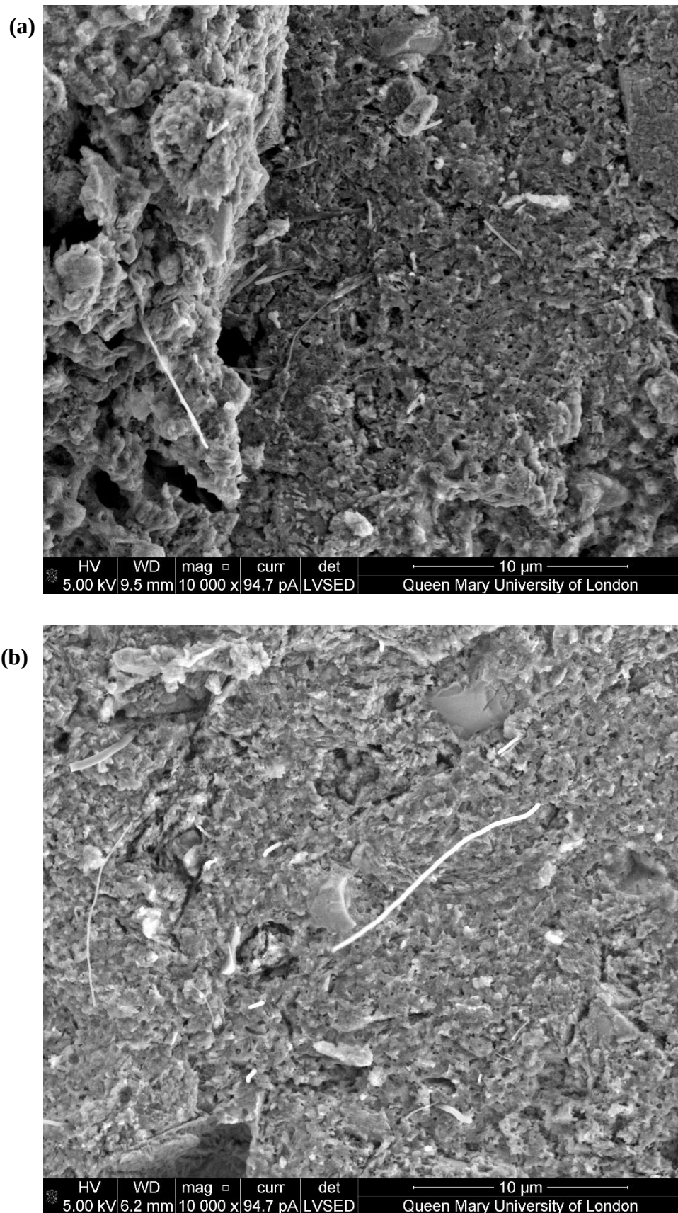
Figure 5.69. SEM micrographs of SCB5 core sample with 1.0% SF + 1.0% CNF at 10000× magnification
