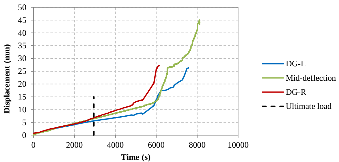
Figure 5.27. DG measurements for SCB3
