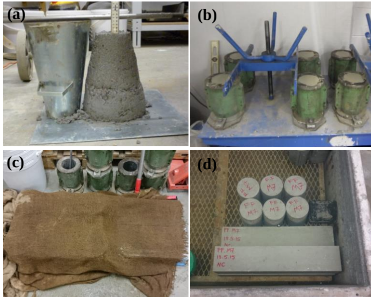
Figure 3.1. Sample preparation: (a) slump test; (b) vibration; (c) samples covered with wet cloth; (d) curing in water tank
