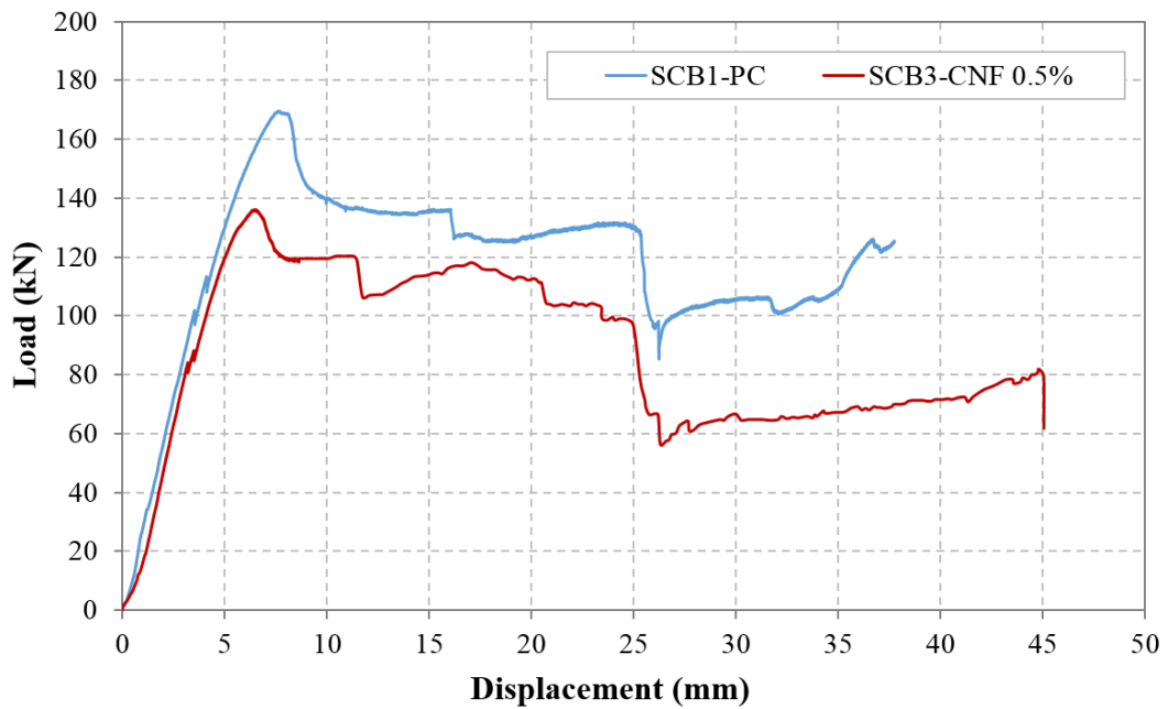
Figure 5.23. Load-displacement curve for SCB3
