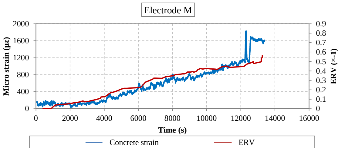
Figure 6.38. Electrode M results for SCB8
