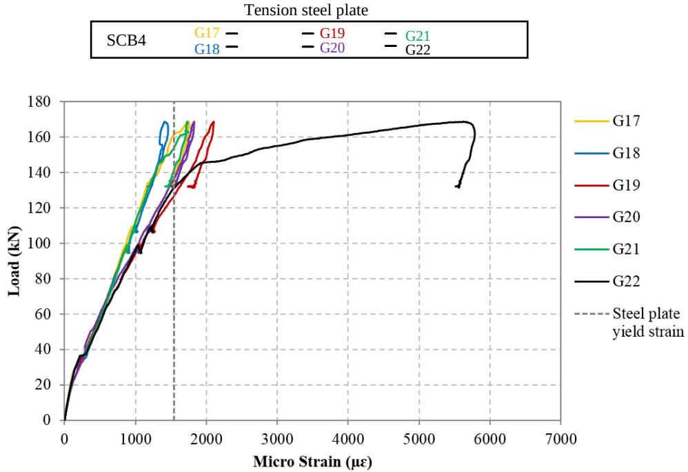
Figure 5.38. Measured strain in tension steel plate for SCB4
