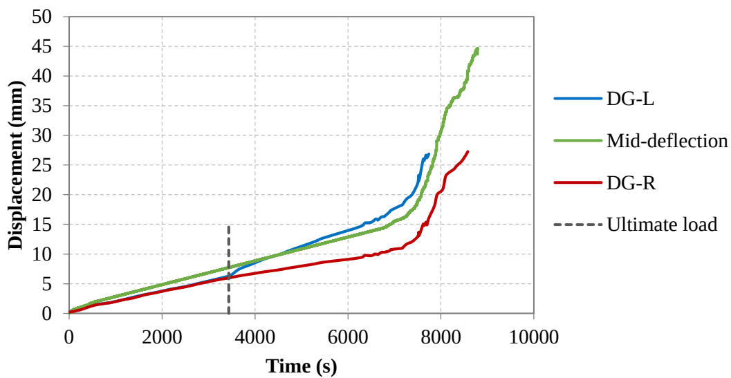
Figure 5.36. DG measurements for SCB4
