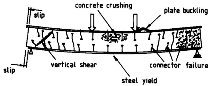
Figure 2.11. Failure modes of double skin composite beam (Wright et al., 1991b)
