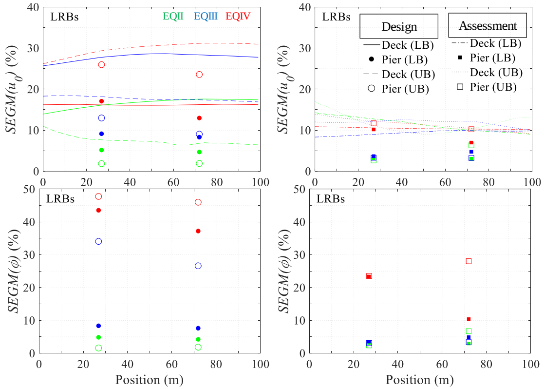
Fig. 5.10 SEGM (%) of peak relative (to the ground) deck and pier displacements u_0 , and curvatures \phi at the pier base derived from design (left) and assessment (right) stages in the case of the LRB scheme
