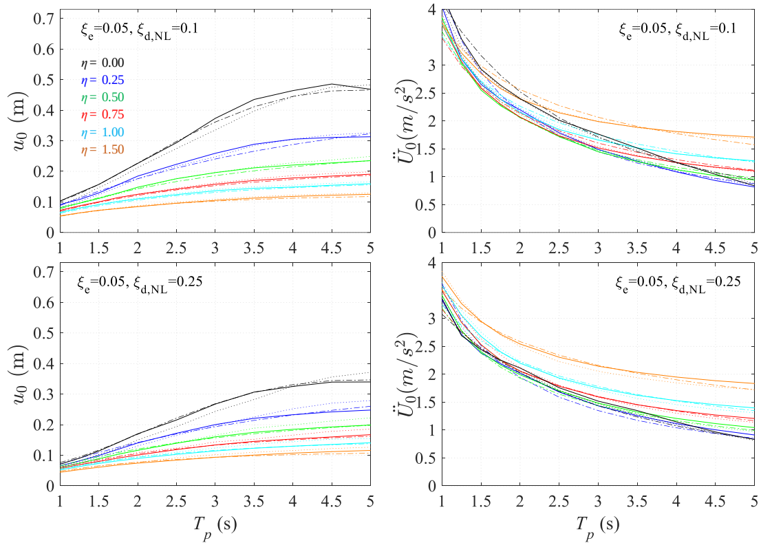
Fig. 4.26 NLRHA u_0 (left) and \ddot{U}_0 (right) under Art B considering energy-equivalent VDs of a=1 (solid), a=0.2 (dotted), compared to RM3 predicted response (dashed-dotted) for PGA=0.42g ( T_R \approx 2500 yrs, SF_{EQ}=2 )
