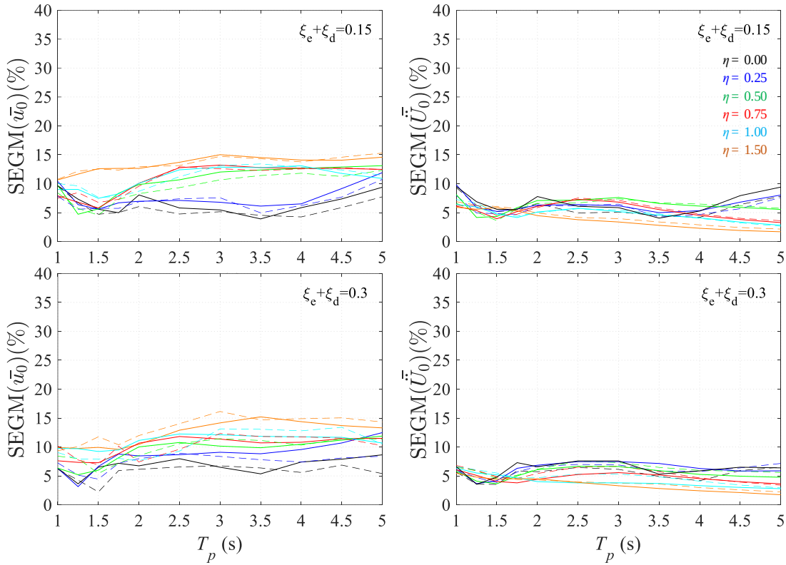
Fig. 4.21 NLRHA results under Art B suite: SEGM (%) of \bar{u}_0 (left) and \bar{U}_0 (right) considering energy-equivalent VDs of a=1 (solid) and a=0.2 (dashed) for PGA=0.42g ( T_R \approx 2500 yrs, SF_{EQ}=2 ), \zeta=15\% , 30\%
