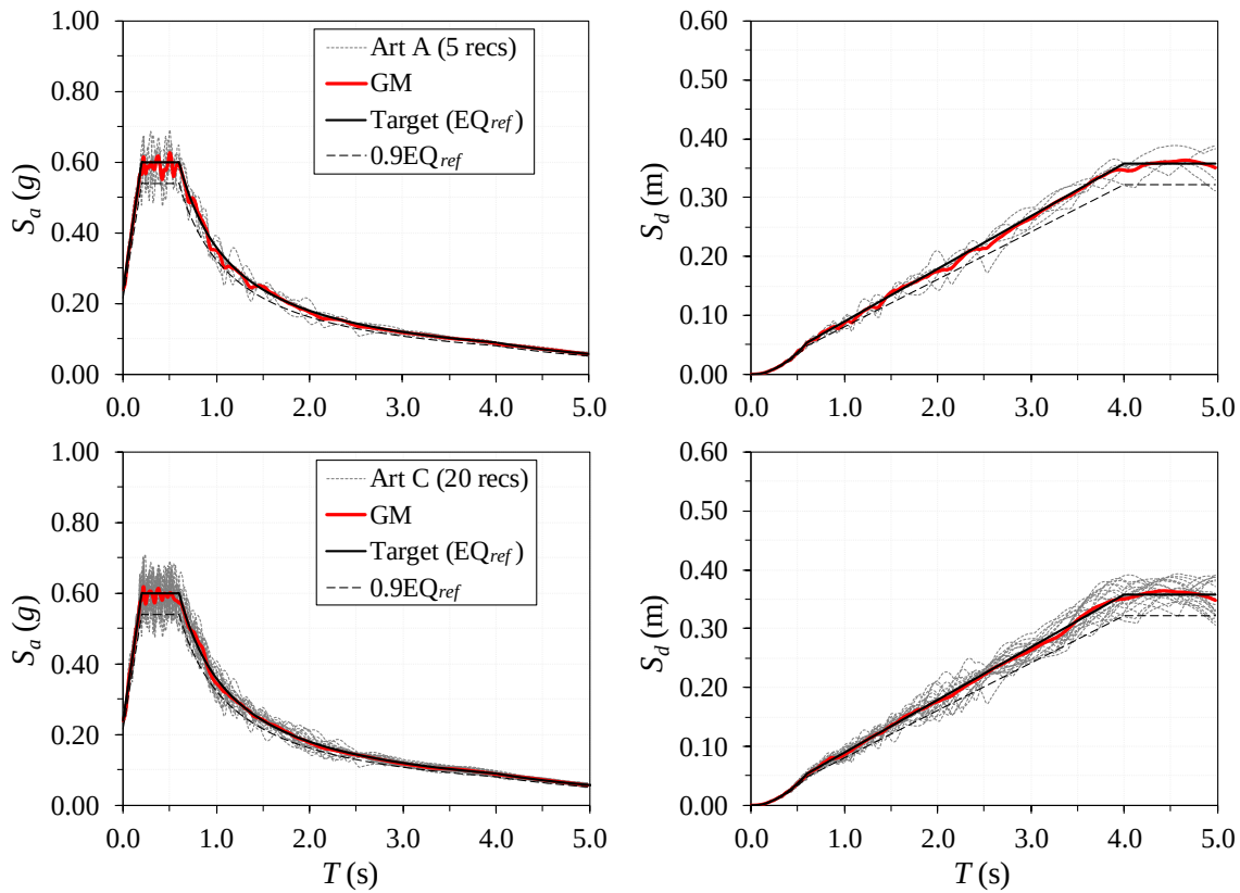
Fig. B.1 Spectral matching of response acceleration (left) and displacement (right) geometric mean (GM) spectra to the 1D target spectrum ( PGA of 0.21g , site 'C', T_{R,ref} ) for Art A, C) of artificial records
