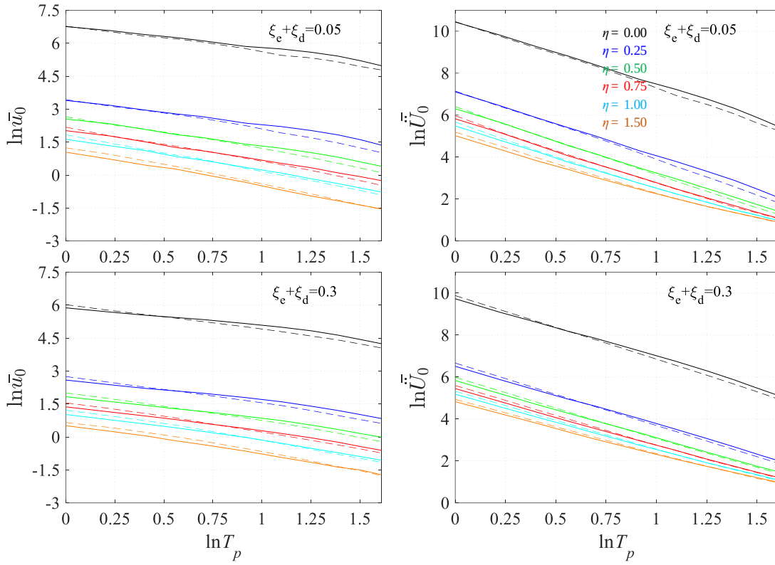
Fig. 4.29 NLRHA results under Art D (solid), Nat(SRSS) ( SF_{EC}=1 ) (dashed) suites: GM of \ln \bar{u}_0 (left) and \ln \bar{U}_0 (right) for PGA=0.42g ( T_R \approx 2500 yrs, SF_{EQ}=2 ), \zeta=5 , 30%, and \eta=0 \sim 1.5
