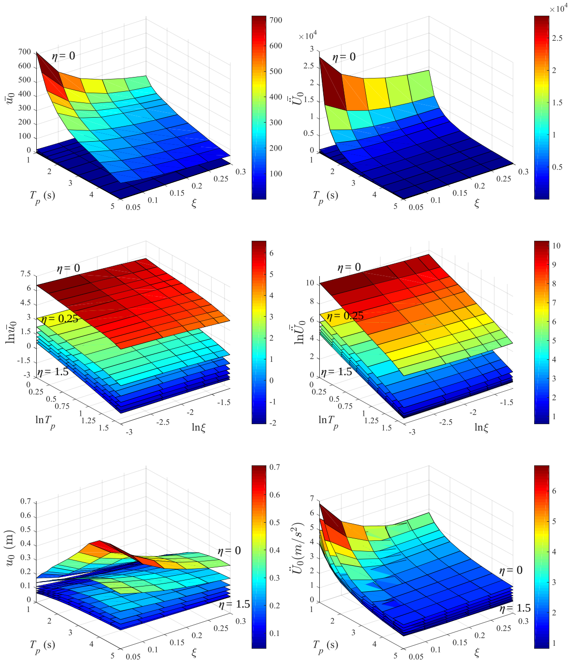
Fig. 4.10 NLRHA results under Art B suite: GM of peak normalised response ( \bar{u}_0 , \bar{U}_0 ), log-transformed peak normalised response ( \ln \bar{u}_0 , \ln \bar{U}_0 ), and non-normalised response ( u_0 , \ddot{U}_0 ) for PGA=0.42g ( T_R \approx 2500 yrs, SF_{EQ}=2 )
