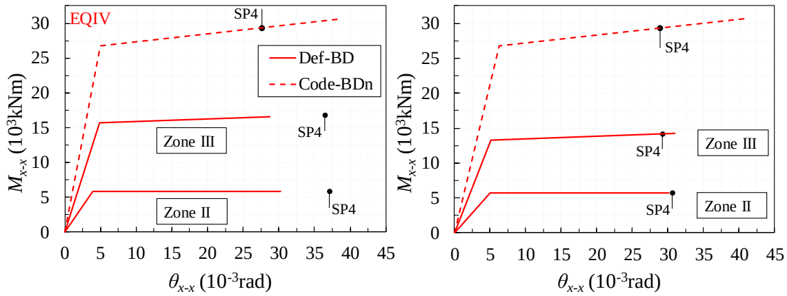
Fig. 6.5 Moment ( M_{x-x} ) vs. chord rotation ( \theta_{x-x} ) demand curves derived from assessment of Def-BD (ZII, ZIII), Code-BDn, under EQIV at the base of Pier 1 (left) and Pier 2 (right), compared with allowable SP4 deformation limits (solid dots)
