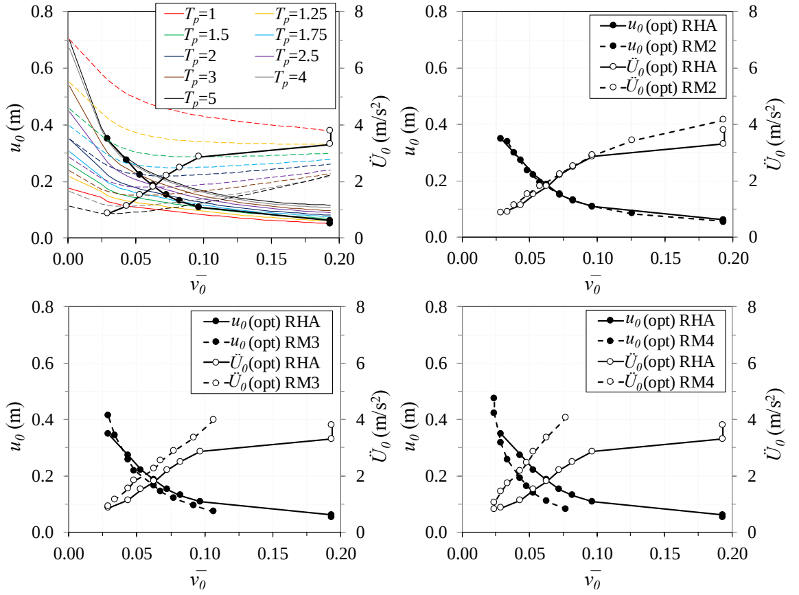
Fig. 4.20 NLRHA response u_0 (solid), \ddot{U}_0 (dashed), optimal peak total accelerations \ddot{U}_0^{\text{opt}} (solid) and corresponding relative displacements u_{\text{opt}} (solid) under Art B suite, compared to u_{\text{opt}} , \ddot{U}_0^{\text{opt}} (solid) derived from RM2, RM3, RM4 (dashed) for PGA=0.42g ( T_R \approx 2500\text{yrs} , SF_{EQ}=2 ), \zeta=5\% , 1D excitation
