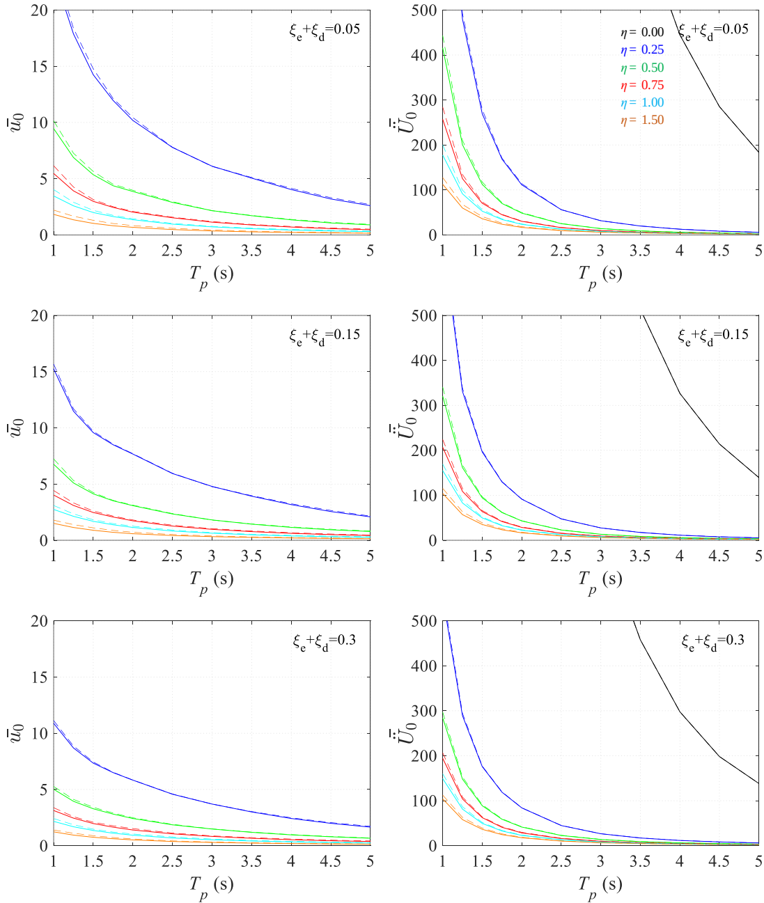
Fig. 4.12 NLRHA results under Art B suite: GM of \bar{u}_0 (left) and \bar{U}_0 (right) for PGA=0.21g ( T_R=475 yrs, SF_{EQ}=1 ) (dashed), PGA=0.42g ( T_R \approx 2500 yrs, SF_{EQ}=2 ) (solid), \xi=5, 15, 30\% , and \eta=0 \sim 1.5
