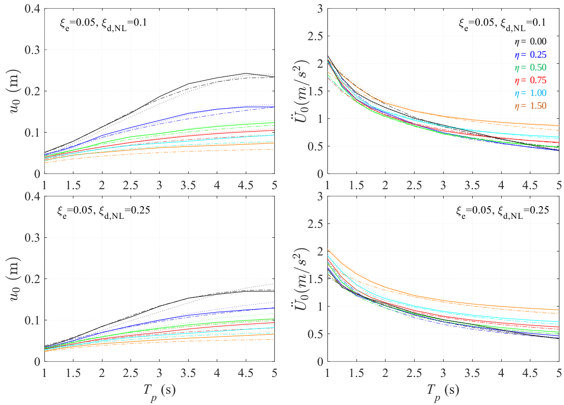
Fig. 4.25 NLRHA u_0 (left) and \ddot{U}_0 (right) under Art B considering energy-equivalent VDs of a=1 (solid), a=0.2 (dotted), compared to RM3 predicted response (dashed-dotted) for PGA=0.21g ( T_R=475 yrs, SF_{EQ}=1 )
