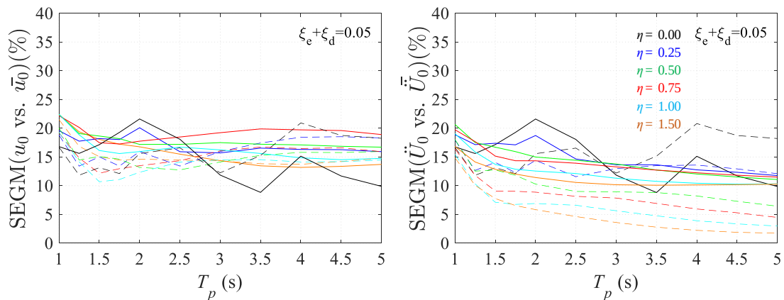
Fig. 4.17 NLRHA results under Nat(H1) ( SF_{EC}=1 ) suite: SEGM (%) of u_0, \ddot{U}_0 (solid) and \bar{u}_0, \bar{\ddot{U}}_0 (dashed) for PGA=0.42g ( T_R \approx 2500yrs , SF_{EQ}=2 ), \zeta=5\% , and \eta=0 \sim 1.5
