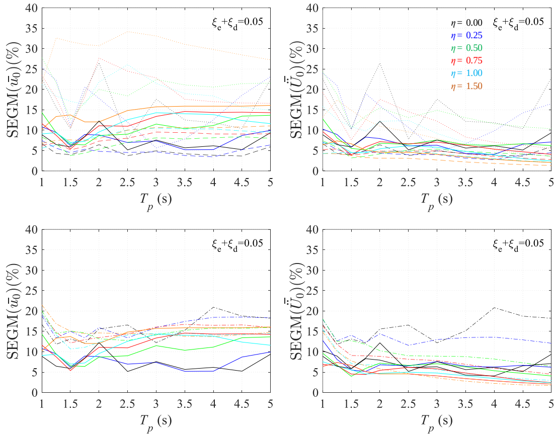
Fig. 4.16 NLRHA results under Art A (dotted), Art B (solid), Art C (dashed) (top), Art B (solid), Nat(H1) ( SF_{EC}=1 ) (dashed-dotted) (bottom) suites: SEGM of \bar{u}_0 (left) and \bar{\ddot{U}}_0 (right) for PGA=0.42g ( T_R \approx 2500yrs , SF_{EQ}=2 ), \zeta=5\% , and \eta=0 \sim 1.5
