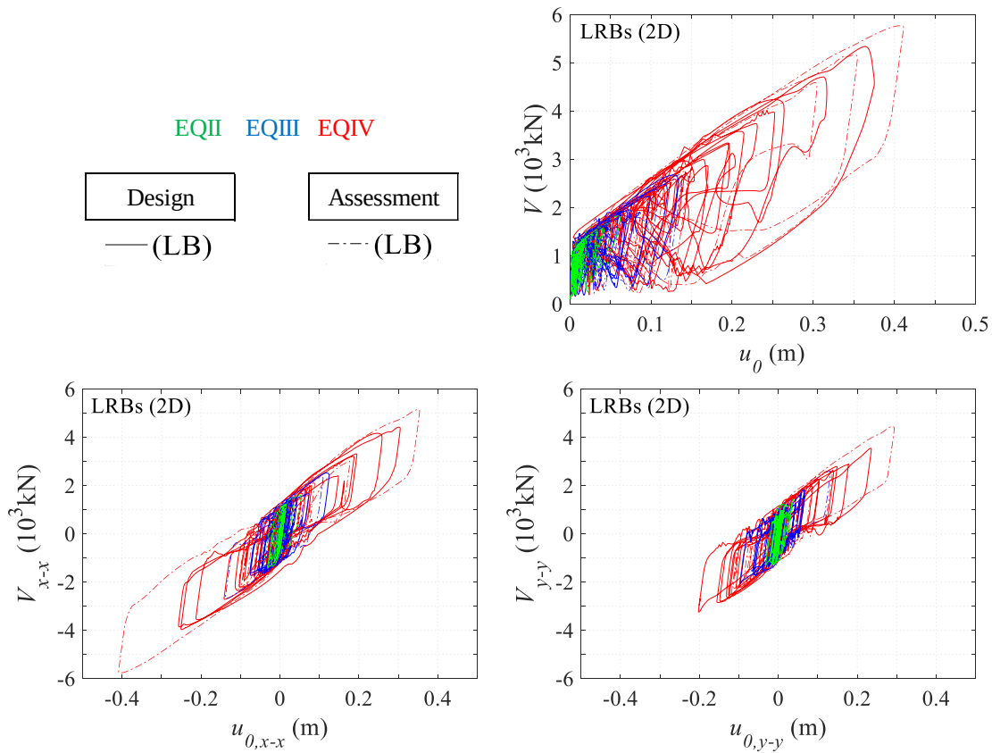
Fig. 5.18 Total shear force V vs. average relative displacement histories u_0 under RSN=776 (design), Art 1 (assessment), LB-DPs, and \theta_{EQ}=90^\circ
