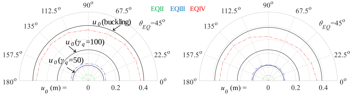
Fig. 6.13 GM of peak relative displacements u_0 of isolator located on top of Pier 1 (left) and Pier 2 (right) derived from assessment for \theta_{EQ}=0-180^\circ and LB-DPs, compared with SP requirements per PL
