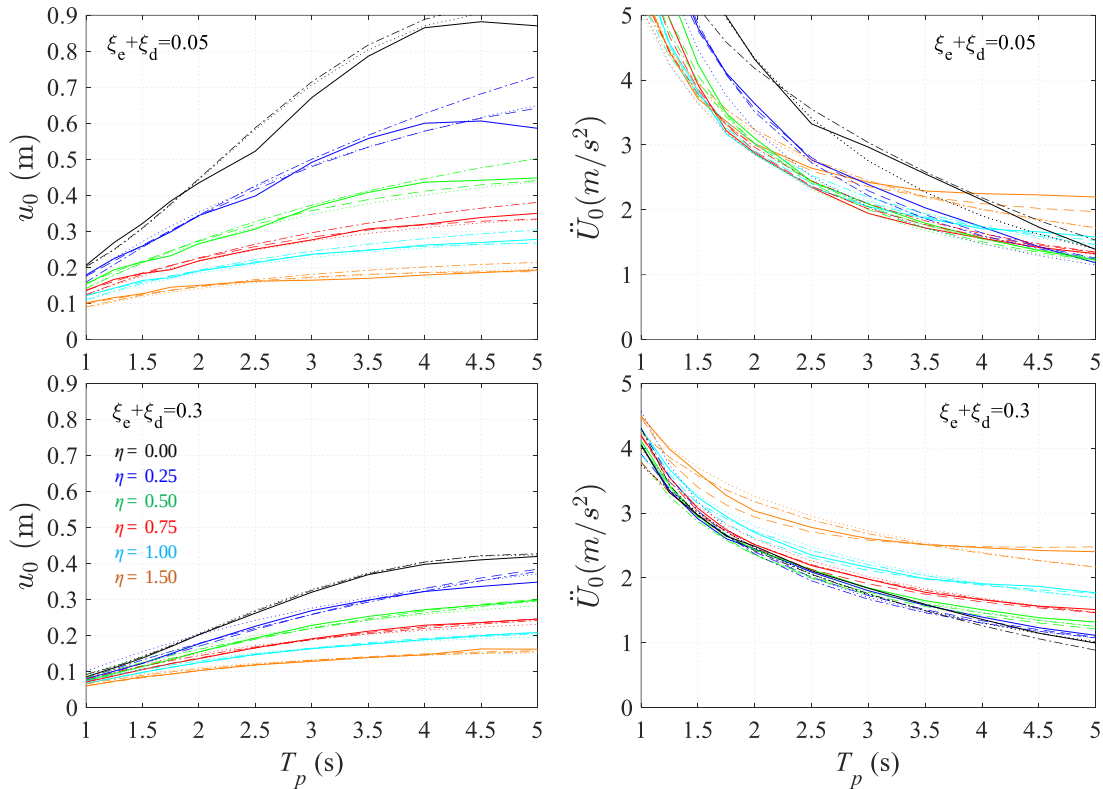
Fig. 4.34 NLRHA response u_0 (left) and \ddot{U}_0 (right) under Art D (solid) suite compared to response predicted from RM3 (dashed-dotted), and RM5 (dotted) for PGA=0.42g ( T_R=2500\text{yrs} , SF_{EQ}=2 ), \xi=5 , 30%
