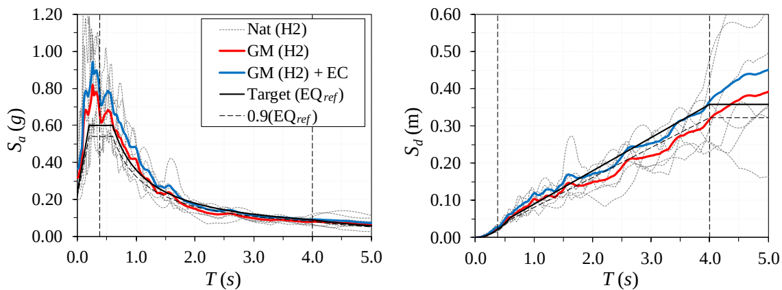
Fig. 5.6 Spectral matching of response acceleration (left) and displacement (right) geometric mean (GM) and EN1998-2-scaled geometric mean (GM+EC) ( SF_{EC}=1.15 ) spectra to the 1D target spectrum ( PGA of 0.21g, site ‘C’, T_{R,EQIII} ) for the adopted suite of SF_{MSE} -scaled natural (Nat) records considering H2 components
