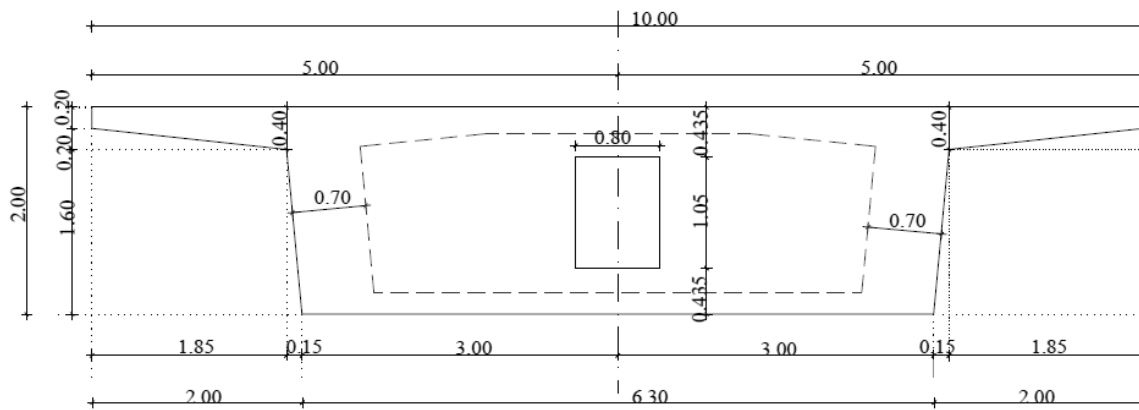
Section 1-1 in Fig. 3.6
