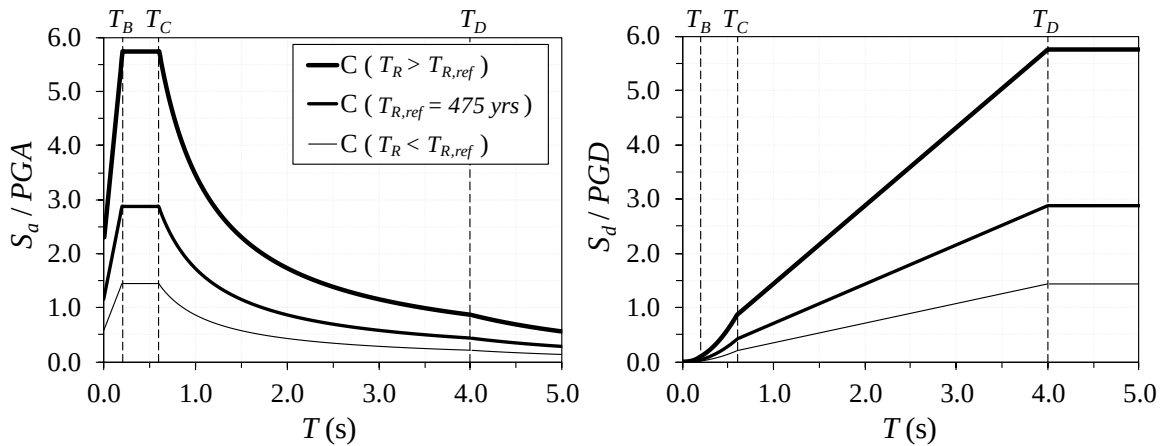
Fig. 3.9 1D target design horizontal acceleration S_a/PGA (left) and displacement S_d/PGD (right) response spectra for site conditions ‘C’ and different return periods T_R
