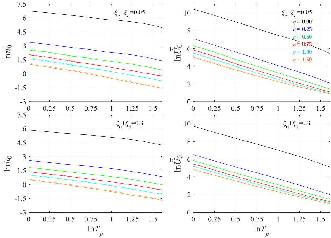
Fig. 4.28 NLRHA results under Art D suite: GM of \ln \bar{u}_0 (left) and \ln \ddot{U}_0 (right) for PGA=0.21g ( T_R=475 yrs, SF_{EQ}=1 ) (dashed), PGA=0.42g ( T_R \approx 2500 yrs, SF_{EQ}=2 ) (solid), \xi=5, 30\% , and \eta=0 \sim 1.5
