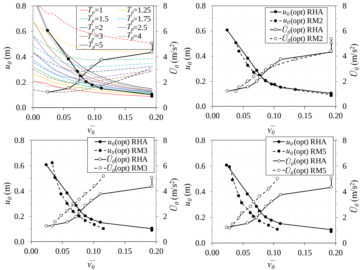
Fig. 4.35 NLRHA response u_0 (solid), \ddot{U}_0 (dashed), optimal peak total accelerations \ddot{U}_0^{\text{opt}} (solid) and corresponding relative displacements u_{\text{opt}} (solid) under Art D suite, compared to u_{\text{opt}} , \ddot{U}_0^{\text{opt}} (solid) derived from RM2, RM3, RM5 (dashed) for PGA=0.42g ( T_R \approx 2500\text{yrs} , SF_{EQ}=2 ), \zeta=5\% , 2D excitation
