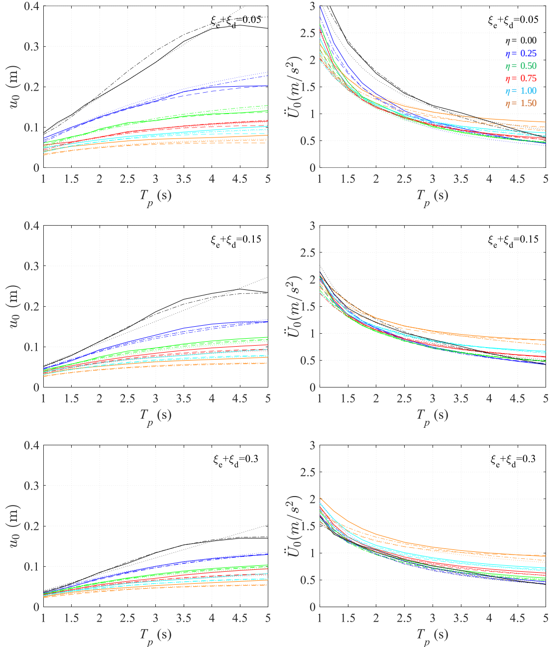
Fig. 4.18 NLRHA u_0 (left) and \ddot{U}_0 (right) under Art B (solid) compared to response predicted from RM2 (dashed), RM3 (dashed-dotted), and RM4 (dotted) for PGA=0.21g ( T_R=475\text{yrs} , SF_{EQ}=1 ), \xi=5, 15, 30\% , \eta=0\sim 1.5
