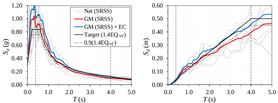
Fig. 5.7 Spectral matching of response acceleration (left) and displacement (right) geometric mean (GM) and EN1998-2-scaled geometric mean (GM+EC) ( SF_{EC}=1.15 ) SRSS spectra to the 2D target spectrum ( PGA_{2D} of 0.30g, site 'C', T_{R,EQIII} ) for the adopted suite of rotated and SF_{MSE} -scaled natural (Nat) records
