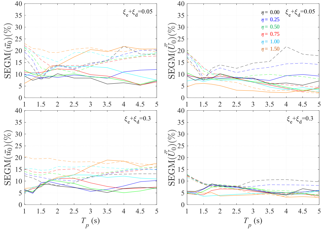
Fig. 4.27 NLRHA results under Art D (solid), Nat(SRSS) ( SF_{EC}=1 ) (dashed) suites: SEGM of \bar{u}_0 (left) and \ddot{U}_0 (right) for PGA=0.42g ( T_R \approx 2500 yrs, SF_{EQ}=2 ), \xi=5, 30\% , and \eta=0 \sim 1.5
