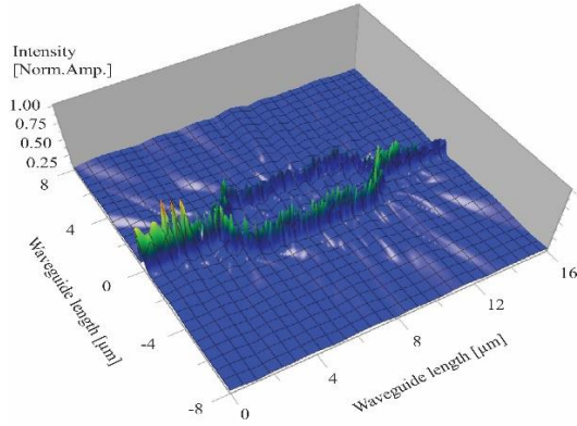
Figure 2: The 3D image obtained using the Optiwave program, where all parameters are given in Figure 1. The input source wavelength is 1.55 \text{ } \mu\text{m} .
